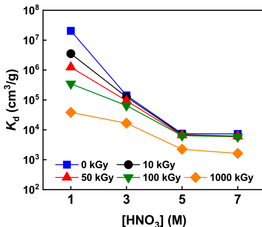
Figure 4. K_d of \text{KAlFe}(\text{CN})_6/\text{SiO}_2 for \text{Pd}(\text{II}) before and after irradiation in 1–7 M \text{HNO}_3 ; phase ratio = 100 \text{ cm}^3 \text{g}^{-1} , [\text{Pd}] = 200 \text{ mg L}^{-1} , temperature = 25^\circ \text{C} , and contact time = 24 h.
