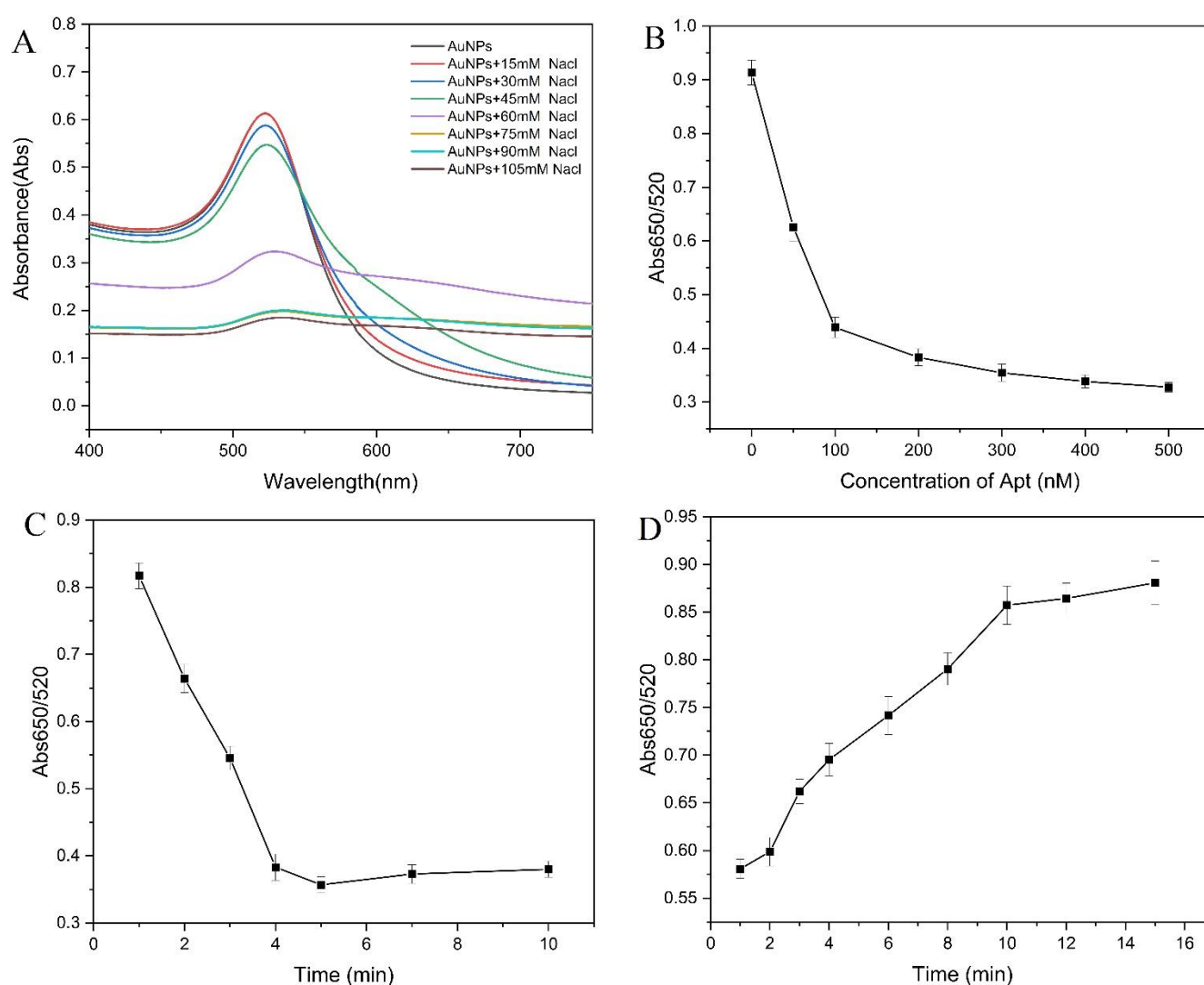
Figure 5. Optimization of the aptamer-AuNPs colorimetric conditions. (A) NaCl concentration. (B) Aptamer concentration. (C) Reaction time between AuNPs and NaCl. (D) Incubation time of aptamer and AuNPs.
