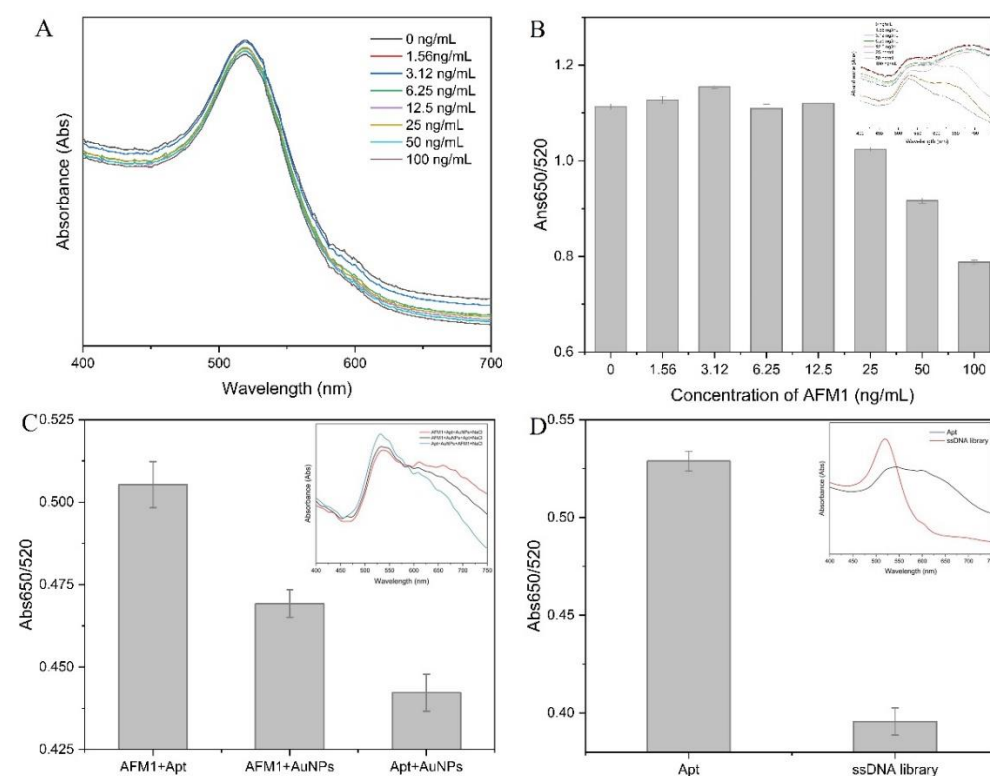
Figure 4. UV-vis spectra of AuNPs in the absence (A) and presence (B) of NaCl in the presence of different concentrations of AFM1. (C) The effect of AFM1, aptamer, and AuNPs reaction sequence. (D) Comparison of binding ability of aptamer and ssDNA library.
