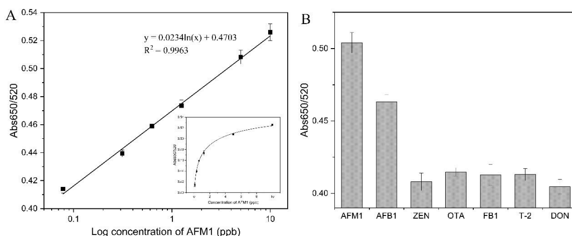
Figure 6. (A) Standard curve of the aptamer-AuNPs colorimetric method for detection of AFM1. (B) Specificity of aptamer-AuNPs colorimetric method for detection of AFM1.
