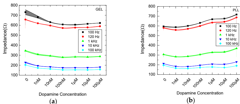
Figure 3. Comparison of mean impedance magnitude values for cells in 3D (GEL) (a) and 2D (PLL) (b) cultures treated with DA at five different frequencies (100Hz/ 120Hz/ 1KHz/ 10KHz/ 100KHz), with \pm SD values.
