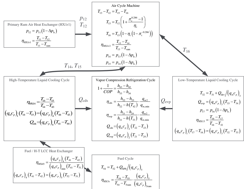
Figure 3. Structure of parameter matching algorithm of integrated thermal management system.
