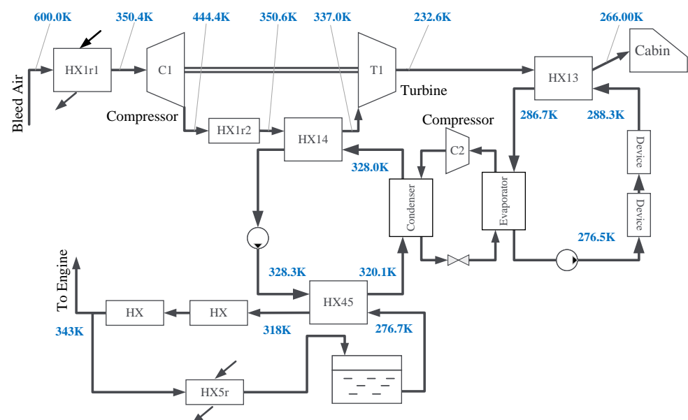
Figure 5. Temperature results under ground conditions.
