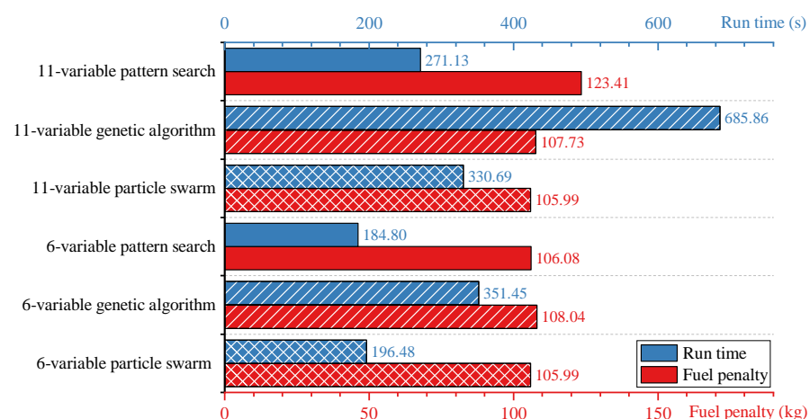
Figure 9. Comparison of optimization results and run times.
