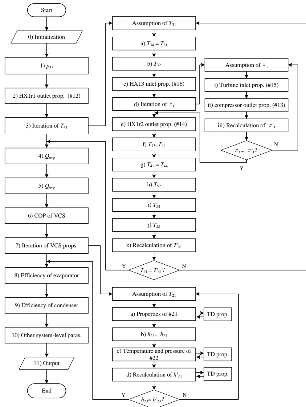
Figure 4. Flow chart of parameter matching of integrated thermal management system.
