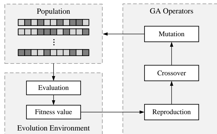
Figure 8. Flow diagram of the genetic algorithm.
