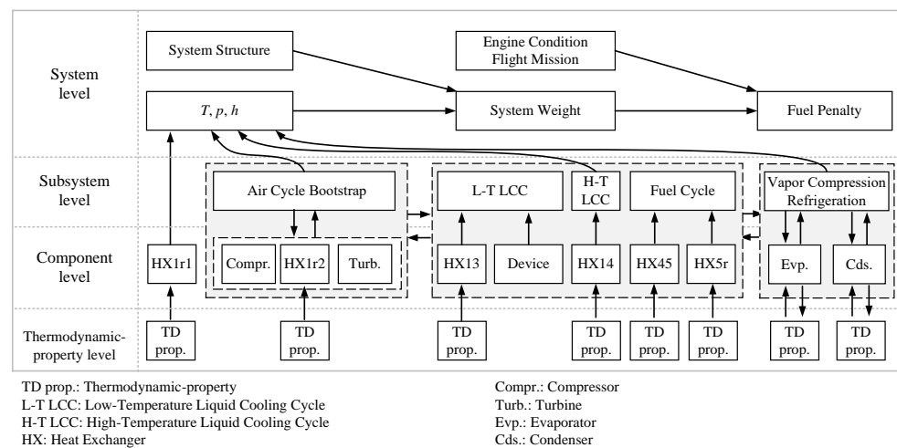
Figure 2. Levels of parameter matching of integrated thermal management system.
