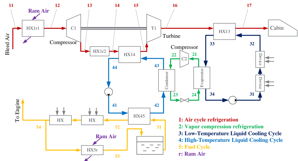
Figure 1. Structure of the integrated thermal management system.
