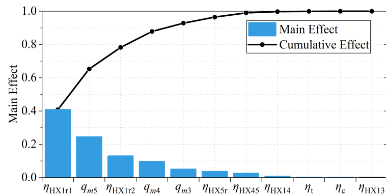
Figure 7. Analysis of variance of main influencing factors on fuel consumption.
