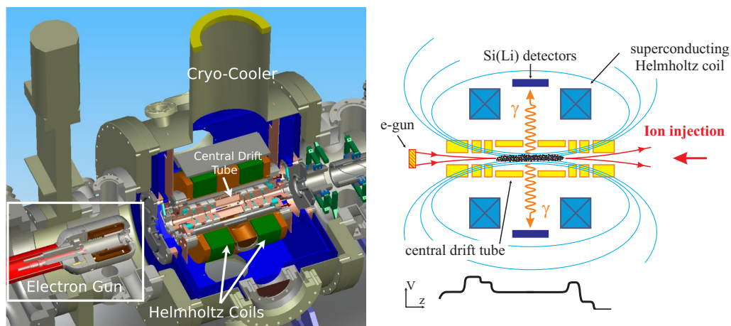
Figure 2. (left) a schematic view of the trap and electron-gun portions of the TITAN EBIT; (right) an illustration of the EBIT operation for decay spectroscopy and charge breeding (not to scale). Depicted below the trap components is a typical potential profile of the trap electrodes while the ion bunch is confined in the EBIT.
