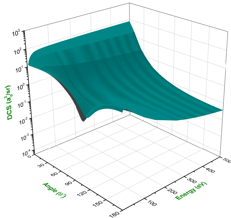
Figure 11. Variation of the DCS ( a_0^2/sr ) for the elastic scattering of electrons from carbon dioxide.
