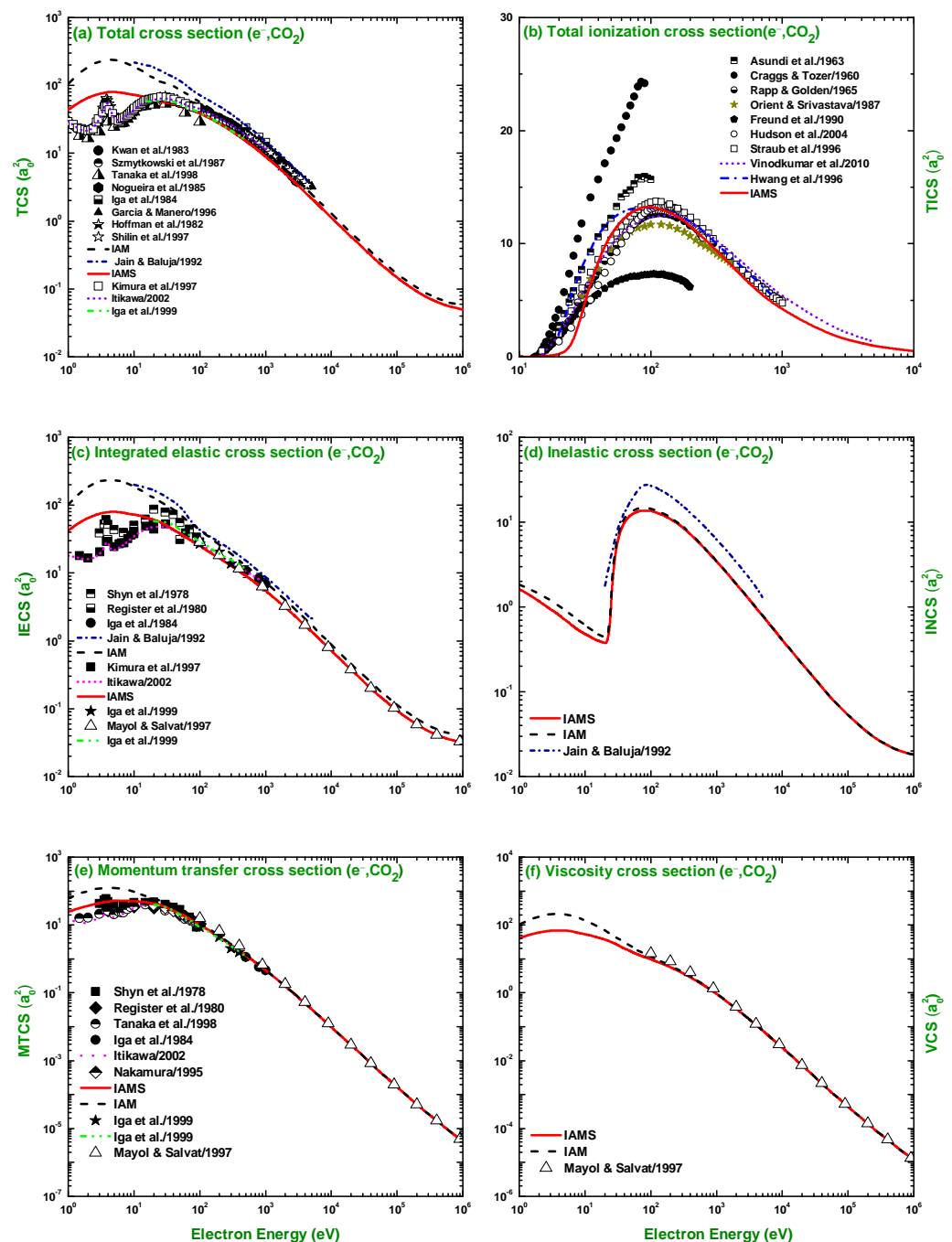
Figure 16. Values ( a_0^2 ) of TCS, TICS, IECS, INCS, MTCS, and VCS for the scattering of electrons from carbon dioxide. Theoretical: IAM, IAMS, Vinodkumar et al. [21], Iga et al. [45], Jain and Baluja [63], Hwang et al. [64], and Mayol and Salvat [71]. Recommended: Itikawa [14]. Experimental: Hudson et al. [20], Iga et al. [45], Tanaka et al. [46], Shyn et al. [47], Register et al. [48], Iga et al. [52], Kwan et al. [57], Szmytkowski et al. [58], Nogueira et al. [59], Garcia and Manero [60], Hoffman et al. [61], Shilin et al. [62], Asundi et al. [65], Craggs and Tozer [66], Rapp and Golden [67], Orient and Srivastava [68], Freund et al. [69], Straub et al. [70], Kimura et al. [72] and Nakamura [73].
