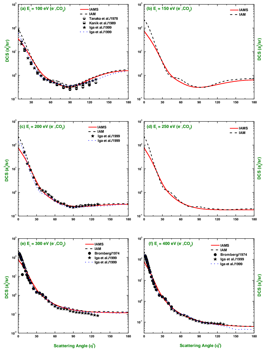
Figure 2. DCS ( a_0^2/\text{sr} ) for the elastic scattering of electrons from carbon dioxide at energies of 100, 150, 200, 250, 300, and 400 eV. Theoretical: References in Figure 1. Experimental: References in Figure 1, Iga et al. [45], and Bromberg [50].
