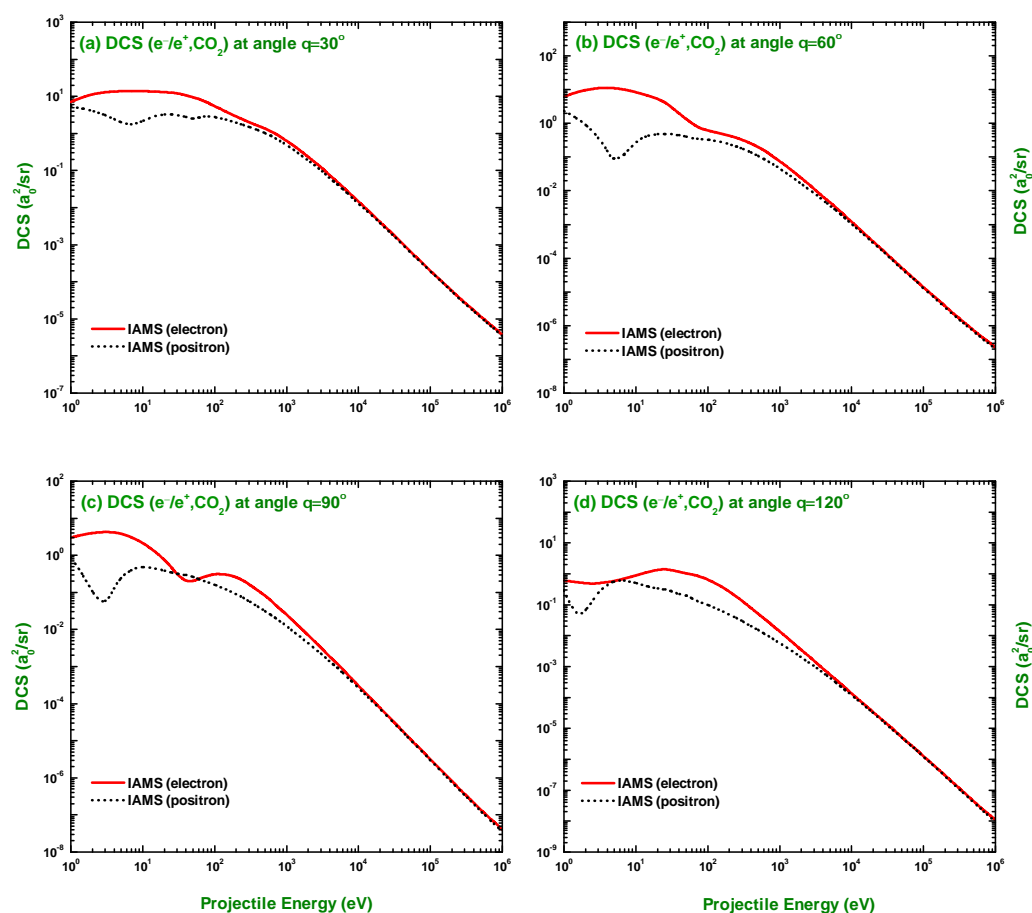
Figure 10. Comparison of the DCSs ( a_0^2/\text{sr} ) for the elastic scattering of electrons and positrons from carbon dioxide at angles of 30^\circ , 60^\circ , 90^\circ , and 120^\circ .
