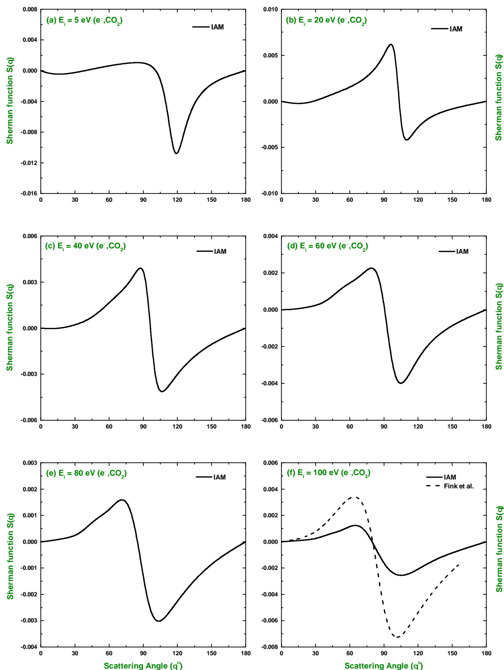
Figure 13. Angular dependence of the spin polarization of scattered electrons. Theoretical: IAM, Fink and Yates [55], and Fink and Ingram [56].
