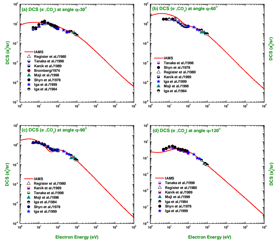
Figure 8. Energy dependence of the DCS ( a_0^2/\text{sr} ) for the elastic scattering of electrons from carbon dioxide at angles of 30^\circ , 60^\circ , 90^\circ , and 120^\circ . References: available in Figures 1–4.
