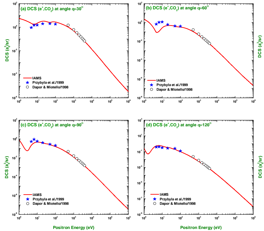
Figure 9. Energy dependence of the DCS ( a_0^2/\text{sr} ) for the elastic scattering of positrons from carbon dioxide at angles of 30^\circ , 60^\circ , 90^\circ , and 120^\circ . References: available in Figures 5–7.
