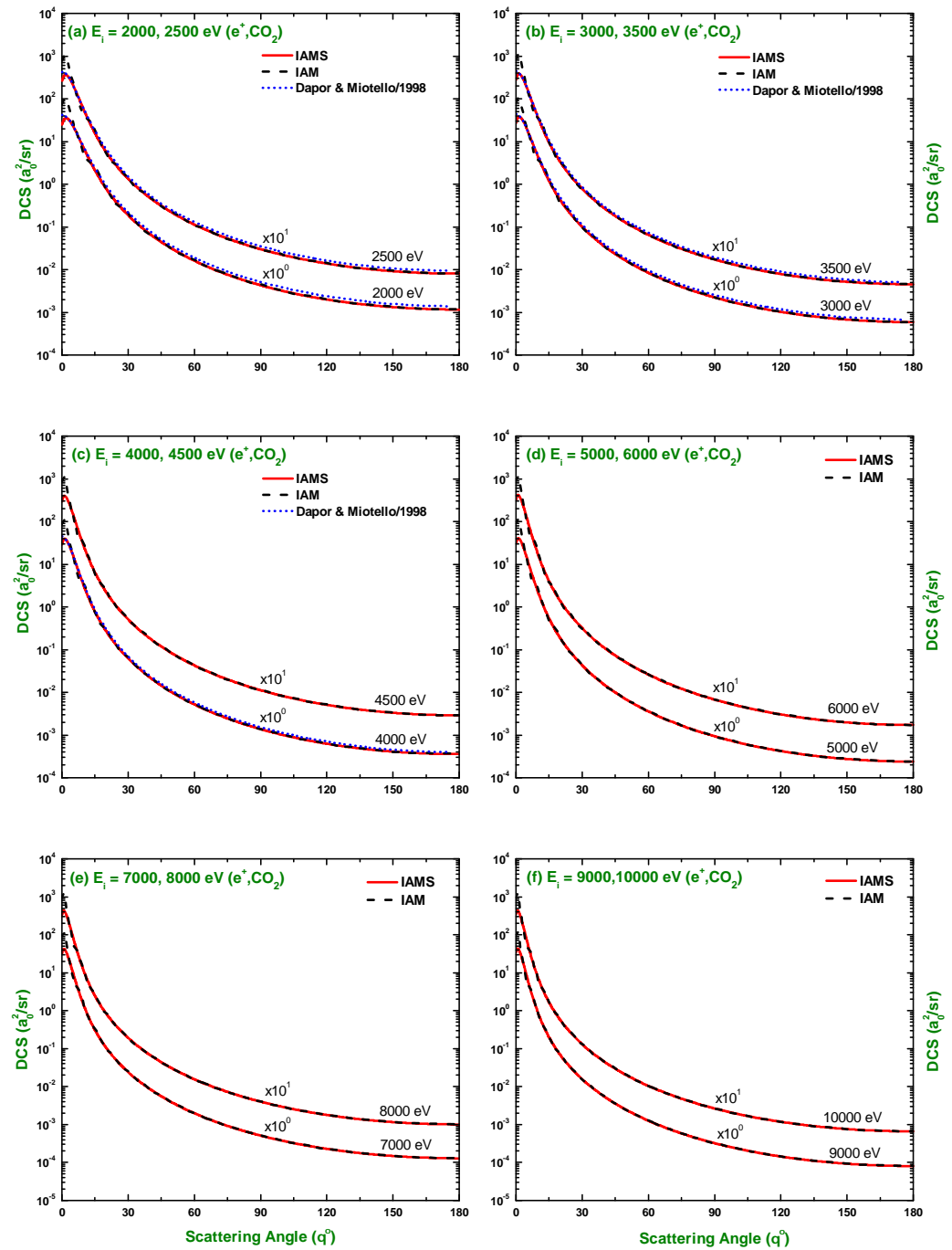
Figure 7. DCS ( a_0^2/\text{sr} ) for the elastic scattering of positrons from carbon dioxide at energies of 2000, 2500, 3000, 3500, 4000, 4500, 5000, 6000, 7000, 8000, 9000, and 10,000 eV. References in Figure 6.
