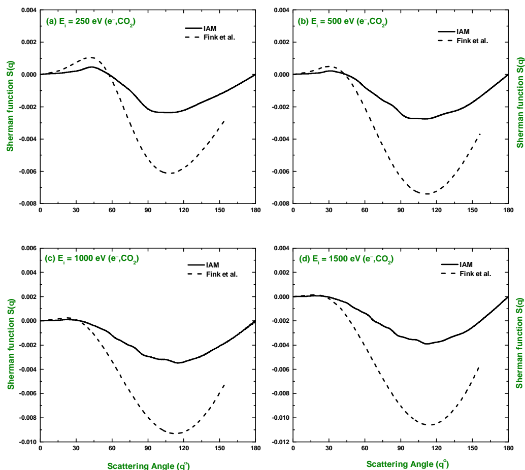
Figure 14. Angular dependence of the spin polarization of scattered electrons. References: available in Figure 13.
