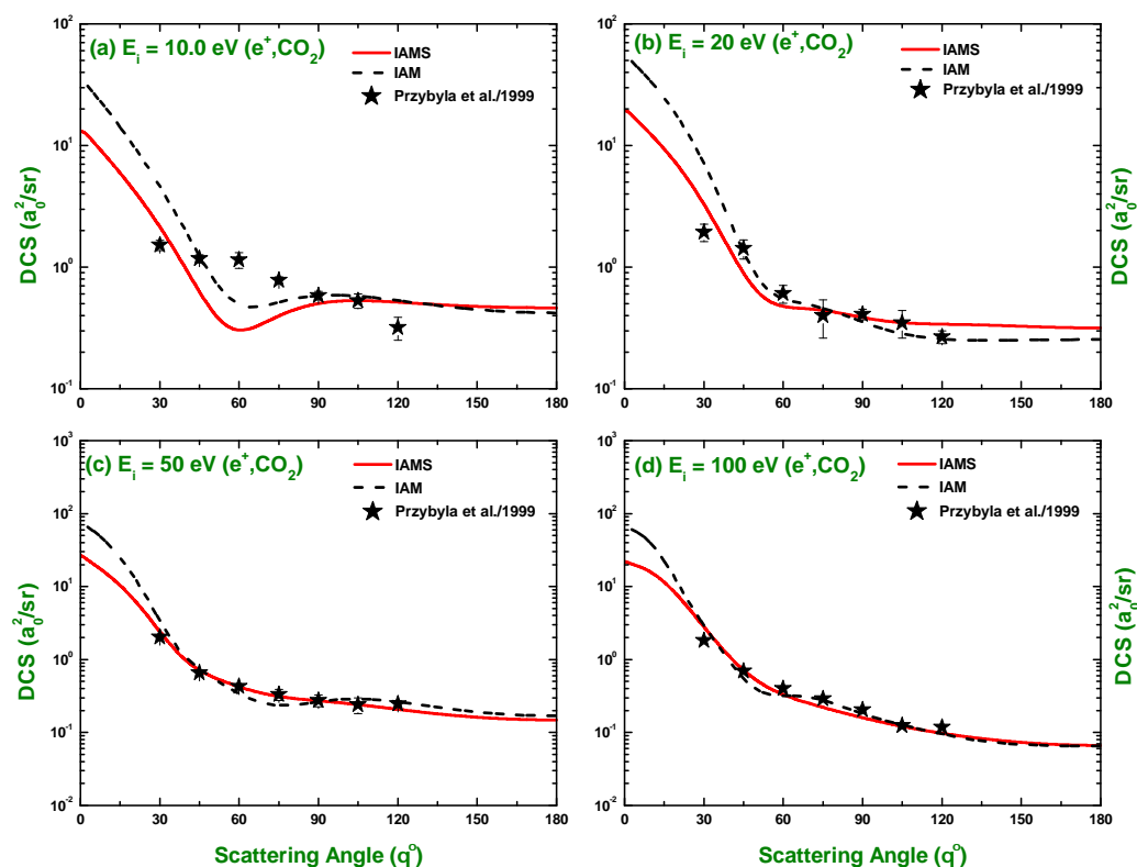
Figure 5. DCS ( a_0^2/\text{sr} ) for the elastic scattering of positrons from carbon dioxide at energies of 10, 20, 50, and 100 eV. Theoretical: IAM and IAMS. Experimental: Przybyla et al. [53].
