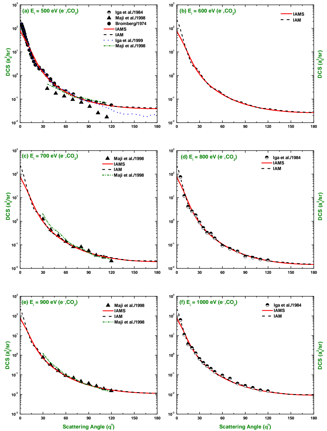
Figure 3. DCS ( a_0^2/\text{sr} ) for the elastic scattering of electrons from carbon dioxide at energies of 500, 600, 700, 800, 900, and 1000 eV. Theoretical: References in Figure 1. Experimental: References in Figures 1 and 2 and Maji et al. [51].
