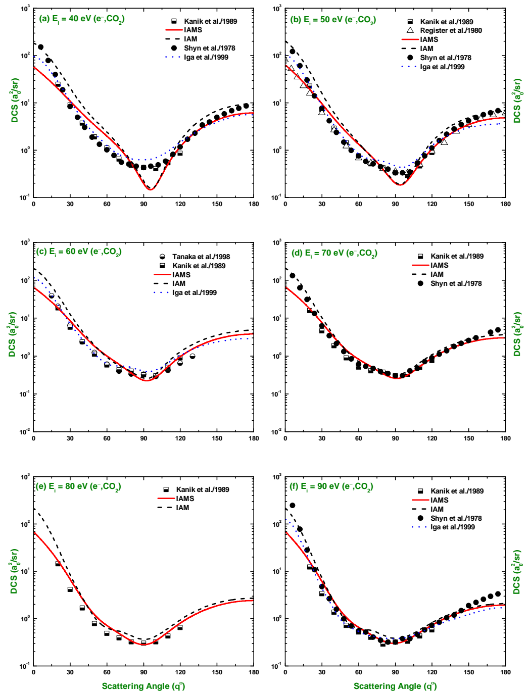
Figure 1. DCS ( a_0^2/\text{sr} ) for the elastic scattering of electrons from carbon dioxide at energies of 40, 50, 60, 70, 80, and 90 eV. Theoretical: IAM, IAMS, and Iga et al. [45]. Experimental: Tanaka et al. [46], Shyn et al. [47], Register et al. [48], and Kanik et al. [49].
