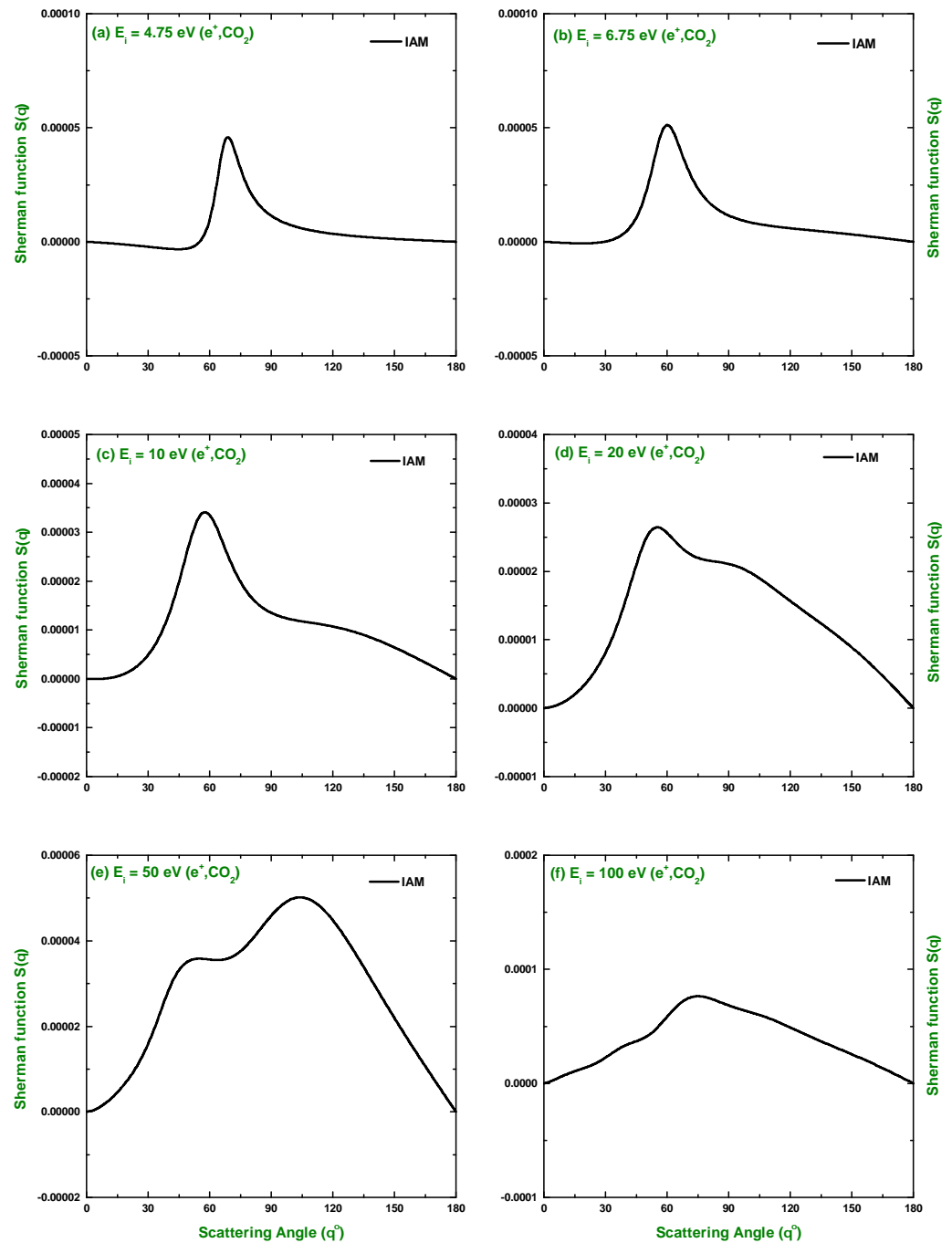
Figure 15. Angular dependence of the spin polarization of scattered positrons.
