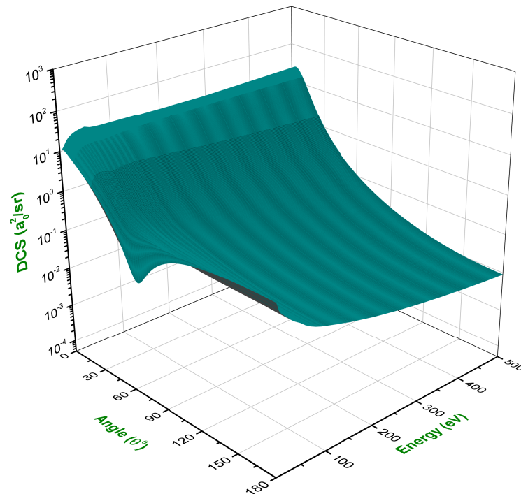
Figure 12. Variation of the DCS ( a_0^2/sr ) for the elastic scattering of positrons from carbon dioxide.
