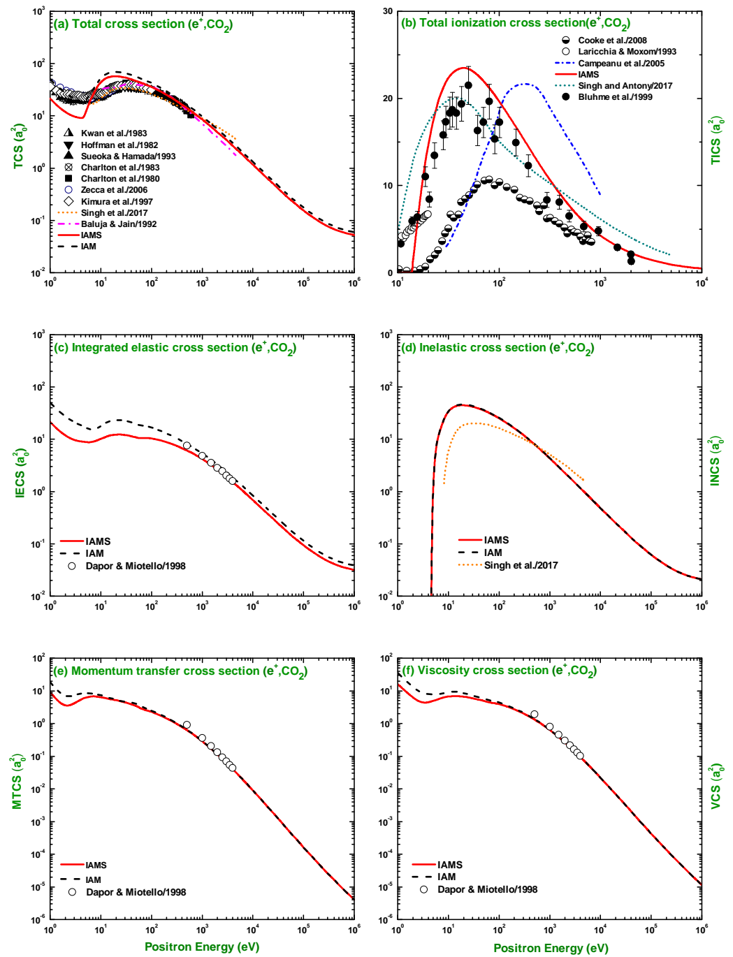
Figure 17. Values ( \text{a}_0^2 ) of TCS, TICS, IECS, INCS, MTCS, and VCS for the scattering of positrons from carbon dioxide. Theoretical: IAM, IAMS, Singh et al. [3], Baluja and Jain [27], Campeanu et al. [28], Dapor and Miotello [54] and Singh and Antony [77]. Experimental: Laricchia and Moxom [22], Sueoka and Hamada [23], Bluhme et al. [24], Cooke et al. [26], Kwan et al. [57], Hoffman et al. [61], Kimura et al. [72], Charlton et al. [74,75], and Zecca et al. [76].
