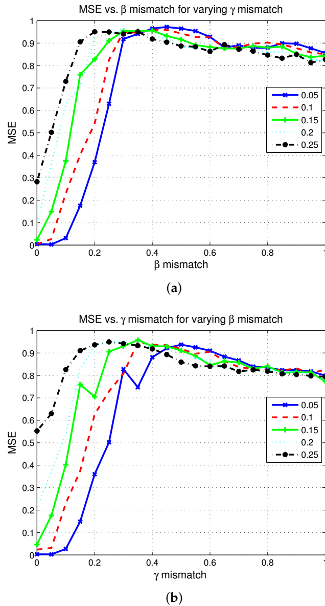
Figure 5. (a) Mean square error (MSE) versus \beta mismatch with varying \gamma mismatch. Increasing \gamma mismatch causes increase of error for the same level of \beta mismatch; (b) MSE versus \gamma mismatch with varying \beta mismatch. Increasing \beta mismatch causes the increase of error for the same level of \gamma mismatch.
