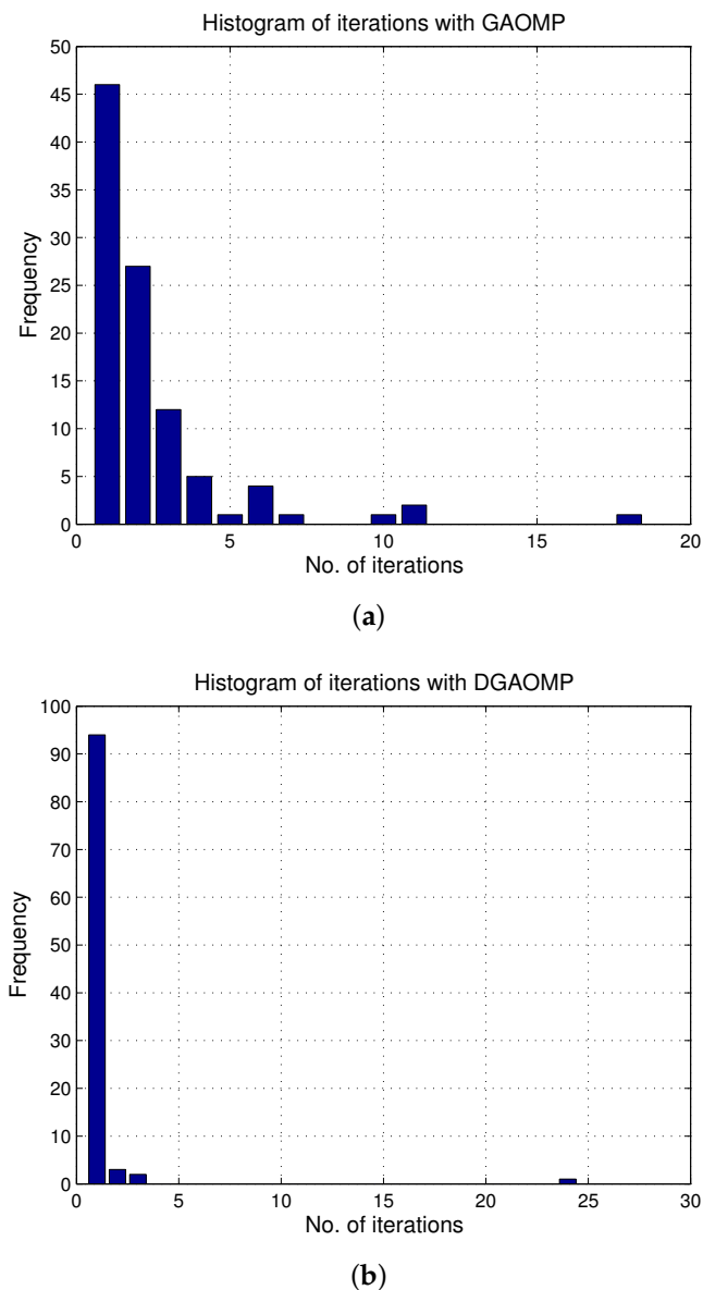
Figure 8. (a) Histogram of iterations for GAOMP. The success rate for single iteration is around 45%. One iteration represents three repetitions of the OMP algorithm. (b) Histogram of iterations for the technique of DGAOMP. The success rate for single iteration is more than 90%. One iteration represents three repetitions of the OMP algorithm.
