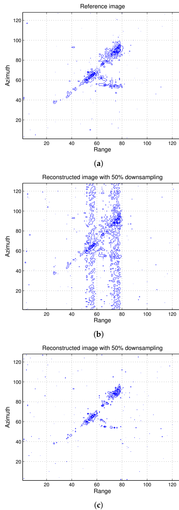
Figure 1. (a) Reference image; (b) reconstructed image using FT with 50% downsampled data; aliasing effects can be seen; (c) reconstructed image using Dictionary-based Genetic Algorithm Orthogonal Matching Pursuit (DGAOMP). The image is reconstructed without any artifacts.
