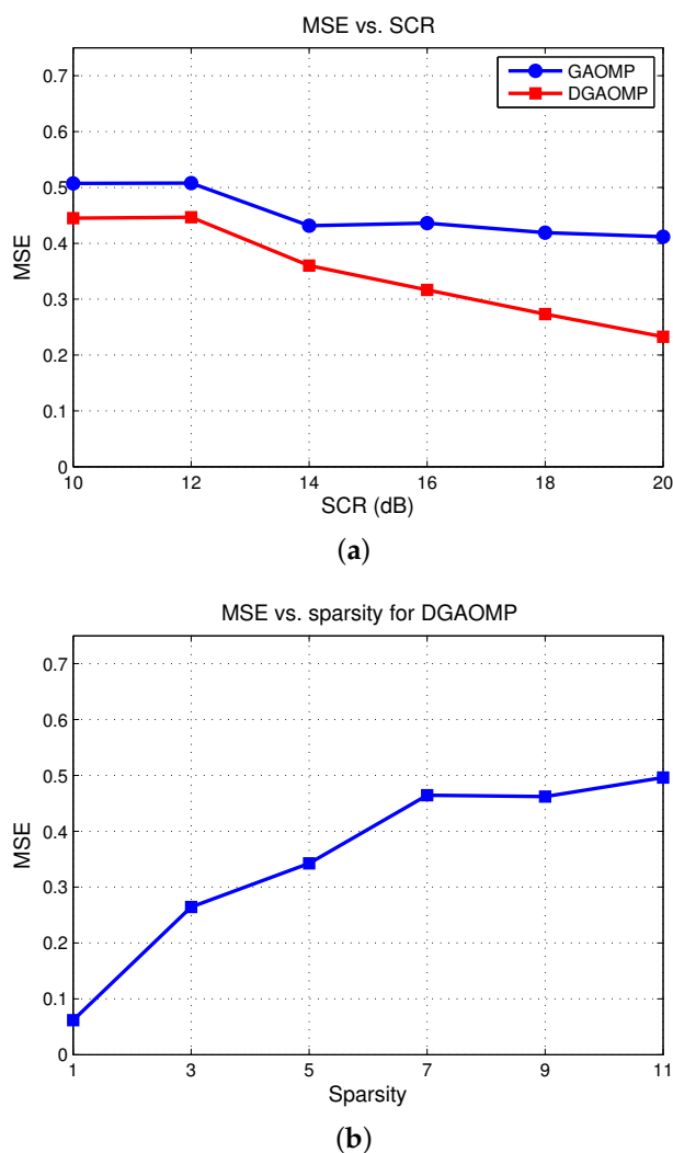
Figure 9. (a) MSE versus Signal-to-Clutter Ratio (SCR) for GAOMP and DGAOMP. The error is more for GAOMP. (b) MSE versus sparsity for DGAOMP. Increasing sparsity leads to a higher error.
