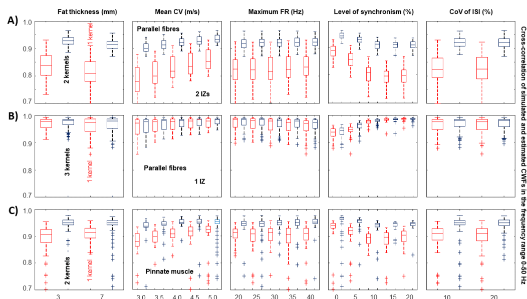
Figure 5. Cross-correlation of the low frequency contributions (up to 50 Hz) of the simulated CWF and estimated by either the single-kernel (red) or multi-kernel method (black). Each estimation was obtained considering single channel SD EMG at 80% MVC with a duration of 10 s. Data are shown after pooling with respect to specific values of fat layer thickness, mean MU CV, maximal FR, level of synchronization of MU firings, and CoV of ISI. Different simulation models are considered: (A) cylindrical volume conductor with parallel fibres and two IZs (50% of MUs innervated under each IZ; uniform distribution of MU size among different IZs); (B) same volume conductor as in (A), but considering a single IZ; (C) pinnate muscle with fibre inclined with respect to the skin surface.
