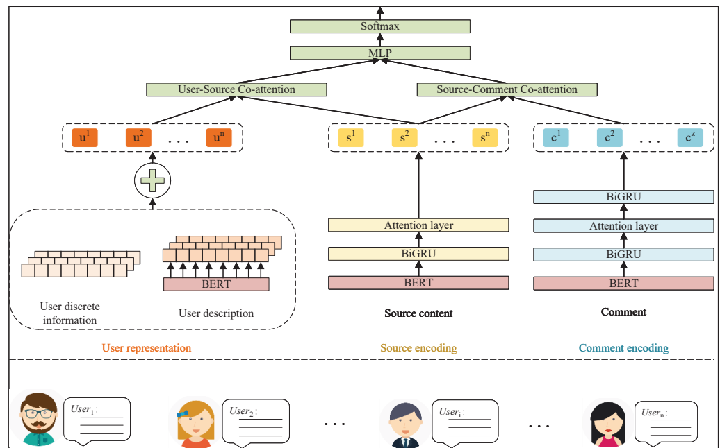
Figure 1. Overall network model architecture.
