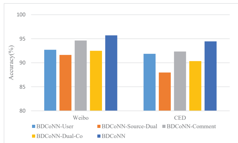
Figure 4. Results of the ablation experiments on the Weibo and CED datasets.
