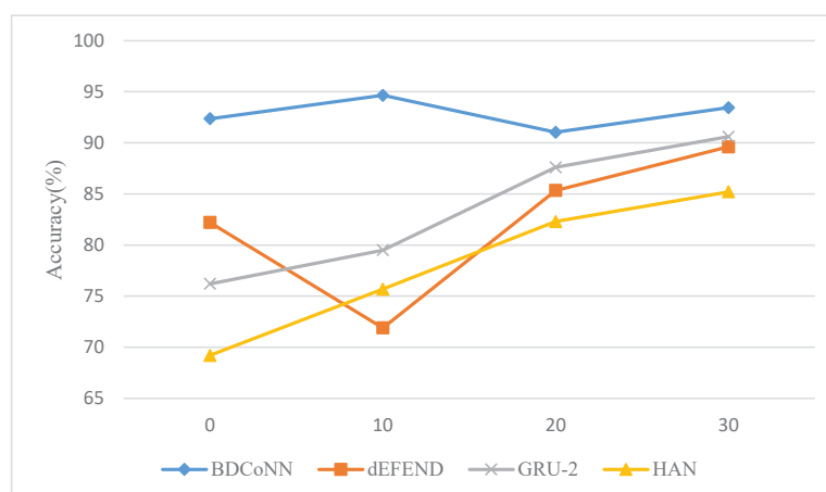
Figure 6. Accuracy of CED's early rumor detection.
