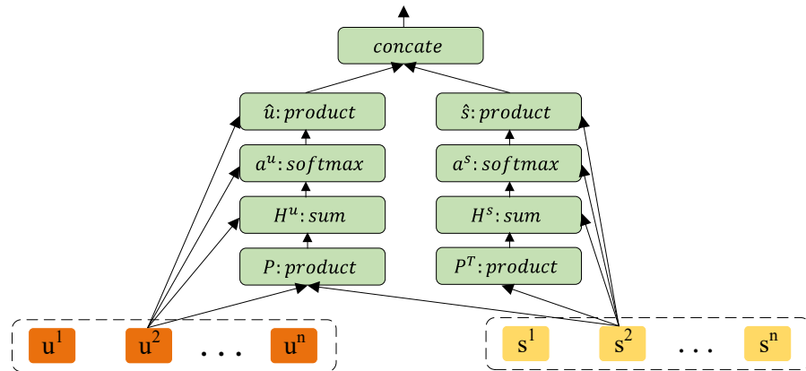
Figure 3. User-source co-attention module.
