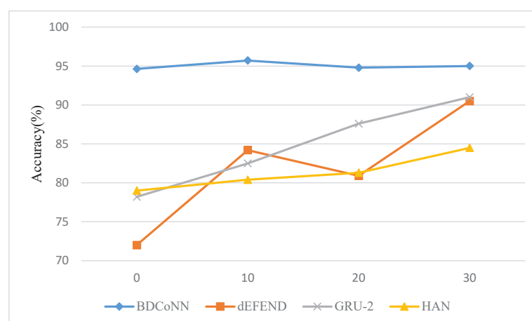
Figure 5. Accuracy of early rumor detection on the Weibo dataset.
