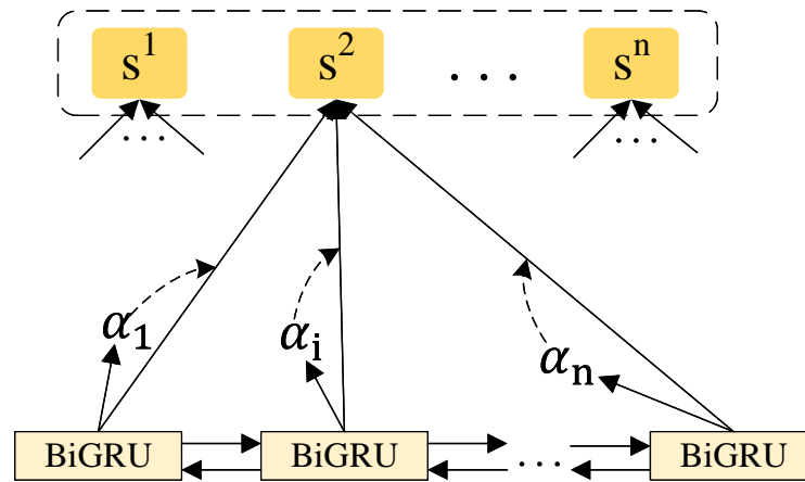
Figure 2. Attention layer.
