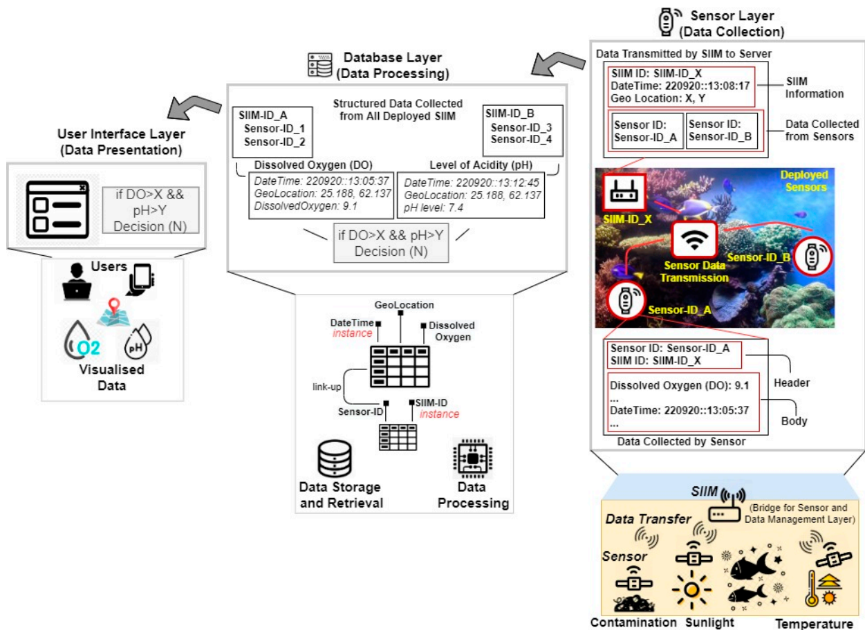
Figure 4. Developing design model flow for IoUT.
