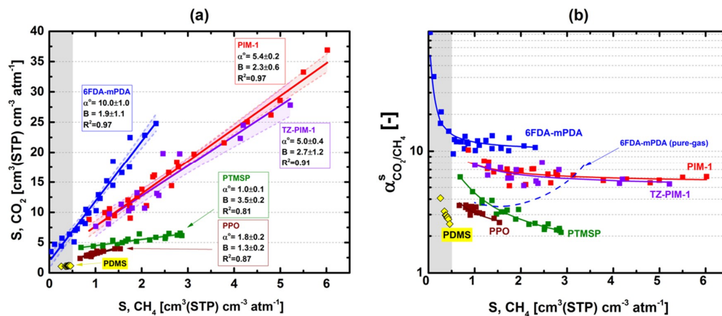
Figure 5. (a) CO 2 vs. CH 4 mixed-gas solubility coefficient of 6FDA-mPDA at 35 °C—solid lines were estimated via linear fitting of experimental data (the dotted curves delimit the confidence intervals of each linear interpolation); (b) data of CO 2 /CH 4 mixed-gas solubility selectivity vs. CH 4 mixed-gas solubility coefficient of 6FDA-mPDA (CO 2 /CH 4 mixed-gas solubility selectivity vs. CH 4 mixed-gas solubility coefficient mixed- (solid line) and pure-gas trends (dashed-line) are also shown for comparison). Mixed-gas solubility coefficient data from previous reports on PDMS [11], PIM-1 [20], TZ-PIM-1 [23], PTMSP [15], and PPO [18] are included in (a,b).
