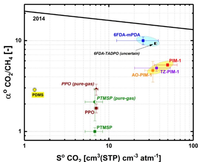
Figure 6. CO_2 solubility coefficient vs. CO_2/CH_4 solubility selectivity (at infinite dilution) data of all polymers tested for CO_2 - CH_4 mixed-gas sorption at 35 °C [11,15,18,20,22,23,48]. CO_2/CH_4 solubility selectivities were obtained from linear interpolation of CO_2 mixed-gas solubility coefficient vs. CH_4 mixed-gas solubility coefficient data or from pure-gas uptake data via DMS model equations—see the discussion in the Supporting Information and data values in Table S2. CO_2 solubility coefficients were estimated from experimental data of pure-gas CO_2 uptake. The 2014 CO_2/CH_4 solubility upper bound was discussed elsewhere [47].
