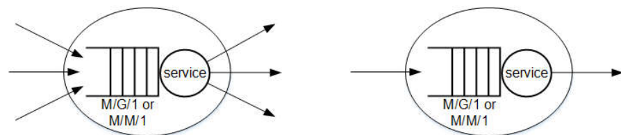
Figure 3. Model of CSCF servers, RACF C1, RACF C2 (left) and links (right).
