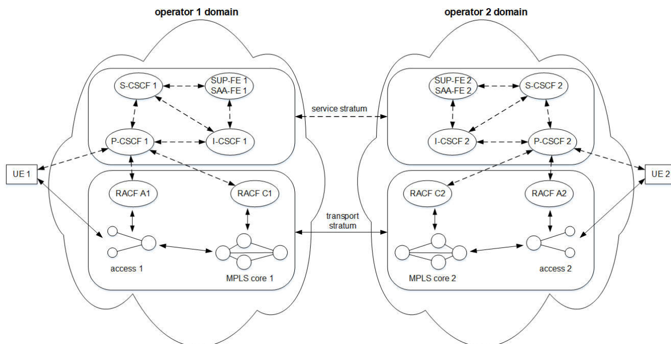
Figure 1. Structure of the multidomain IMS/NGN network with an MPLS-based transport stratum.
