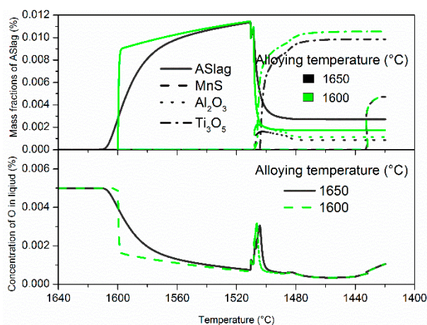
Figure 3. The mass fraction changes of the inclusions during the cooling and solidification process ( top ) and the corresponding changes of oxygen concentration ( bottom ) at the alloying temperatures of 1650 and 1600 °C.
