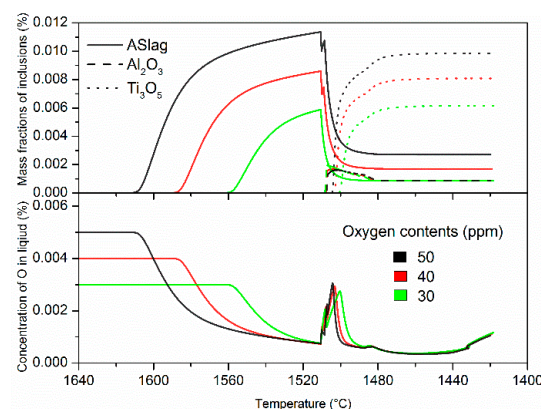
Figure 8. Influence of oxygen content on the mass fraction of inclusions (top) and the corresponding oxygen concentration changes (bottom).
