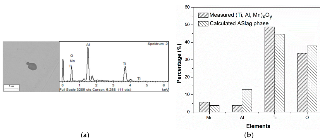
Figure 4. (a) Morphology and EDS analysis of (\text{Ti, Al, Mn})_x\text{O}_y ; (b) comparison of the composition of the calculated ASlag and measured (\text{Ti, Al, Mn})_x\text{O}_y [15].
