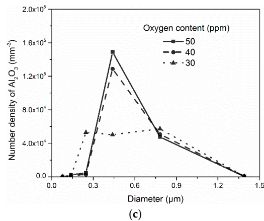
Figure 9. Influence of oxygen content on the size distribution of (a) ASlag, (b) \text{Ti}_3\text{O}_5 and (c) \text{Al}_2\text{O}_3 at solidus temperature.
