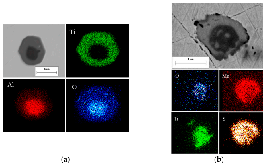
Figure 5. Typical heterogeneous inclusions in steel B: (a) \text{Al}_2\text{O}_3 - \text{TiO}_x and (b) \text{TiO}_x -MnS [15].
