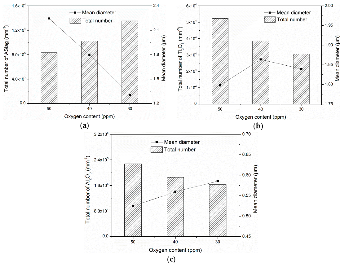
Figure 10. Influence of oxygen content on the number and mean diameter of (a) ASlag, (b) \text{Ti}_3\text{O}_5 and (c) \text{Al}_2\text{O}_3 .
