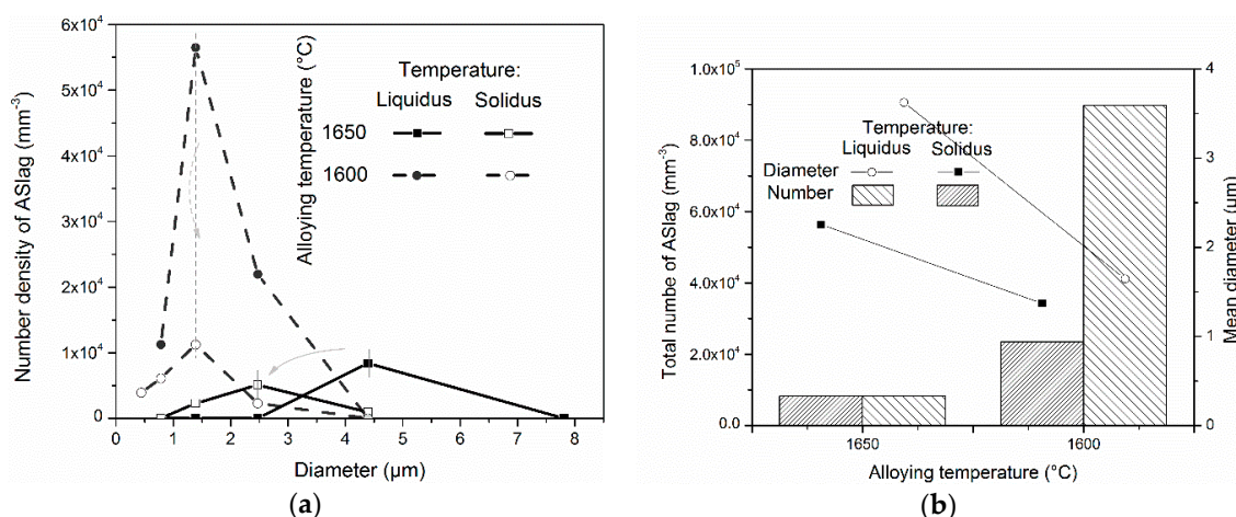
Figure 6. The influence of alloying temperature on ASlag (a) size distribution and (b) mean diameter and total number at solidus and liquidus temperature.
