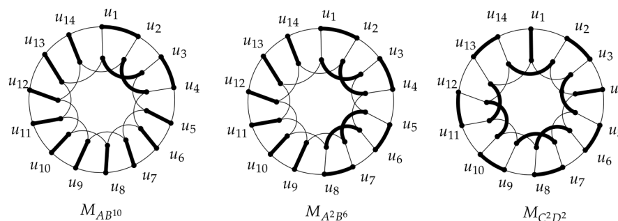
Figure 4. For i = 1 , the perfect matchings M_{A_i^h B^h} ( h \in \{1, 2\} ) and M_{C_i^2 D^{p-1}} of GP(14, 2) . Here, bold lines denote the edges in the perfect matching.
