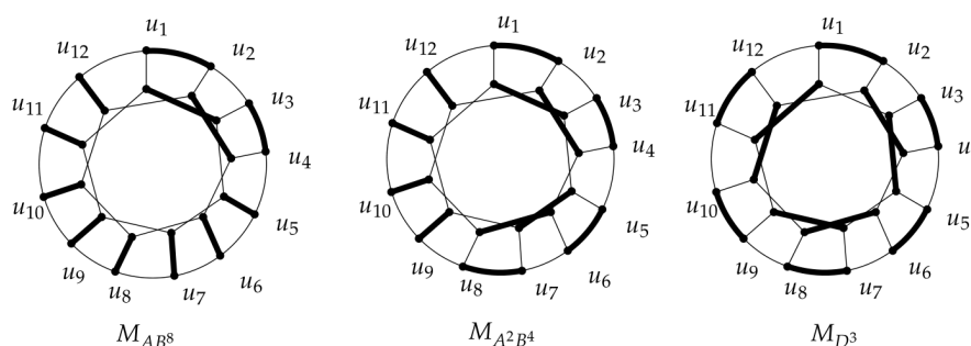
Figure 3. For i = 1 , the perfect matchings M_{A_i^h B^s} ( h \in \{1, 2\} ) and M_{D_i^p} of GP(12, 2) . Here, bold lines denote the edges in the perfect matching.
