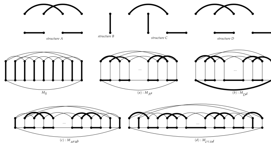
Figure 1. All types of perfect matchings of GP(n,2) . Here, bold lines denote the edges in the perfect matching.
