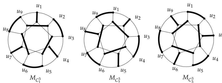
Figure 2. The matching M_{C_i^3} ( i \in \{1, 2, 3\} ) of GP(9, 2) . Here bold lines denote the edges in the perfect matching.
