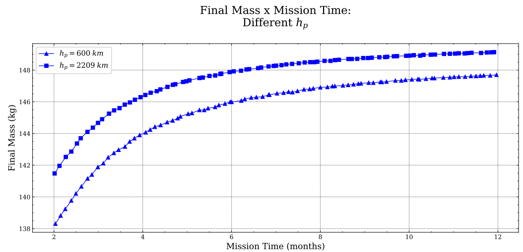
Figure 17. Final mass as a function of mission time for the two initial perigee heights chosen ( h_p = 600 km and h_p = 2209 km) and considering the NEXT propulsion system ( T = 236 mN e I_{sp} = 4190 s), with e = 0 and i_{moon} = 18^\circ .
