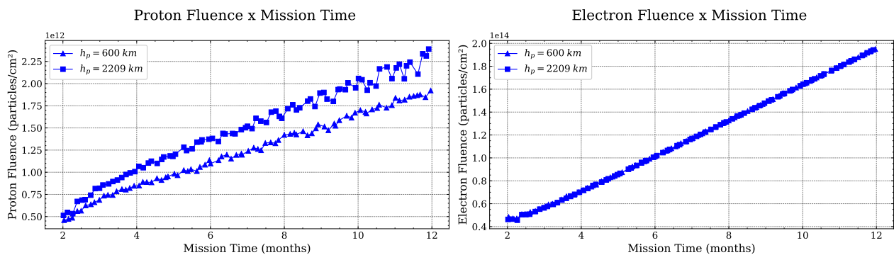
Figure 14. Particle fluence as a function of mission time for the two initial perigee heights chosen ( h_p = 600 km and h_p = 2209 km) and considering the propulsion system NEXT ( T = 236 mN e I_{sp} = 4190 s), with e = 0 and i_{moon} = 18^\circ .
