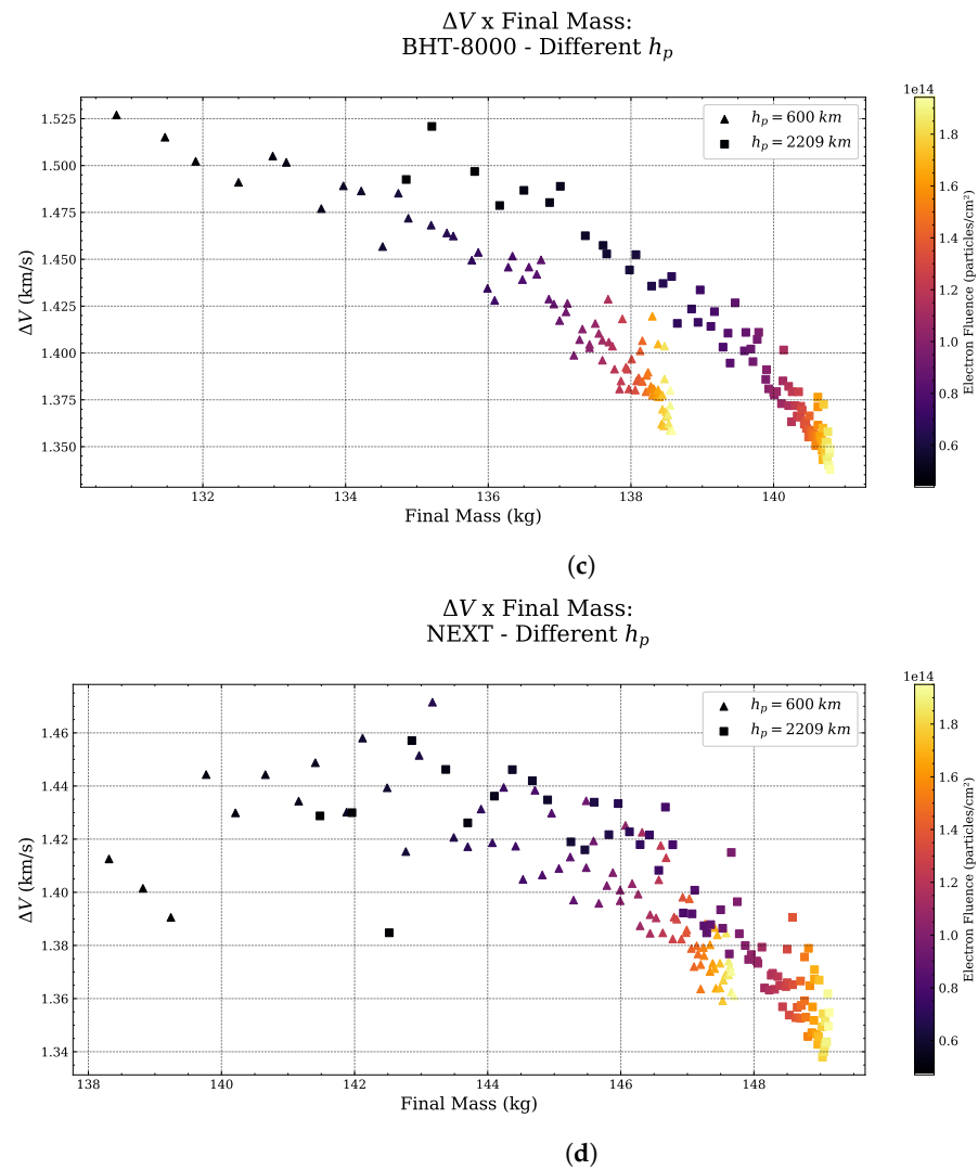
Figure 32. Gain in velocity as a function of the final mass, where the color of the dots represents the fluence of electrons, for the two initial perigee heights chosen ( h_p = 600 km and h_p = 2209 km), with e = 0 , i_{moon} = 18^\circ and R_p = 1910.7 km. (a) Ionic propulsion system. (b) PPS-1350 propulsion system. (c) BHT-8000 propulsion system. (d) NEXT propulsion system.
