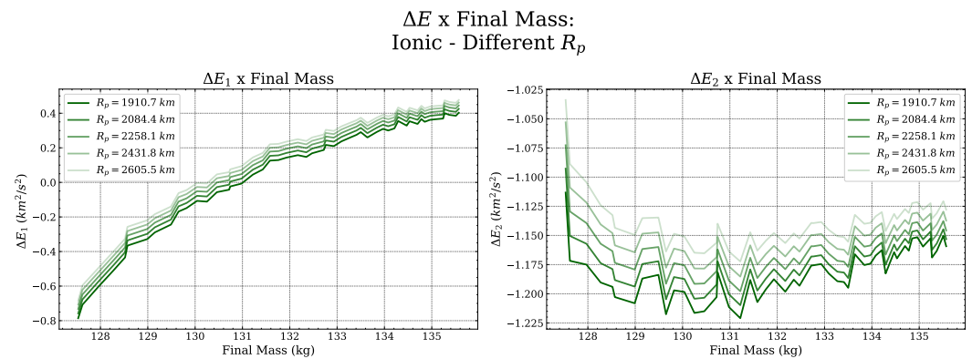
Figure 29. Energy gain, in its two configurations, as a function of the final mass for the five approximation distances R_p chosen initials (1910.7; 2084.4; 2258.1; 2431.8; 2605.5 km) and considering the ionic propulsion system, h_p = 600 km, e = 0 km, i_{moon} = 18^\circ .
