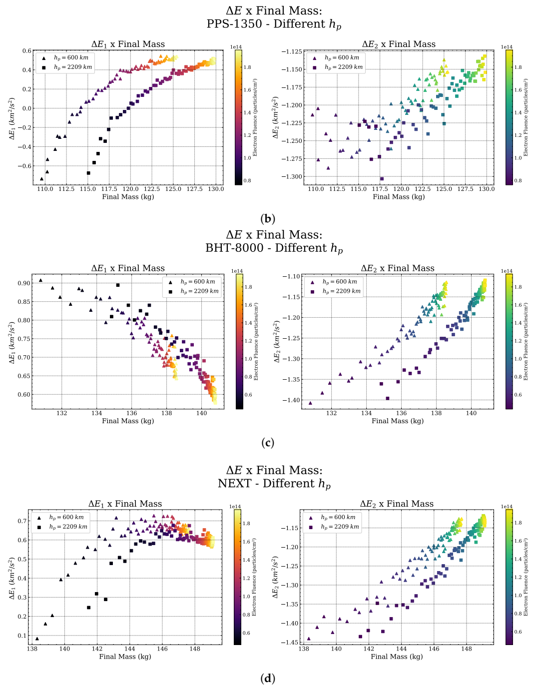
Figure 28. Energy gain, in its two configurations, as a function of the final mass, where the color of the dots represents the fluence of electrons, for the two initial perigee heights chosen ( h_p = 600 km and h_p = 2209 km), with e = 0 , i_{moon} = 18^\circ and R_p = 1910.7 km. (a) Ionic propulsion system. (b) PPS-1350 propulsion system. (c) BHT-8000 propulsion system. (d) NEXT propulsion system.
