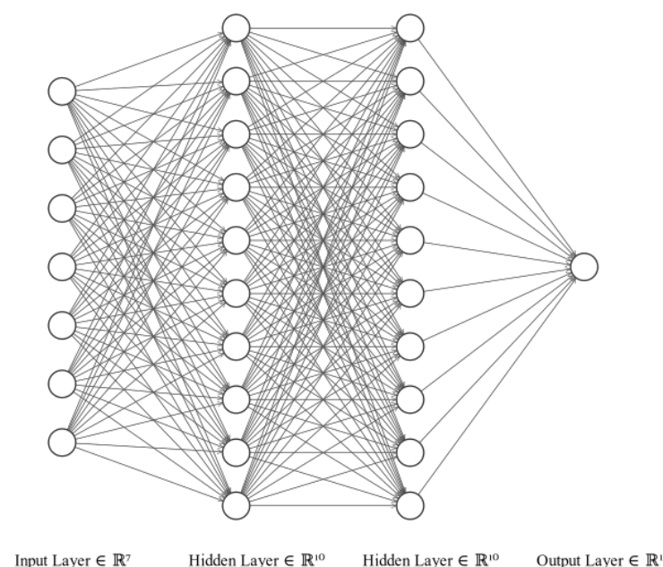
Figure 9. Neural network with two hidden layers of 10 neurons (MDPI: please delete the blank in bottom.).
