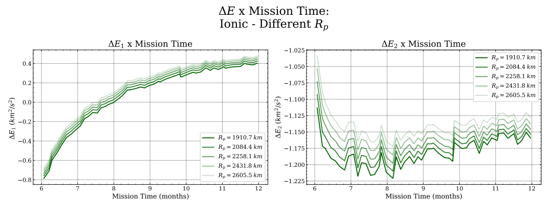
Figure 21. Energy gain, in its two configurations, as a function of mission time for the five approach distances R_p chosen initially (1910.7; 2084.4; 2258.1; 2431.8; 2605.5 km) and considering the ionic propulsion system, h_p = 600 km, e = 0 km, i_{moon} = 18^\circ .
