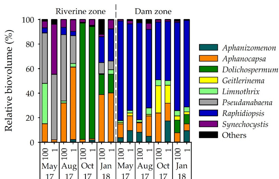
Figure 3. Relative biovolume (%) of cyanobacterial genera identified in Itupararanga reservoir. Others = Aphanothece , Chroococcus , Cuspidothrix , Merismopedia , Microcystis , Phormidium , Glaucospira and Limnocooccus ; 100 = surface; 1 = lower limit of euphotic zone.
