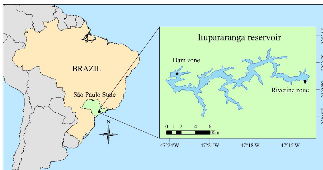
Figure 1. Sampling sites in the Itupararanga reservoir, São Paulo State, Brazil. Itupararanga riverine zone (23°37'24.8" S, 47°13'53.4" W); Itupararanga dam zone (23°36'50.7" S, 47°23'27.3" W).
