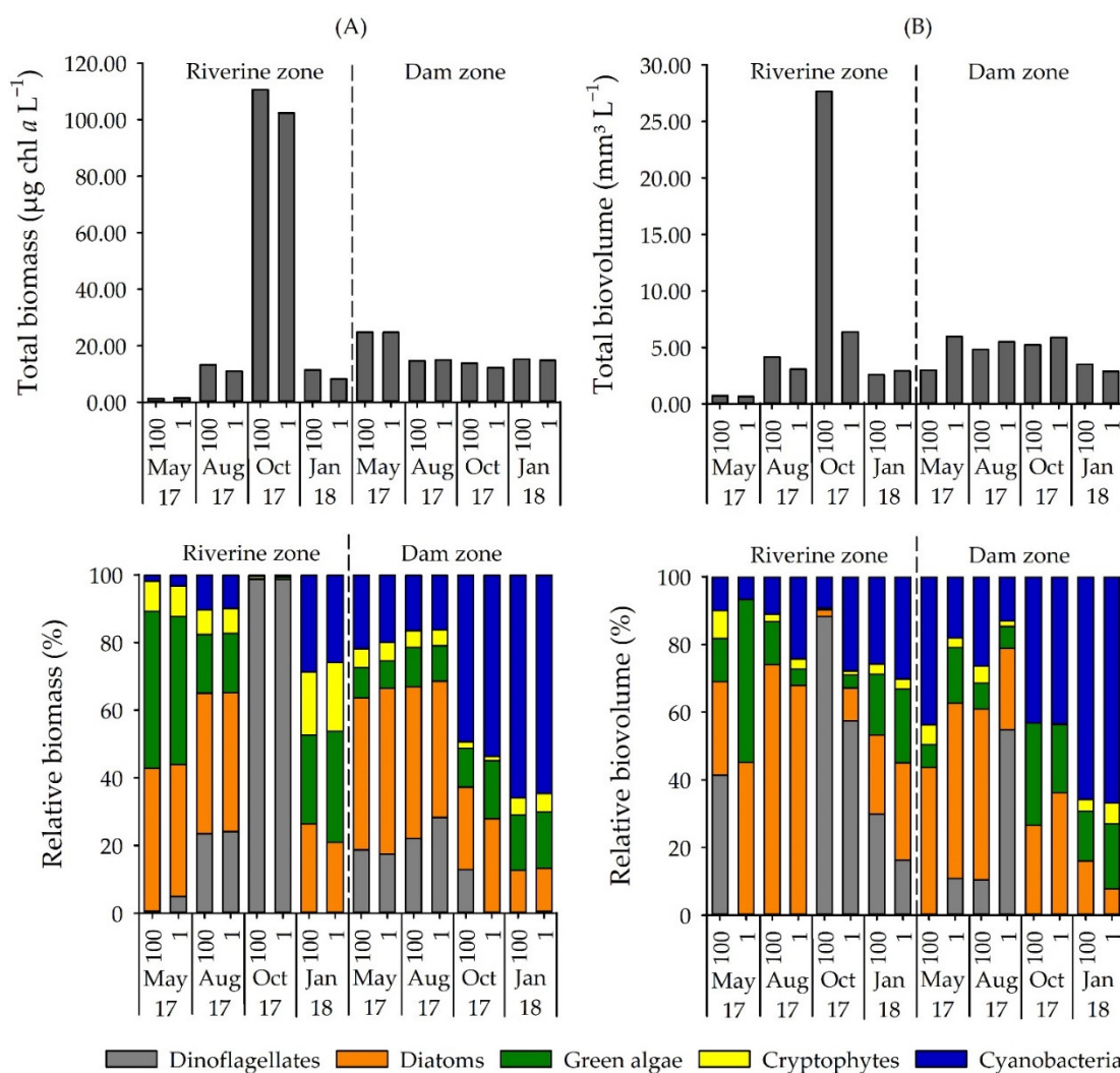
Figure 2. (A) Total biomass ( \mu\text{g chl } a \text{ L}^{-1} ) and relative biomass (%) of phytoplankton groups determined by the pigment method and (B) total biovolume ( \text{mm}^3 \text{ L}^{-1} ) and relative biovolume (%) of phytoplankton groups in Ituparanga reservoir. 100 = surface; 1 = lower limit of euphotic zone.
