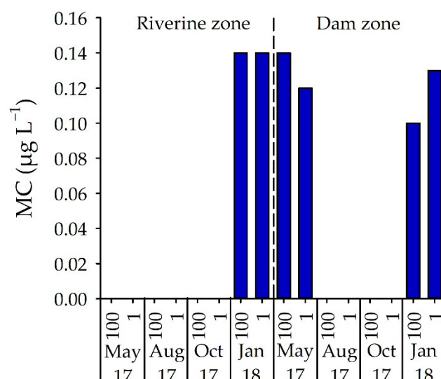
Figure 6. MC concentration ( \mu\text{g L}^{-1} ) in samples from two field stations, in four months and two depths in Ituparanga reservoir. 100 = surface; 1 = lower limit of euphotic zone.
