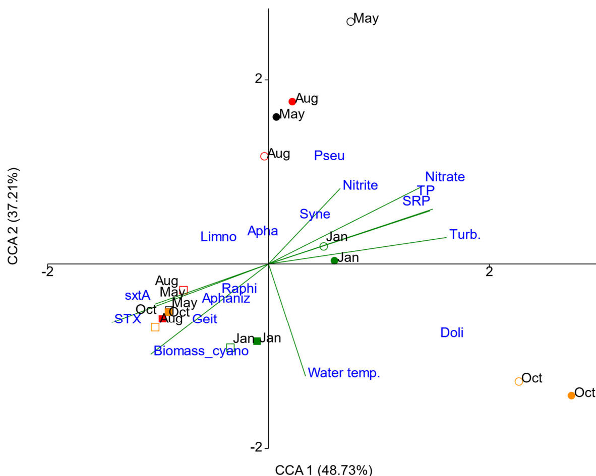
Figure 7. Canonical correspondence analysis (CCA) biplot of cyanobacteria biovolume and environmental variables in Itupararanga reservoir. The periods of sampling were May (May 2017, black), Aug (August 2017, red), Oct (October 2017, orange) and Jan (January 2018, green); the riverine zone is represented by dot and dam zone is represented by square;
