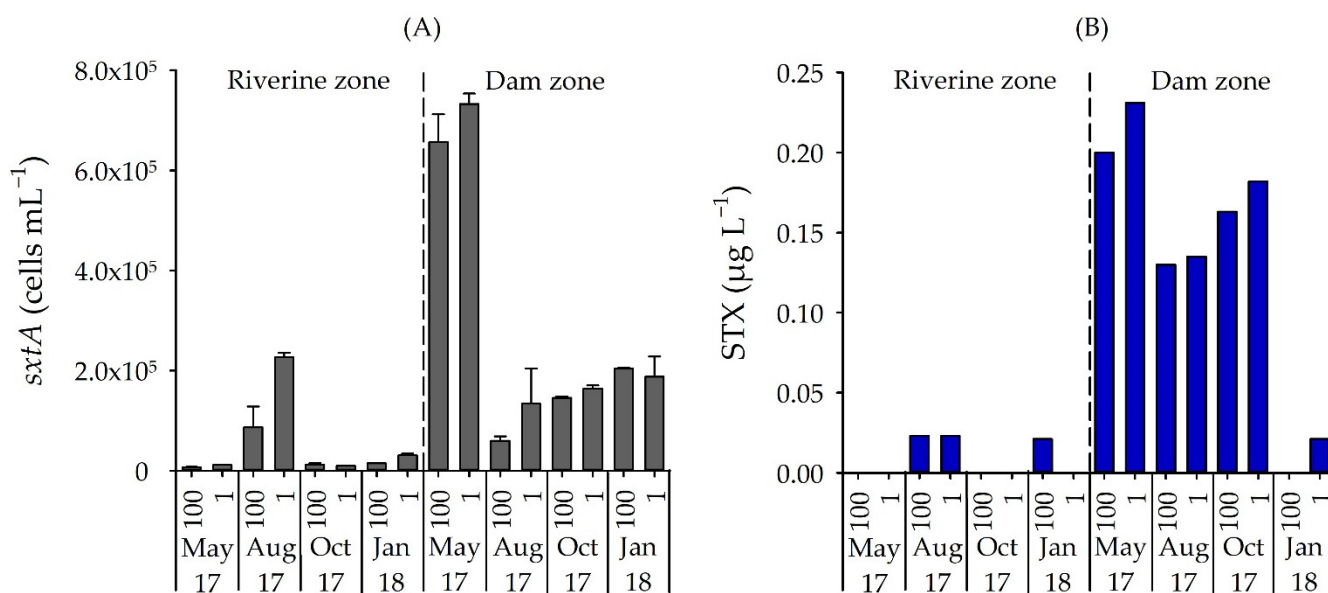
Figure 5. (A) Number of sxtA gene (cells mL -1 ) and (B) STX concentration (μg L -1 ) in samples from two field stations, in four months and two depths in Itapararanga reservoir. Standard deviations of triplicate samples shown. 100 = surface; 1 = lower limit of euphotic zone.
