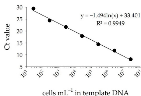
Figure 4. Standard curve of Ct values for tenfold dilutions of known DNA concentration of Raphidiopsis raciborskii T3 (cells \text{mL}^{-1} ). Error bars provide standard deviations of triplicate amplifications.
