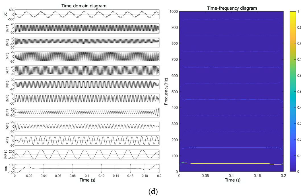
Figure 8. The time-frequency distribution of leakage current. (a) Unaged; (b) aging for 12 days; (c) aging for 24 days; (d) aging for 48 days.
