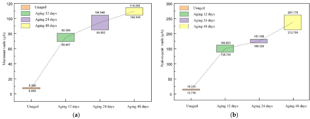
Figure 9. The distribution of dimensioned parameters in the time domain. (a) Maximum value; (b) peak-to-peak value.
