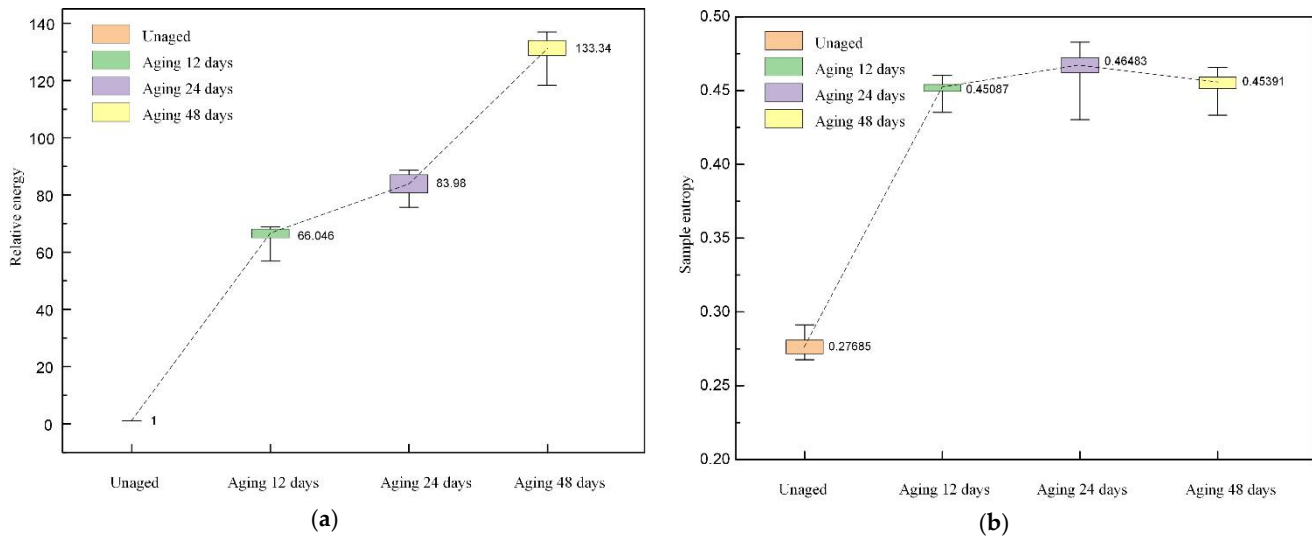
Figure 12. The distribution of relative energy and sample entropy. (a) Relative energy; (b) sample entropy.
