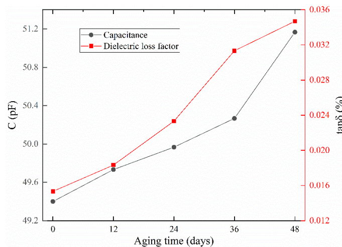
Figure 4. The changes in capacitance and dielectric loss factor of cable sample with aging time.
