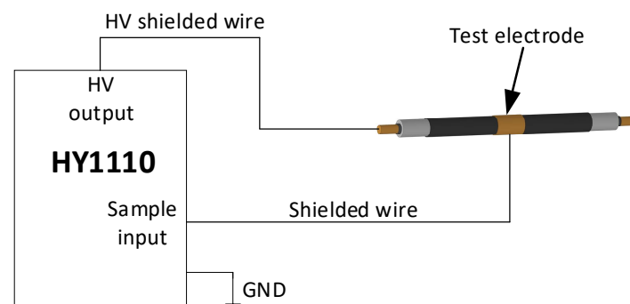
Figure 2. The cable capacitance and dielectric loss factor measurement device.
