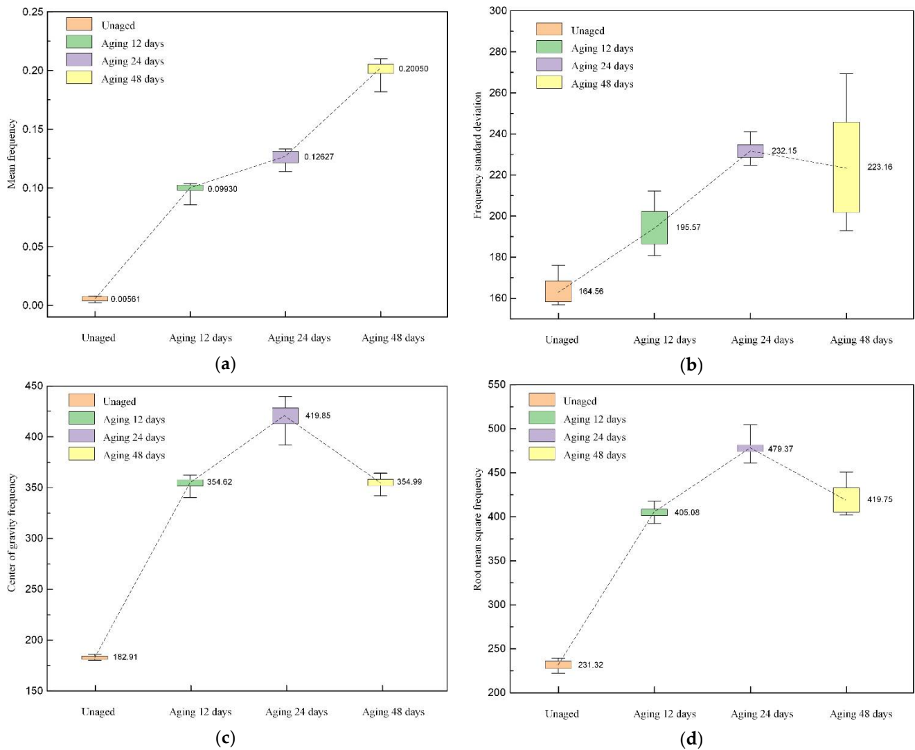
Figure 11. The distribution of frequency-domain parameters. (a) Mean frequency; (b) frequency standard deviation; (c) center of gravity frequency (d) root-mean-square frequency.
