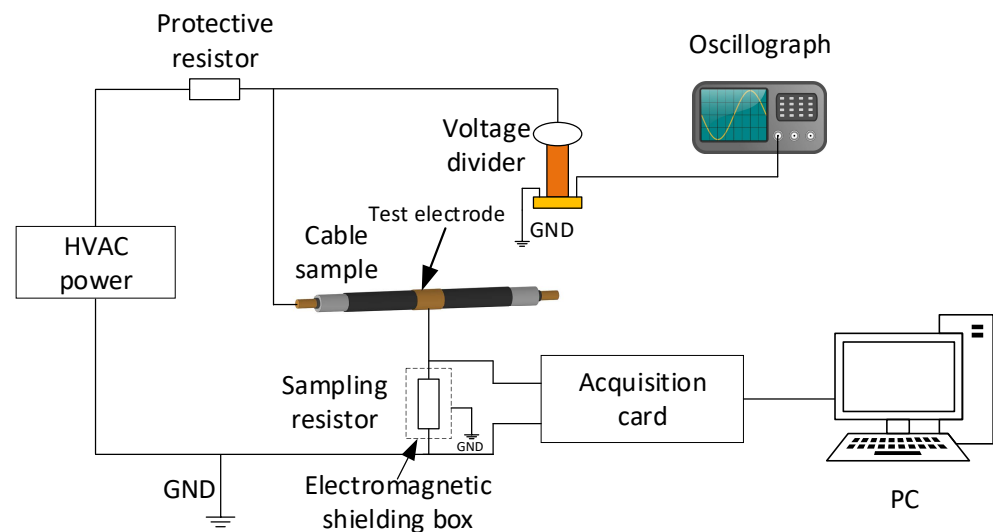
Figure 3. The AC leakage current test experimental setup.
