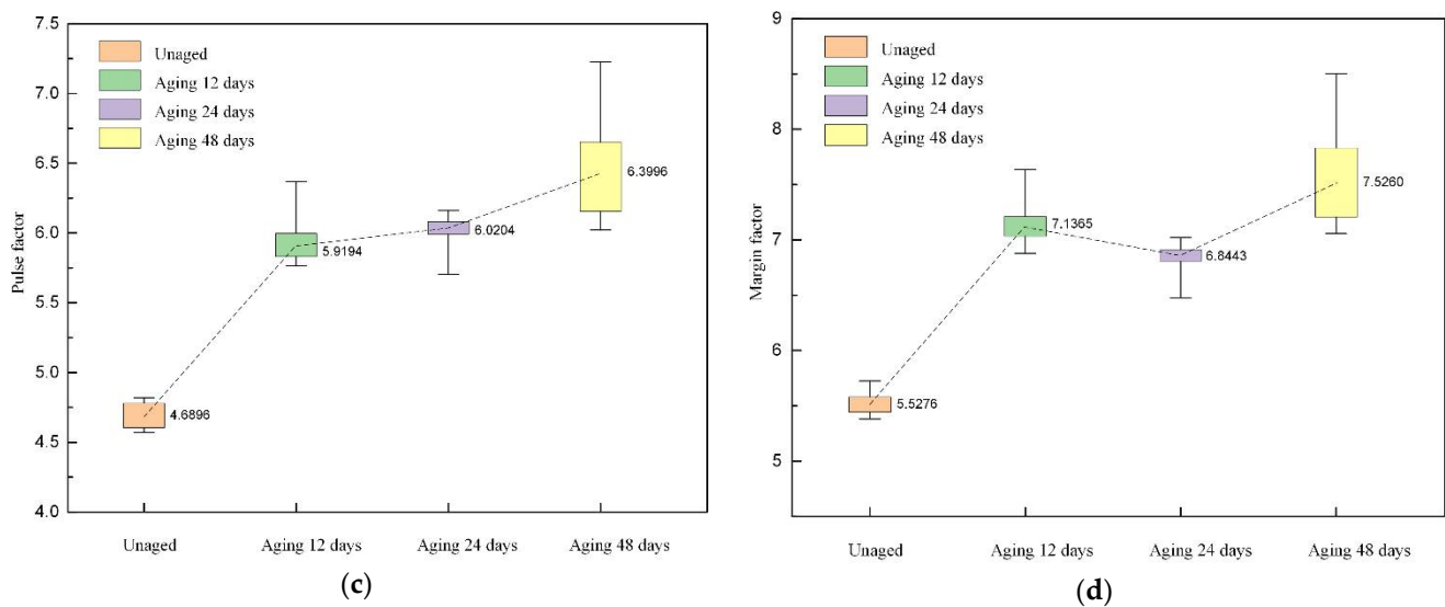
Figure 10. The distribution of dimensionless parameters in the time domain. (a) Waveform factor; (b) crest factor; (c) pulse factor; (d) margin factor.
