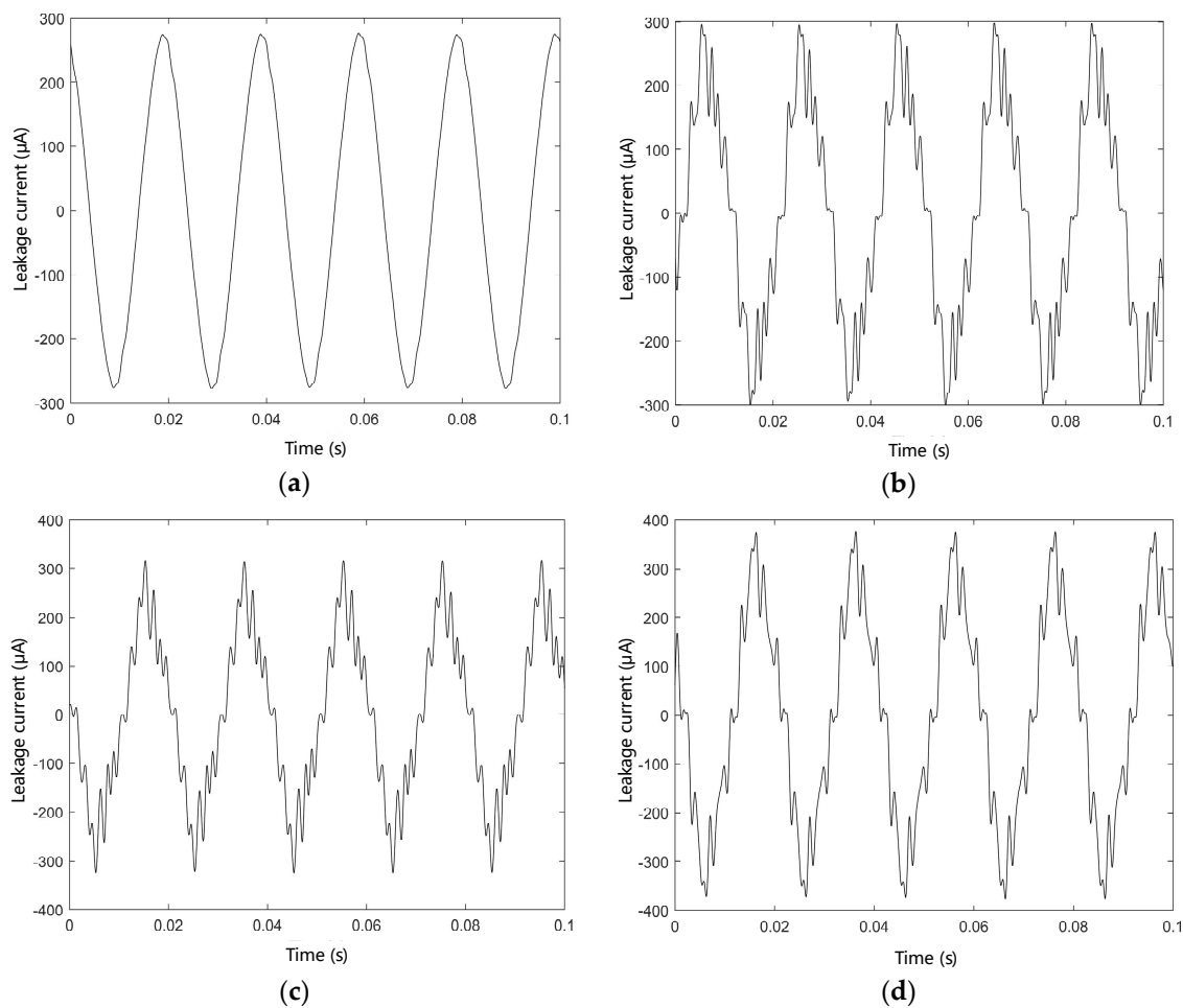
Figure 5. The leakage current test results of cable samples. (a) Unaged; (b) aging for 12 days; (c) aging for 24 days; (d) aging for 48 days.
