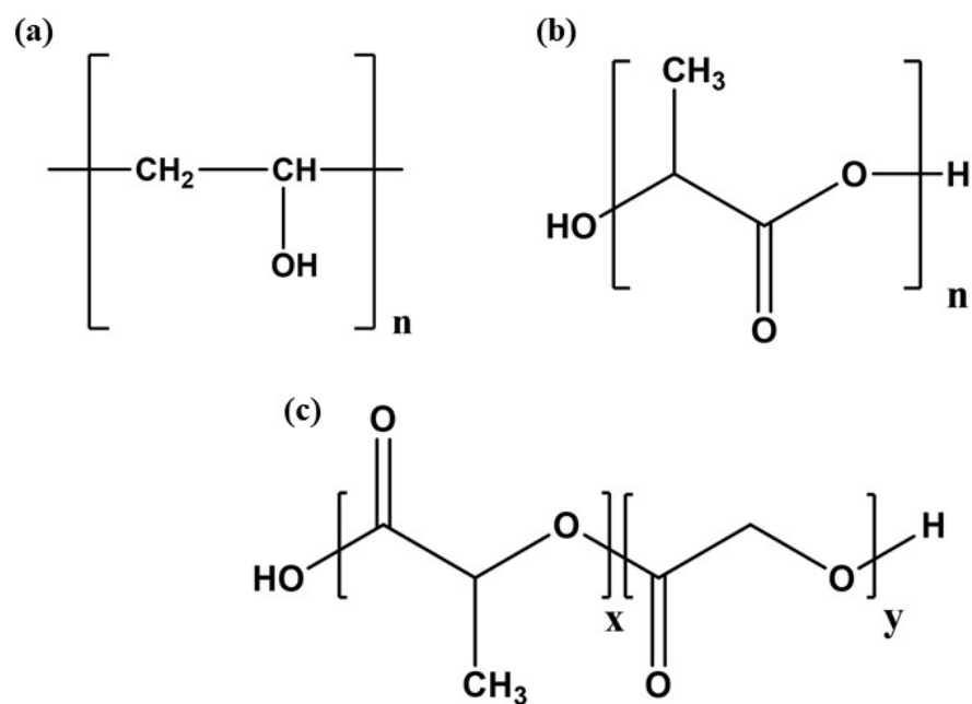
Figure 2. Chemical structure of synthetic polymers (a) Polyvinyl alcohol (PVA), (b) Polylactic acid (PLA), and (c) Poly(lactic-co-glycolic) acid (PLGA).
