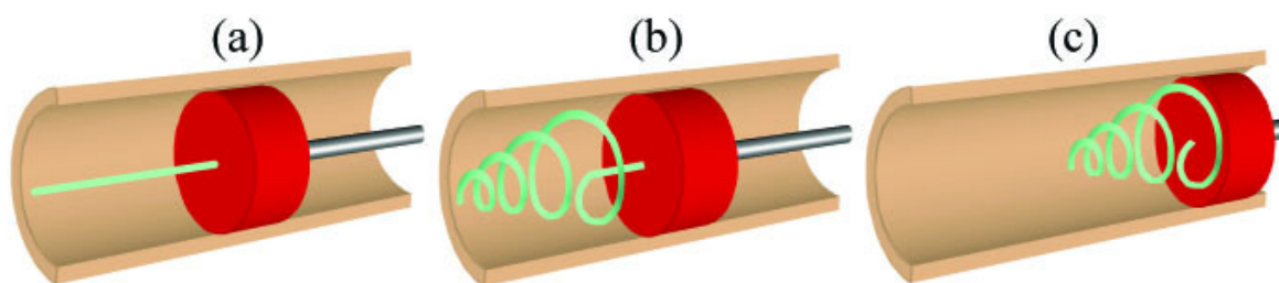
Figure 13. Representation of endovascular thrombectomy using the laser activated shape memory polymer micro actuator attached to an optical fiber. (a) In its secondary straight rod form, the micro actuator is delivered through a catheter distal to the thrombotic vascular occlusion. (b) Primary corkscrew form of micro actuator induced by laser heating. (c) The deployed micro actuator is retracted to capture the thrombus. (Reproduced with permission from [100] Copyright 2005, The Optical Society).
