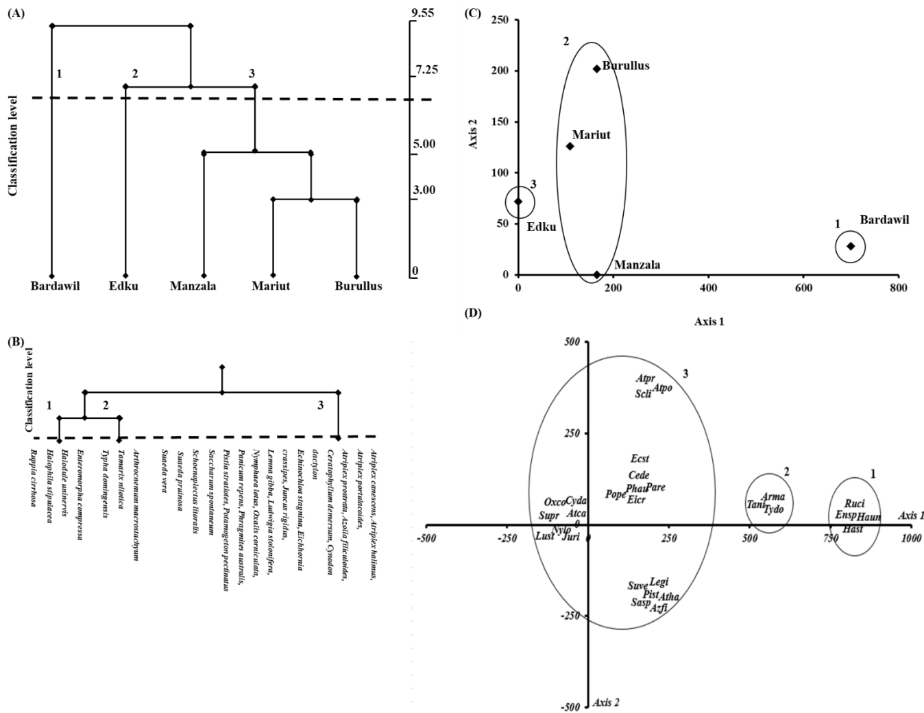
Figure 2. Classification of lakes and plant communities (A,B) after the application of the two-way species indicator analysis (TWINSPAN). Ordination results (C,D) from Detrended Correspondence Analysis technique (DCA) showing three vegetation groups for the five Egyptian northern lakes. For plant species abbreviation, see Table S2.
