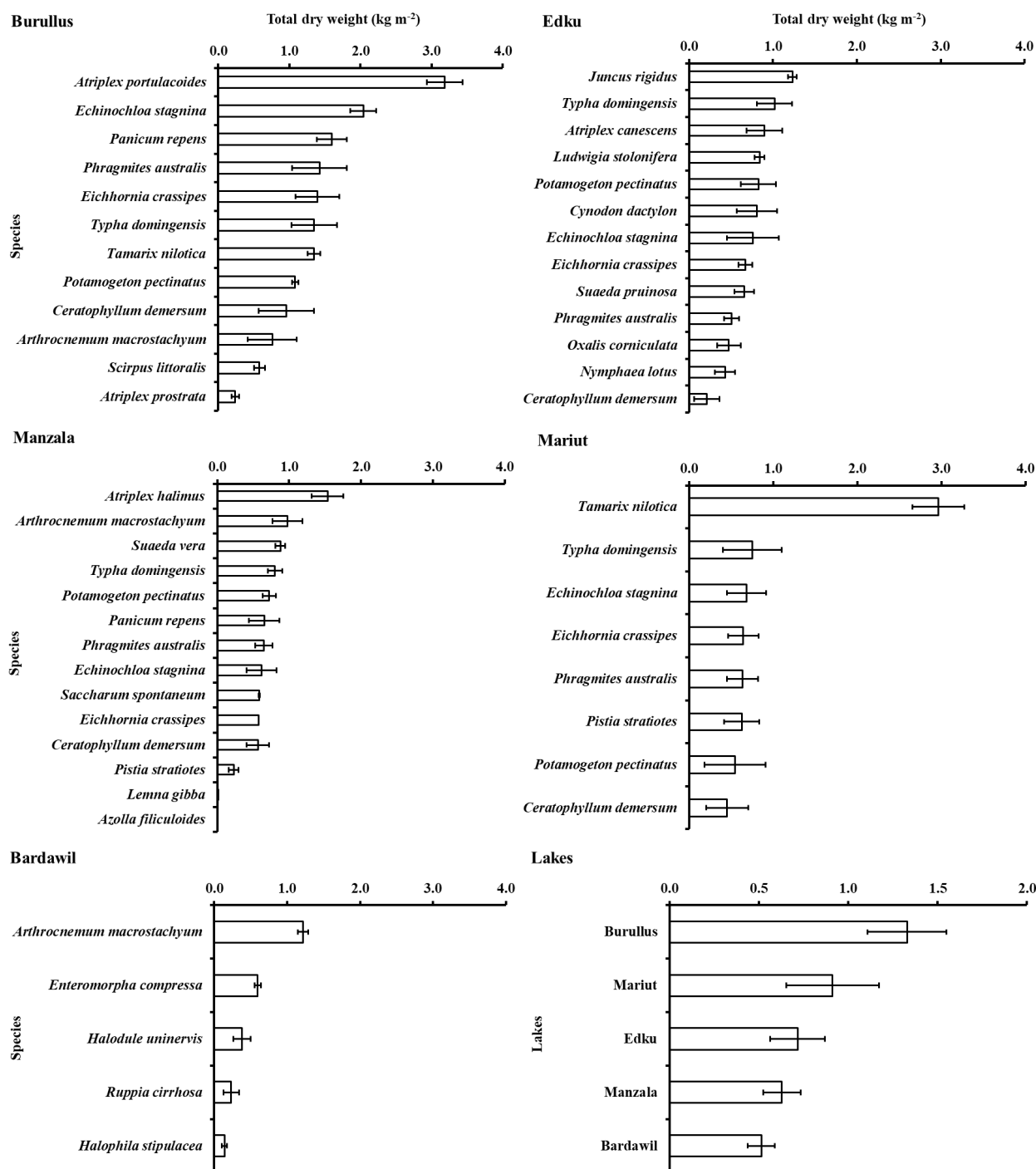
Figure 4. Aboveground biomass ( \text{kg dry weight m}^{-2} ) (mean \pm SE) for identified plant species in the Egyptian northern lakes.
