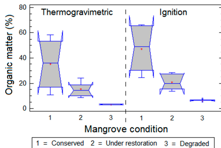
Figure 5. Analysis of variance using the Kruskal–Wallis method, where significant differences can be observed between the different mangrove conditions and different analytical techniques. The analysis shows the OM content in all the soil profiles. The median is indicated by the red cross.
