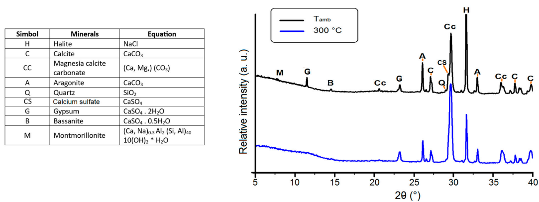
Figure 3. Mineral identification of a mangrove soil sample analyzed using a diffractogram, where a characteristic peak of hydrated calcium sulfates (gypsum, G, and bassanite, B).
