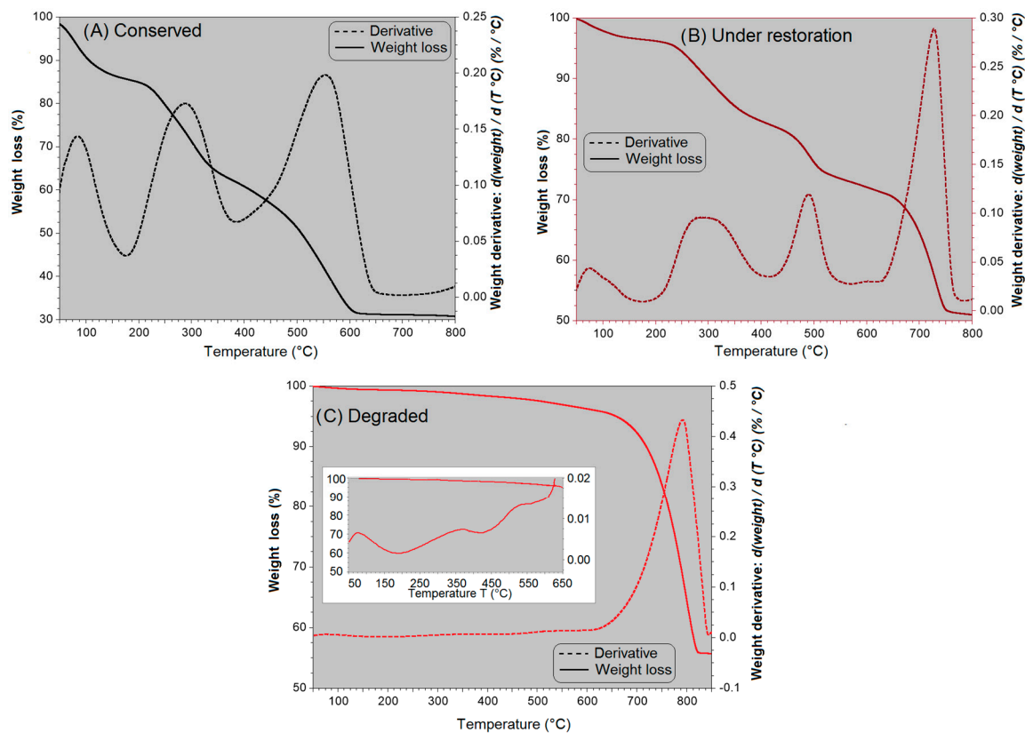
Figure 2. Examples of thermograms at a depth of 0–10 cm, obtained using TGA, showing the weight loss curves and the first derivative of the samples in the different mangrove conditions: (A) conserved; (B) under restoration; and (C) degraded (the zoomed-in image shows the derivative from T_{amb} to 650 °C).
