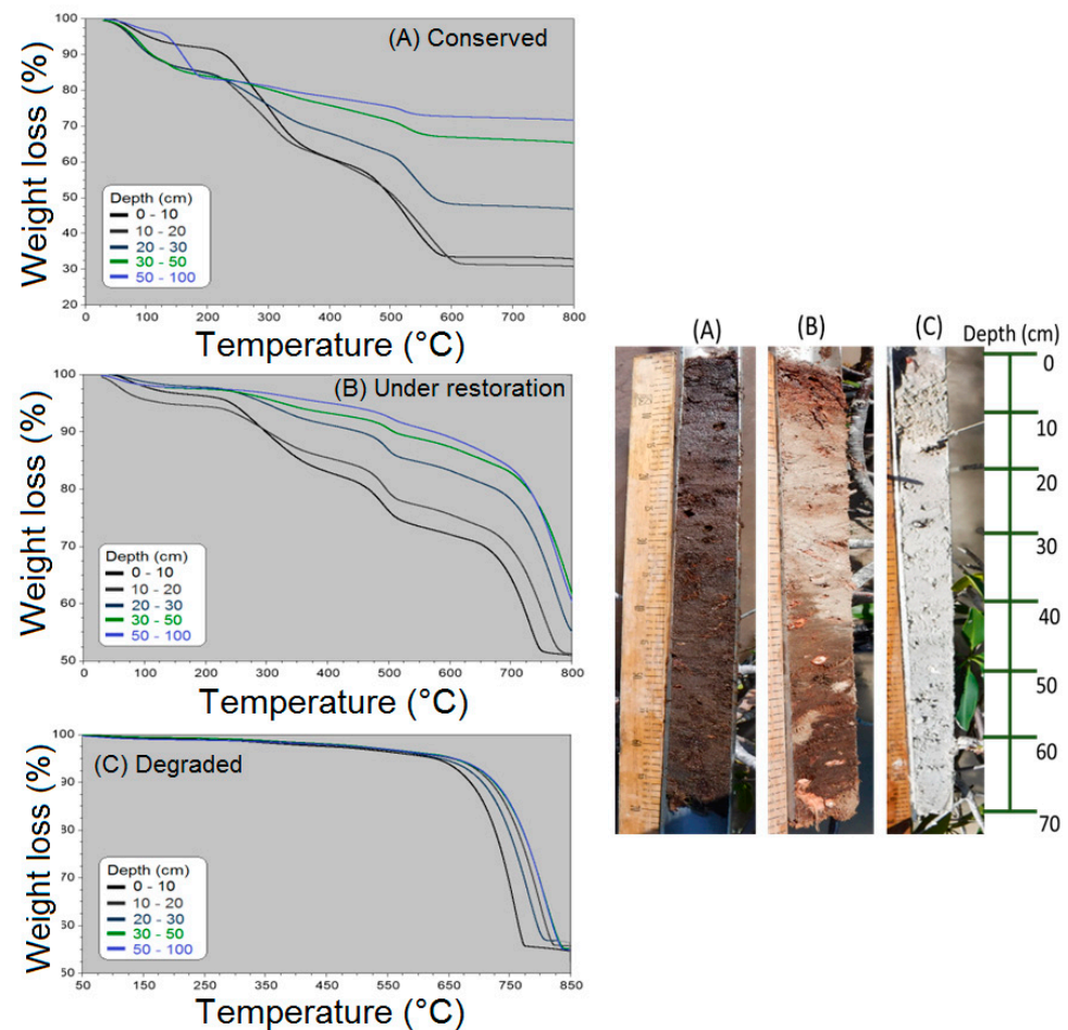
Figure 4. Thermograms of soil samples at different depths by mangrove condition type: (A) conserved; (B) under restoration; and (C) degraded.
