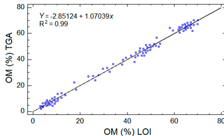
Figure 6. Linear regression of OM content in mangrove soils obtained using TGA ( T_{\text{amb}} —650 °C) and the LOI method (550 °C).
