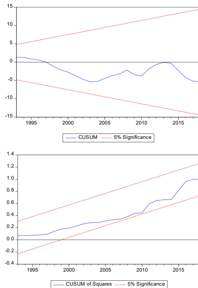
Figure 5. Graph of CUSUM and CUSUMSQR-LIC. Note: The straight lines represent critical bounds at a 5% significance level.
