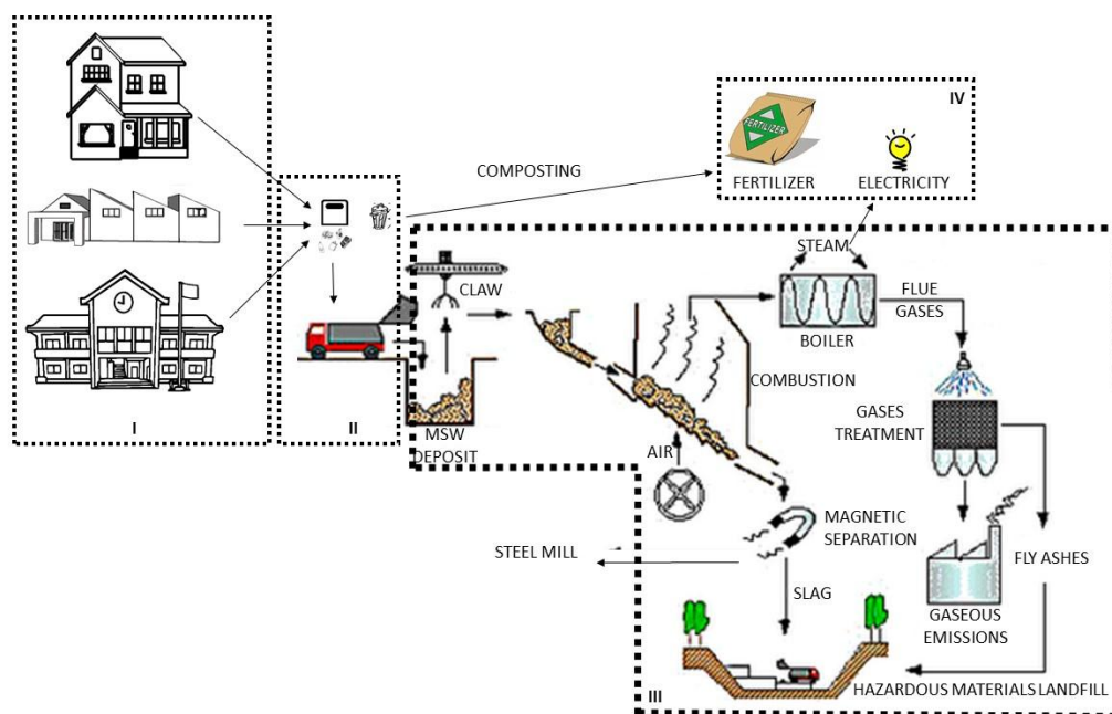
Figure 1. Integrated waste management system operated at the Greater Porto area, ■■■■ representing the chosen boundary for this study.
