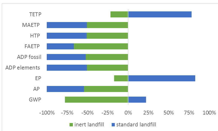
Figure 14. Landfill type effect on the environmental impact categories.
