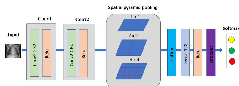
Figure 3. The 2D CNN with 3 \times 3 convolutional layers and SPP architecture.
