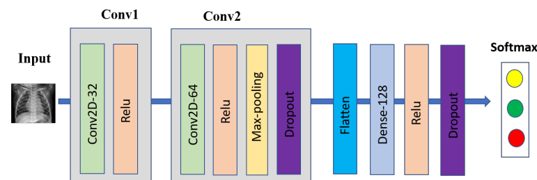
Figure 2. The 2D CNN with 3 \times 3 convolutional layers architecture.
