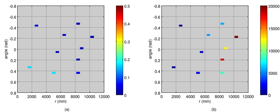
Figure 3. True variances of the observations computed from the data points shown in Figure 2: (a) the angle variance ( \text{deg}^2 ); and (b) the range variance ( \text{mm}^2 ). The values are computed in 2 \text{ deg} \times 500 \text{ mm} bins.
