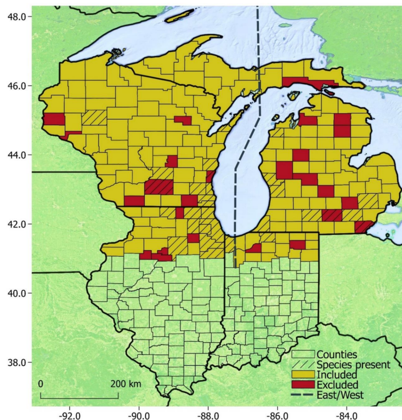
Figure 2. Counties at or above 41^{\circ} N latitude that were included in logistic modeling of presence/absence of silver-haired bats in states surrounding Lake Michigan (yellow). Red counties at or above 41^{\circ} N latitude were excluded, typically because of missing or inadequate climatological data (see text). Cross-hatching indicates counties with at least one record of the silver-haired bat from 2001 to 2016. The boundary for assigning a county to the categories of east versus west of Lake Michigan is also specified. Degrees of latitude and longitude are noted along the left and bottom of the map, respectively.
