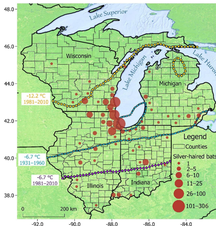
Figure 1. Citizen-based records ( n = 555 ) of the silver-haired bat in four states adjoining Lake Michigan, from 1977 to 2016. The -6.7^\circ\text{C} ( 20^\circ\text{F} ) mean daily minimum isotherm for January 1931–1960 (blue rectangles) [27,34] and for 1981–2010 (purple diamonds) [36] are indicated, as well as the -12.2^\circ\text{C} ( 10^\circ\text{F} ) isotherm for 1981–2010 (yellow squares) [36]. Regions north of a particular isotherm for a given time have cooler average temperatures, whereas those to the south are warmer. The blue oval at the southern end of Lake Michigan indicates that the enclosed area was warmer than -6.7^\circ\text{C} during 1931–1960, whereas the yellow oval in northern Lower Michigan denotes a region that was cooler than -12.2^\circ\text{C} for 1981–2010. Differences in location of the -6.7^\circ\text{C} isotherm for 1931–1960 versus 1981–2010 likely reflect use of additional stations and improved computational techniques [37,38]. Degrees of latitude and longitude are noted along the left and bottom of the map, respectively.
