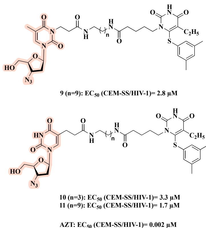
Figure 8. Chemical structures of 9–11 and their anti-HIV-1 profile.
