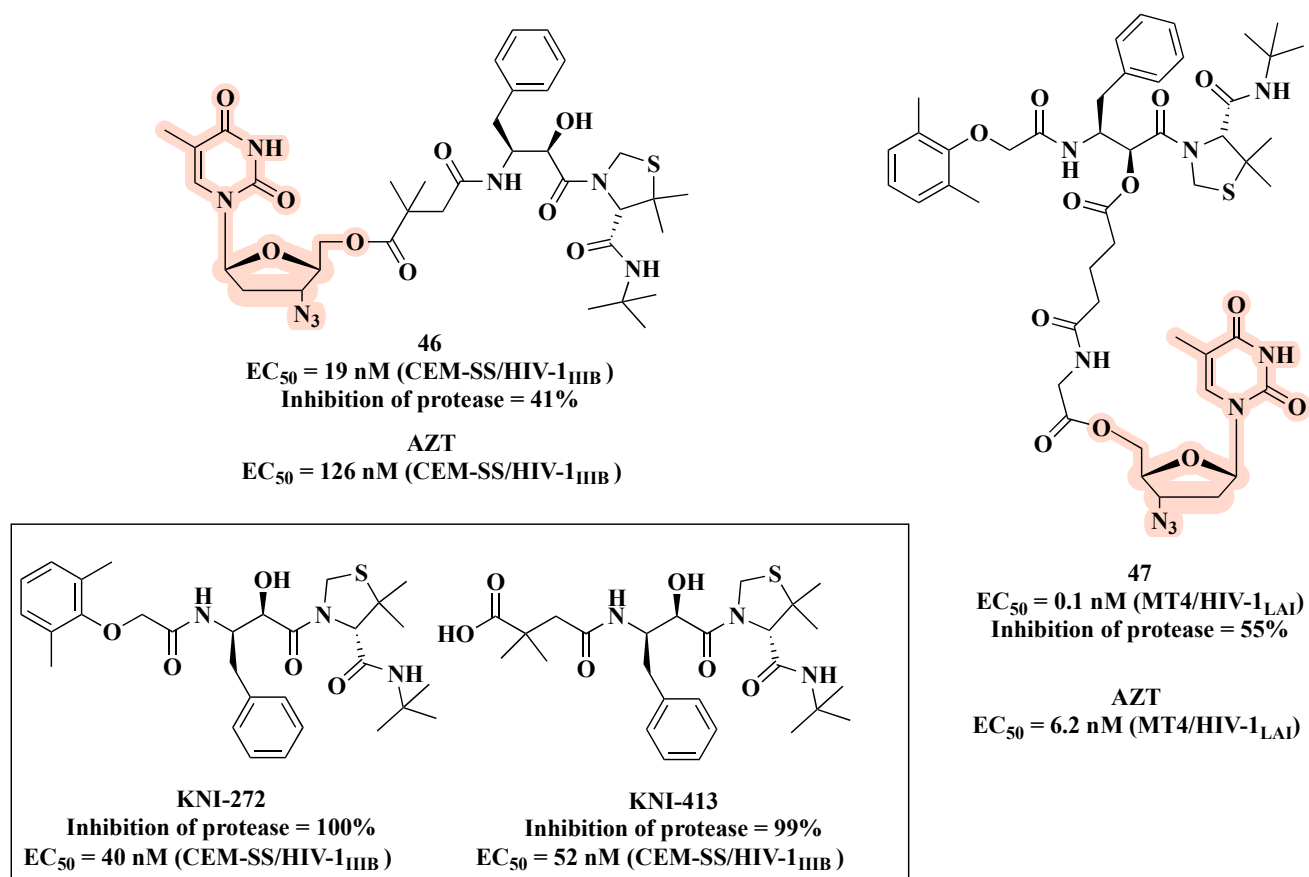
Figure 24. Chemical structures of PIs and co-drugs 46 and 47 along with their anti-HIV-1 profile.
