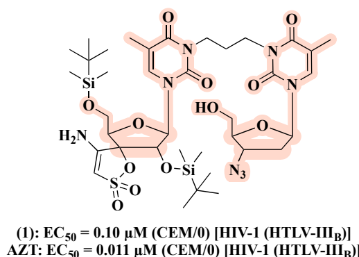
Figure 6. Chemical structure and antiviral activity of 1 compared to the parent compound.
