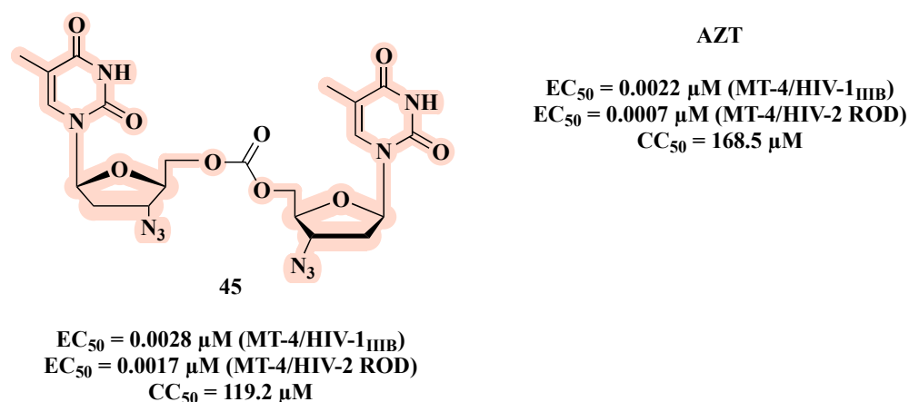
Figure 23. Chemical structure of 45 and its anti-HIV-1 profile.
