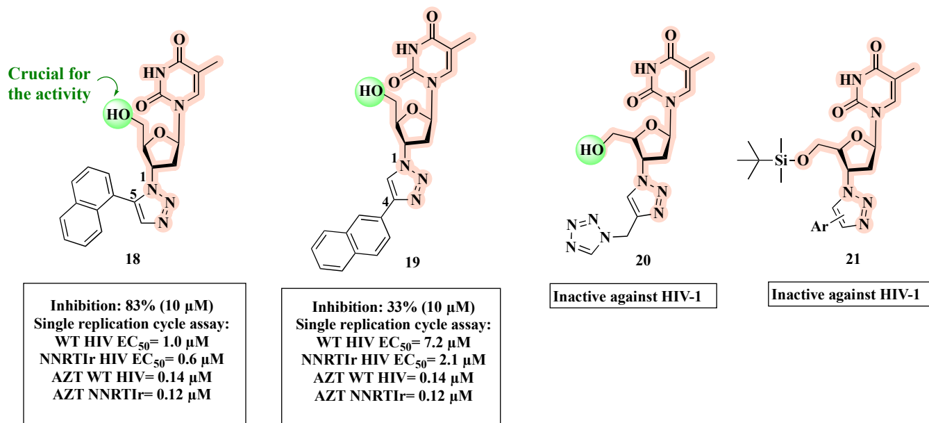
Figure 13. Chemical structures of 18–21 and their anti-HIV profile.
