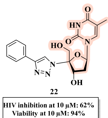
Figure 14. Chemical structure of 22 and its anti-HIV profile.
