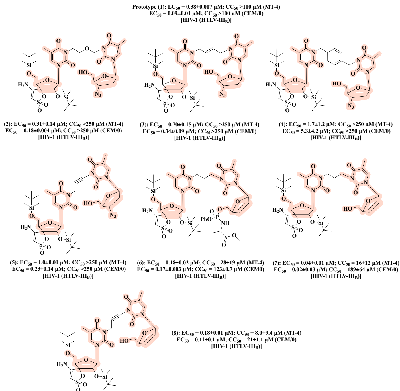
Figure 7. Chemical structures of 2–8 and their anti-HIV-1 profile.
