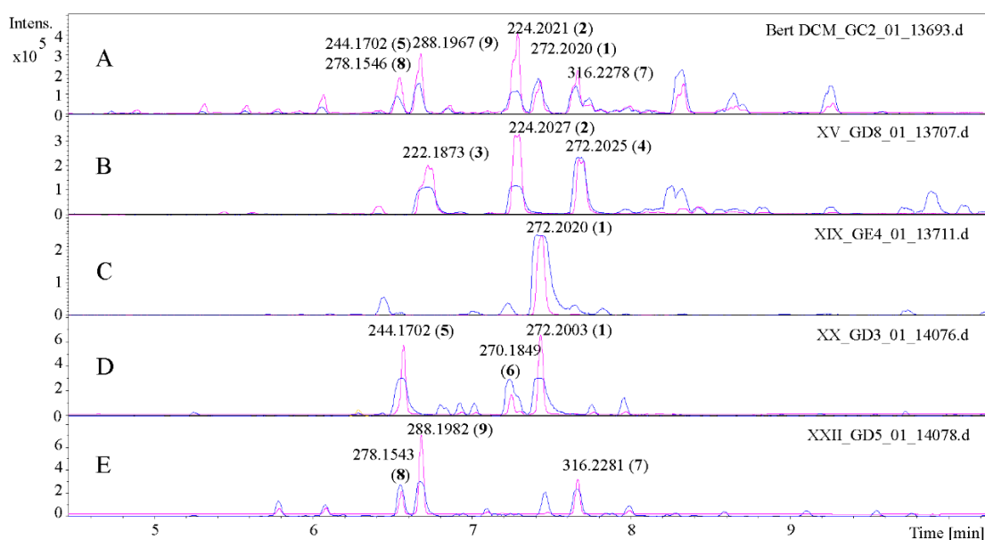
Figure 1. UHPLC/+ESI QqTOF MS-MS chromatograms of the \text{CH}_2\text{Cl}_2 -extract of Anacyclus pyrethrum L. (A) c = 10 \text{ mg/mL} and the selected fractions (B–E) c = 5 \text{ mg/mL} . (B) fraction XV, (C) fraction XIX, (D) fraction XX, and (E) fraction XXII. All peaks are labelled with the measured m/z values and compound numbers. Blue represents base peak chromatogram m/z 100–500, and magenta represents base peak UV-chromatogram at 260 nm.
