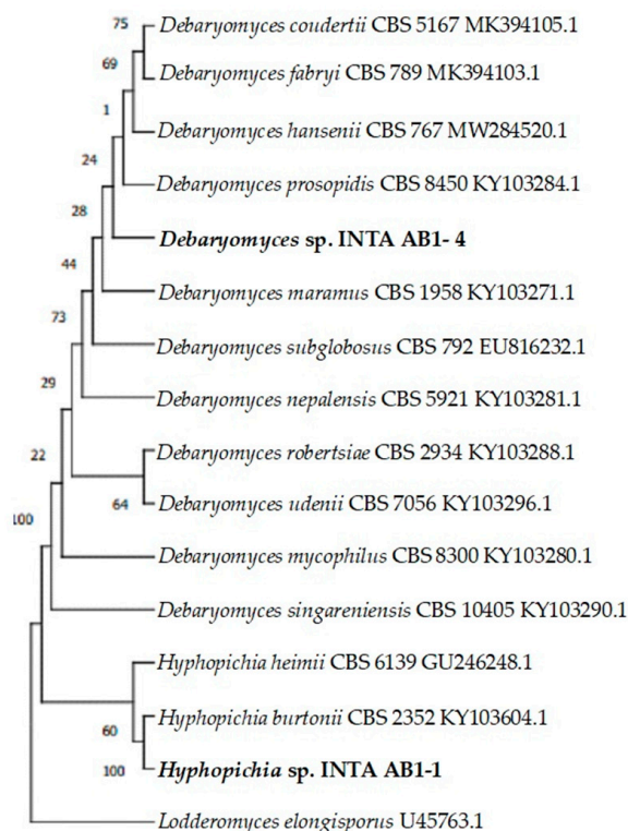
Figure 3. The phylogenetic tree of rRNA gene ITS region sequences illustrates the relationships among the yeast isolates and the type strains of Debaryomyces and Hyphopichia species. The tree was constructed using the neighbor-joining method, and the numbers shown at specific nodes represent consensus bootstrap values derived from 1000 replications.
