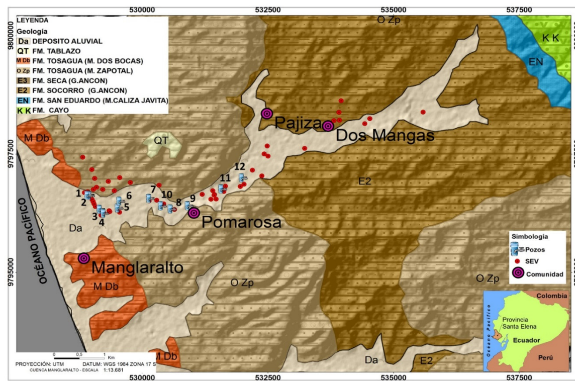
Figure S 1: Map of the geology of the area, in which the location of the SEVs carried out is detailed.
