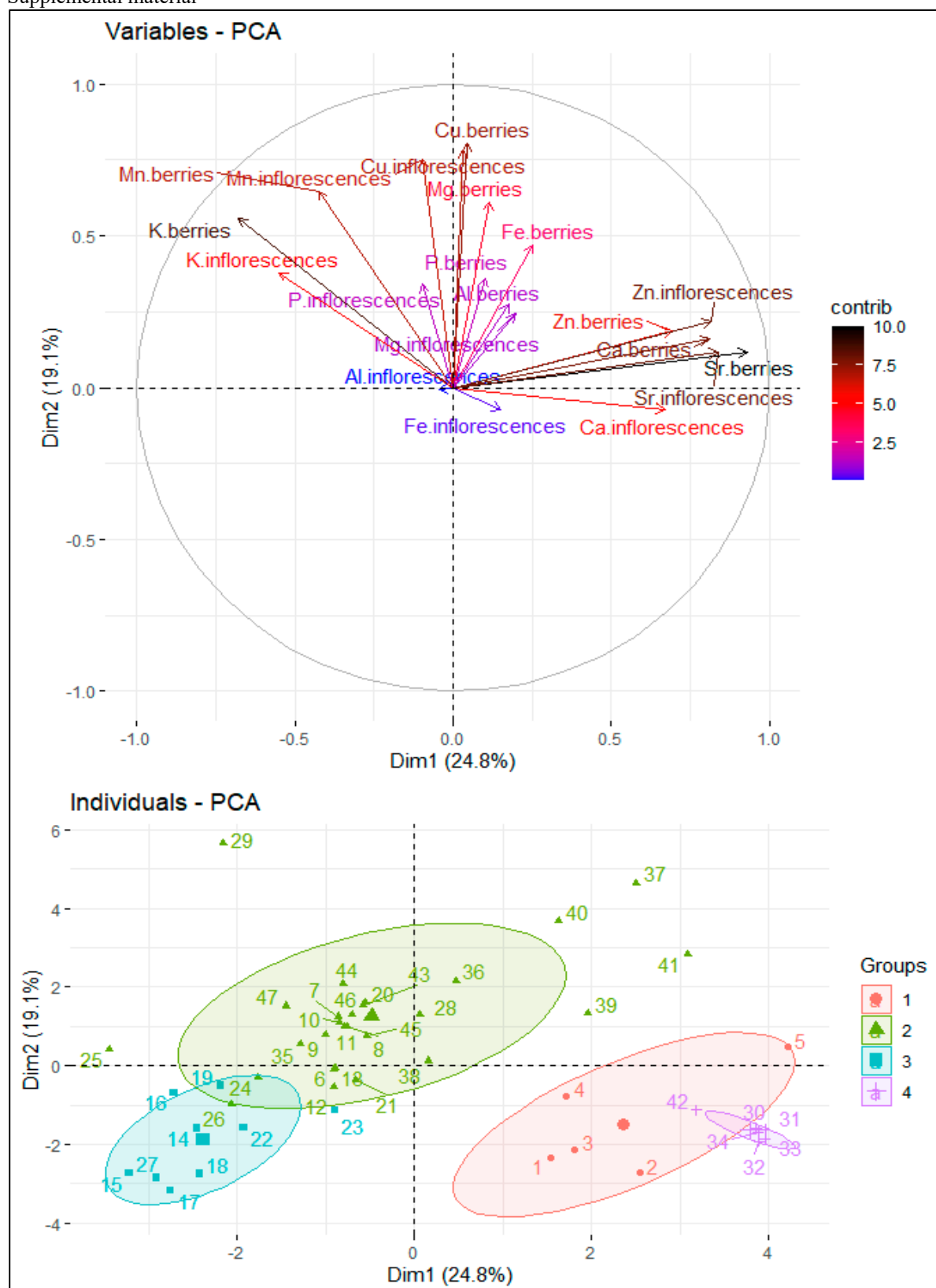
Supplemental material – Figure 1. Variable correlation and scores plot of the first two principal components. Ellipses of clusters represent 0.68 normal probability level.
