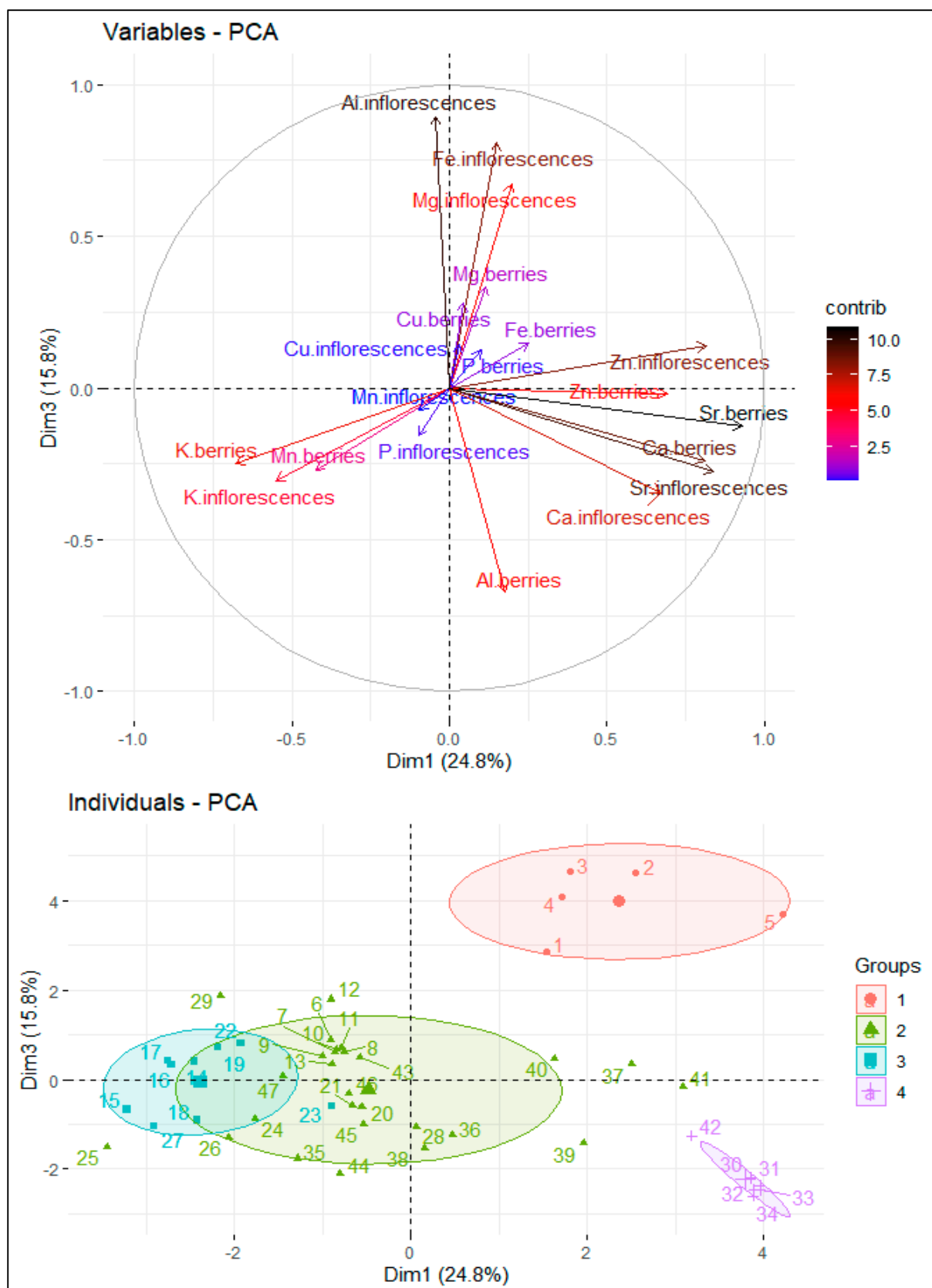
Supplemental material – Figure 2. Variable correlation and scores plot of the first and third principal component. Ellipses of clusters represent 0.68 normal probability level.
