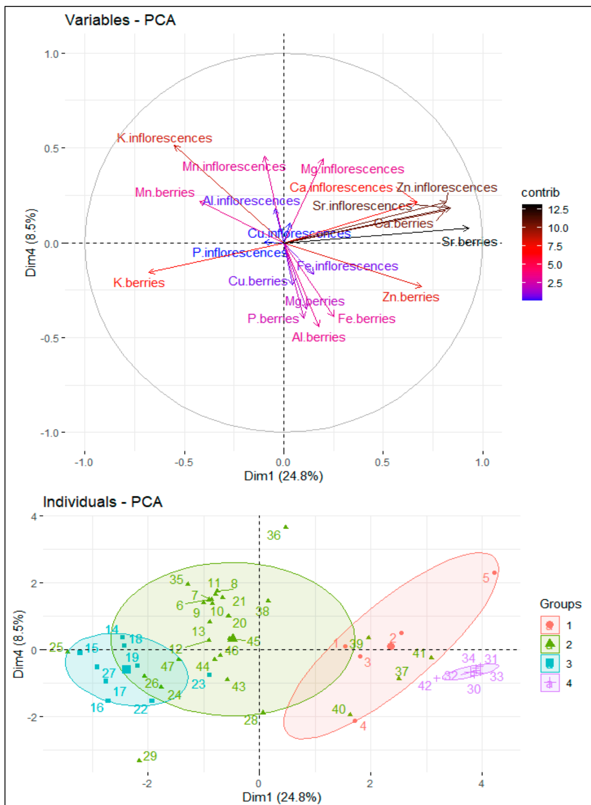
Supplemental material – Figure 3. Variable correlation and scores plot of the first and the fourth principal component. Ellipses of clusters represent 0.68 normal probability level.
