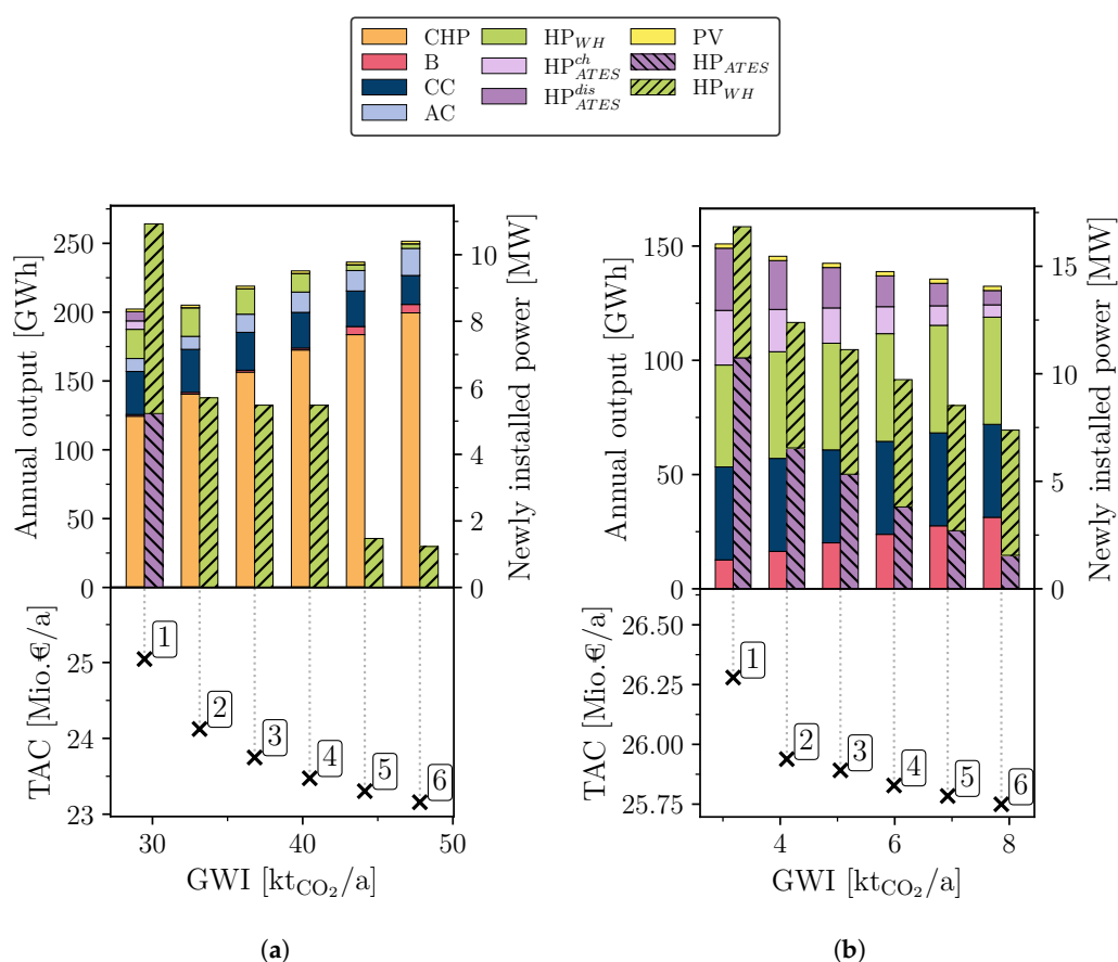
Figure 8. (a) Pareto front of the extended energy system (CS I ). (b) Pareto front of the extended system without CCHP (CS II ). Note that the right y-axis refers to the installed nominal power of the additional components, denoted by striped bars. The left y-axis corresponds to the non-striped bars.
