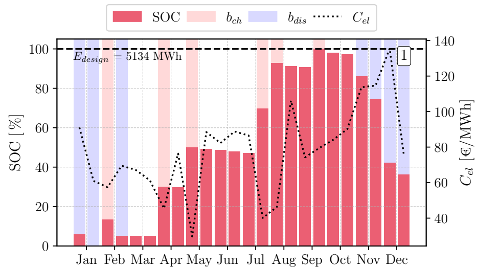
Figure 9. State of charge (SOC) of ATEs for CS I .
