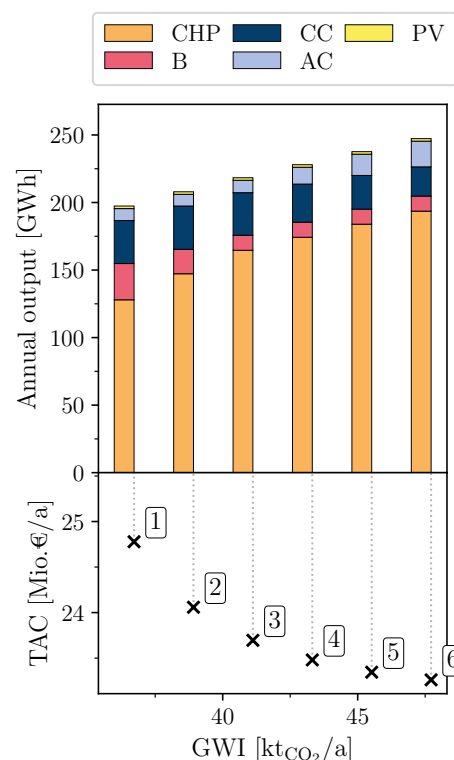
Figure 7. Pareto front of the current energy system (Ref).
