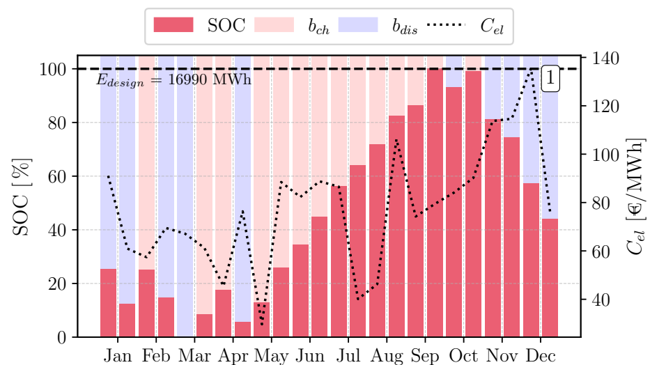
Figure 10. SOC of ATEs for CS II .
