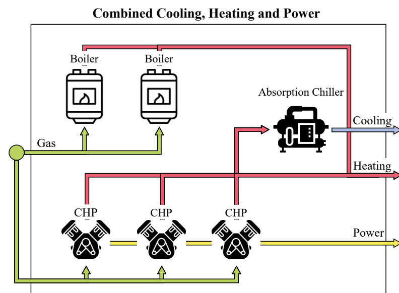
Figure 1. Structure of the combined cooling, heating and power (CCHP) system of Forschungszentrum Jülich (FZJ) consisting of three combined heating and power (CHP) units, two boilers and one absorption chiller. The entire CCHP system has been designed for thermal demand management.
