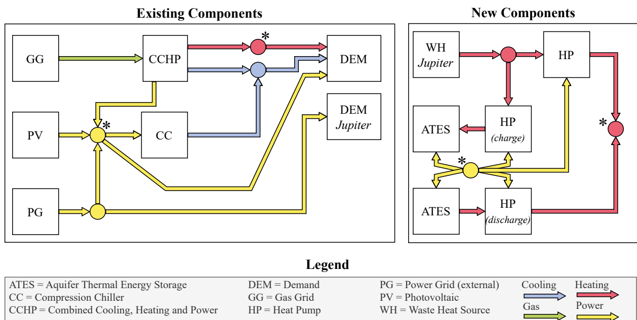
Figure 2. Current and extended energy system of the FZJ. The new components are the waste heat source (WH), heat pumps (HPs) and aquifer thermal energy storage (ATES). Note that the nodes in the same color with * represent the same node for the sake of clarity. Furthermore, the charging and discharging of the ATES cannot occur at the same time.
