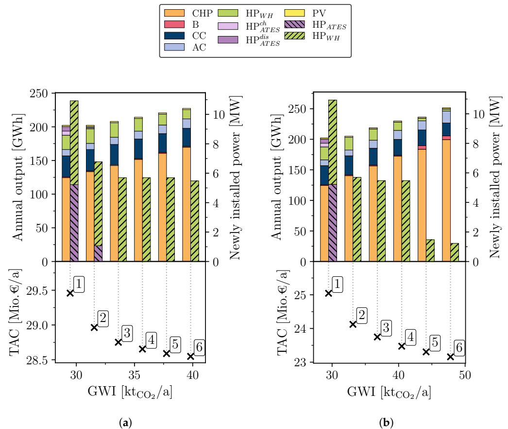
Figure 11. (a) Pareto front for increased energy prices ( S_{II} ). (b) Pareto front for default prices ( CS_I ). Note that the right y-axis refers to the installed nominal power of the additional components, denoted by striped bars. The left y-axis corresponds to the non-striped bars.
