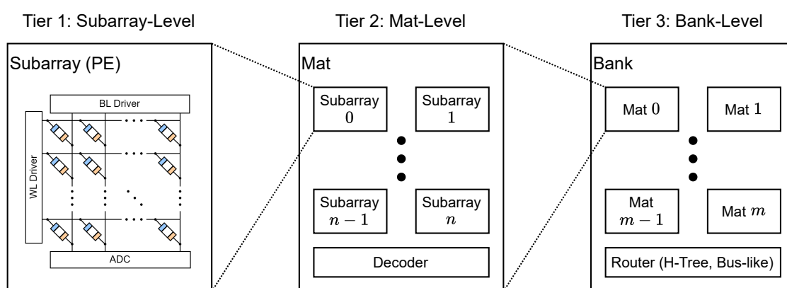
Figure 5. Structure of architectural blocks in NVSim [20]. A PE (pictured here as a crossbar) would be denoted as a 'subarray'. Groups of subarrays form mats, and groups of mats form banks.
