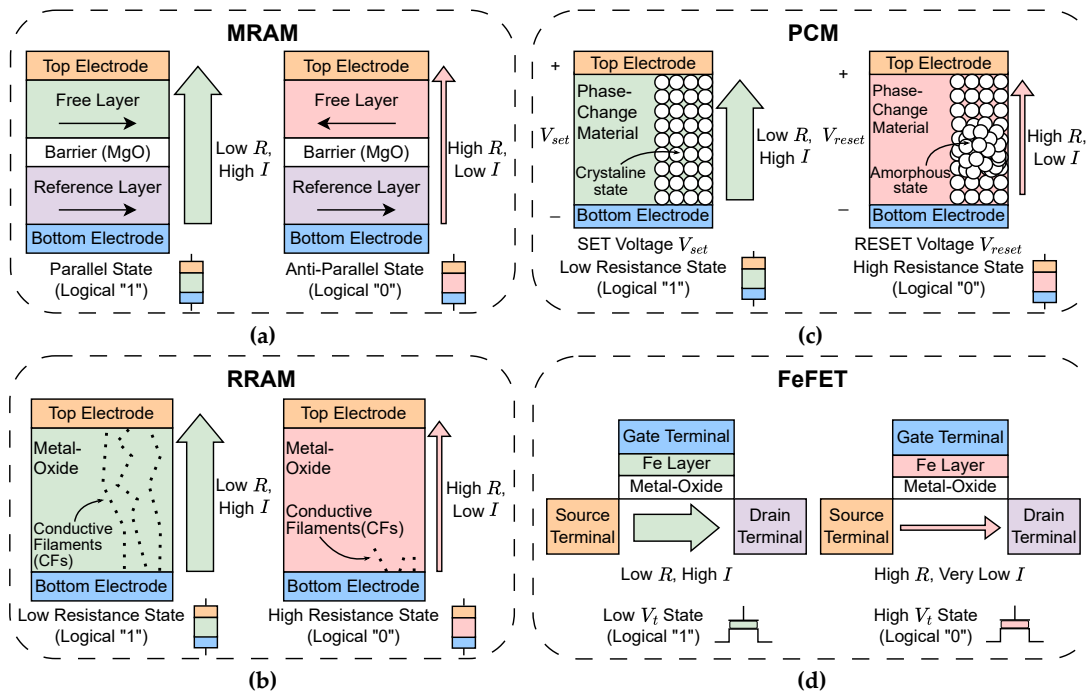
Figure 2. Structure and operation of emerging nonvolatile memory (NVM) devices. Logical “0” is represented whenever the device has high resistance across terminals (light red), and logical “1” is represented when the device has low resistance across terminals (light green). The presented devices are (a) MRAM, (b) RRAM, (c) PCM, and (d) FeFET.
