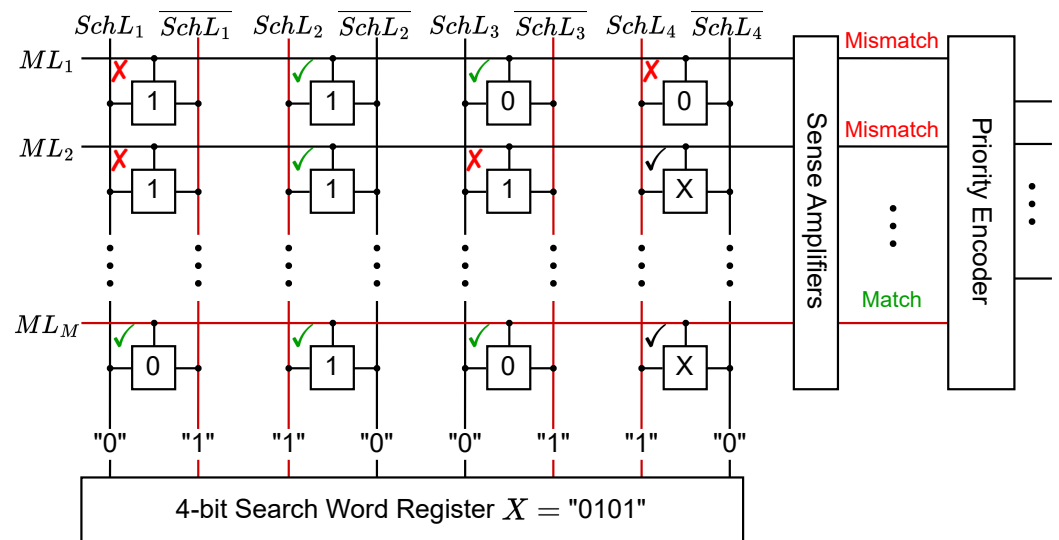
Figure 4. Structure of an M \times 4 TCAM array. The search word X = "0101" is broadcast up the columns via the corresponding search-line SchL_i and its complement \overline{SchL_i} . During evaluation, since there are bits in the top two rows that directly mismatch with the bits in the search word, match-lines ML_1, ML_2 discharge to ground. At ML_M , we have a match case and the line remains charged.
