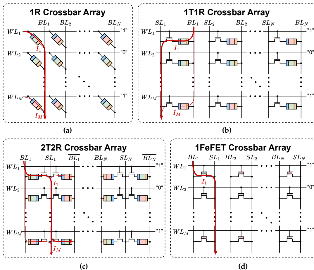
Figure 3. The M \times N array structures of well-known CiM crossbars. Devices in light green are in a LRS while devices in light red are in a HRS. (a) A 1R crossbar array, where the voltage on the WL and the resistance of the device produce a current (dark red) along the BL , accumulating at the bottom to form a sum of products. (b) a 1T1R crossbar array, where a select transistor and an SL are added to provide more control over the selection of cells and to reduce leakage current. (c) a 2T2R crossbar array, where the select transistors share an SL and a complementary bit-line \overline{BL} is added to enable complementary storage of bits. (d) A 1FeFET crossbar array, where the state of the device and the voltage of the WL determine whether or not current flows through it to the SL , representing another sum of products down the SL .
