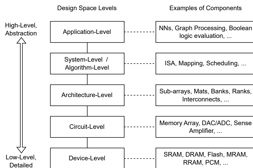
Figure 1. The design space levels for accelerator architectures. Architects have many options to consider for their designs at each of these levels.
