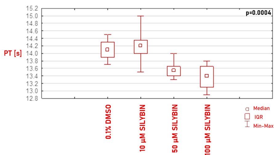
Figure 2. Effects of three different levels of silybin (10 \mu M, 50 \mu M, and 100 \mu M) on prothrombin time (PT) measured in normal human plasma.
