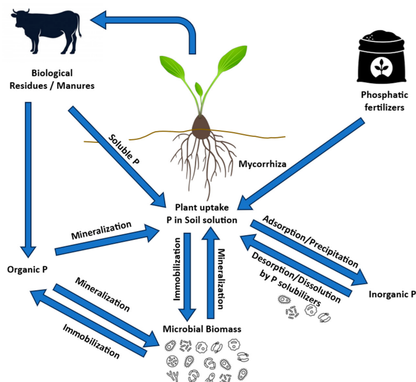
Figure 3. An overview of the phosphorus cycle in nature (Modified from Shrivastava et al., 2018 [147]).
