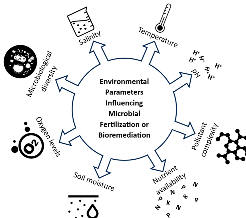
Figure 4. Environmental Parameters Influencing Microbial Fertilization or Bioremediation.
