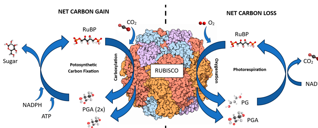
Figure 2. Role of the rubisco molecule in plant primary production and cellular respiration. Modified from Gupta and Kim, 2015 [65].
