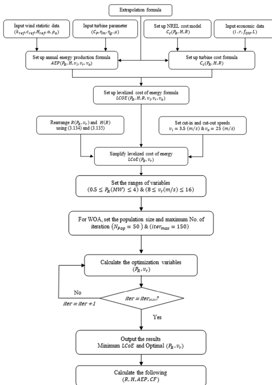
Figure 2. Flow chart of the control software.
