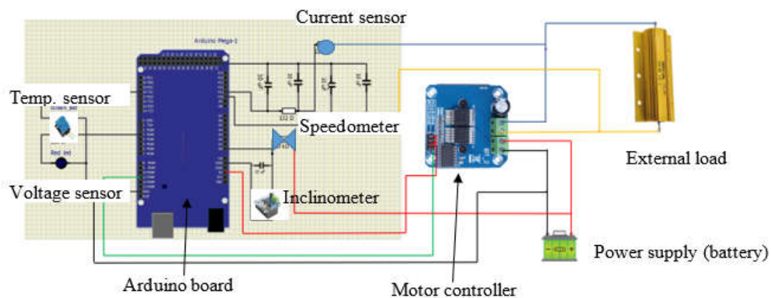
Figure 5. Layout of the experimental simulator.
