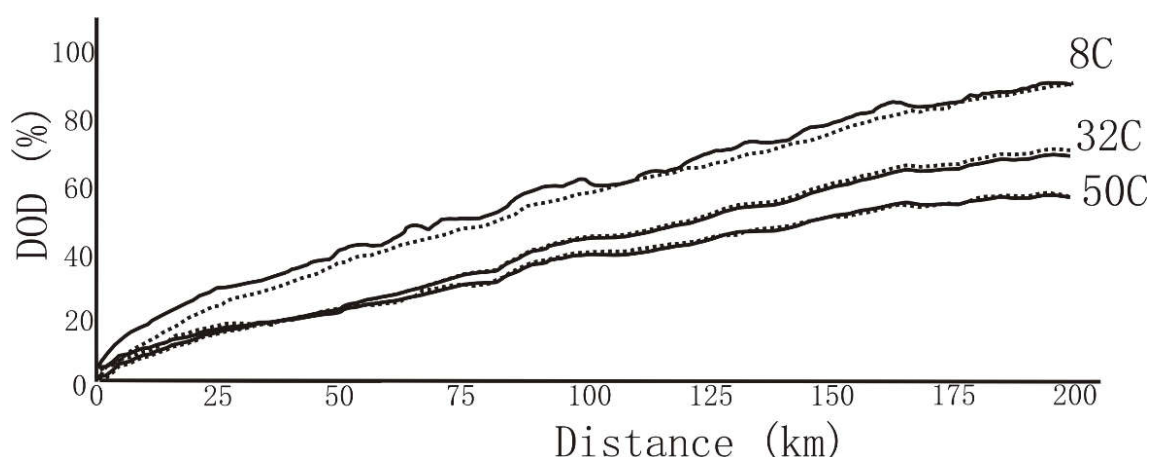
Figure 8. Evolution of DOD of the electric vehicle battery with driving distance.
