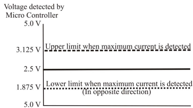
Figure 3. Schematic view of the microcontroller operation.
