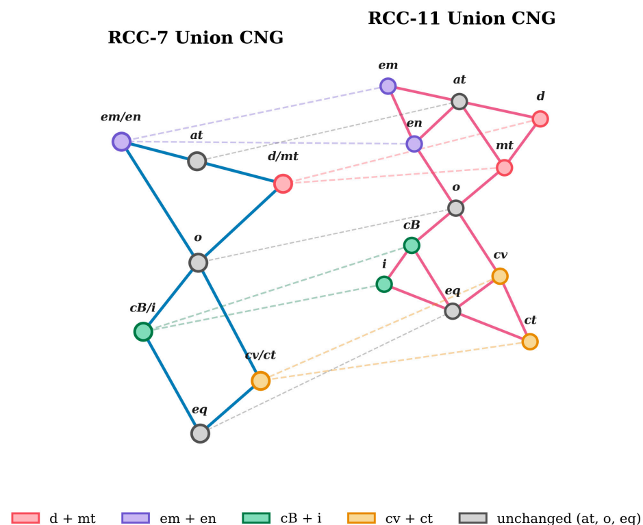
Figure 8. Mapping from region–region relations in RCC-11 [60] to region–region relations in RCC-7 [84]. Connections shown in the graphs are the union of the conceptual neighborhood graphs for homeomorphic deformations [82]. The dashed lines represent crossover connections between the two standalone conceptual neighborhood graphs of RCC-7 and RCC-11.
