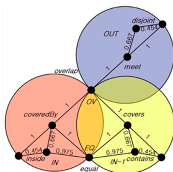
Figure 5. The aggregation of the conceptual neighborhood graphs for RCC-5 [51] and RCC-8 [22] with an eye toward treating the RCC-5 relations as uncertain entities [54]. Each colored circle represents a sphere of somehow similar concepts representing the RCC-5 relation. Conceptually, the expectation is that the uncertain relation is more likely to practically relate to the prototype case without boundary contact. This is merely one example of weighting the conceptual neighborhood graph.
