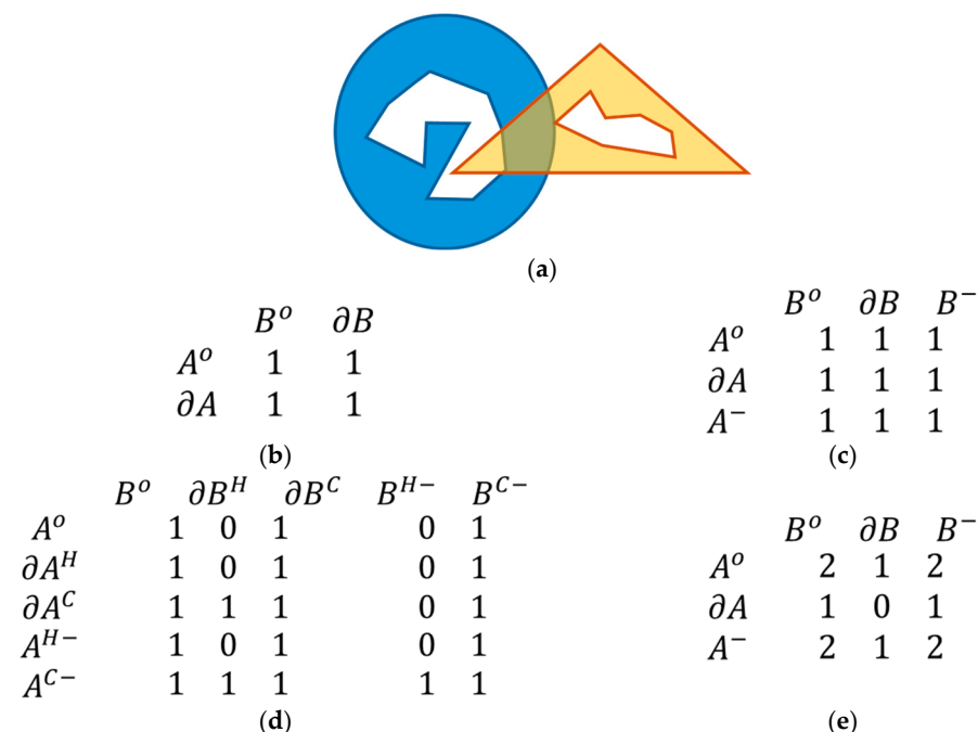
Figure 1. A spatial scene with (a) object A (blue) and object B (orange) with four topological intersection model representations: (b) 4-intersection [44], (c) 9-intersection [21], (d) 9+-intersection [56], and (e) dimensionally extended 9-intersection [57]. Each formalism provides a different set of information about the scene. In (e), the 0 communicates a 0-dimension intersection (i.e., points), whereas in (b–d), 0 would convey no intersection present.
