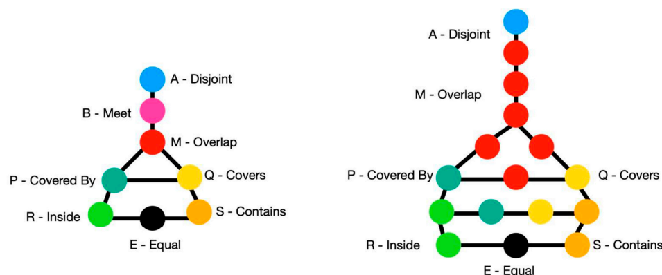
Figure 7. The conceptual neighborhood graph of discretized regions under isotropic scaling ( right ) projected back onto the continuous region–region relations that construct them ( left ) [79], effectively comparing competing models of boundary definition in the digital plane [29–31,43]. The colors become link points in the graphs. Of note is that coveredBy and covers are conceptual neighbors as a function of this aggregation and would not be ordinarily in the continuous set. This is due to the nature of discretization not being able to densely transform itself. The set on the right did not include disjointTouch and therefore did not have the opportunity to model meet conceptually in the continuous setting.
