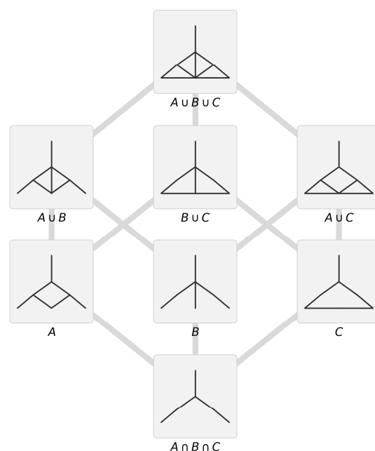
Figure 3. The family of conceptual neighborhood graphs on planar region–region relations, where conceptual neighborhood graph A represents the anisotropic scaling neighborhood, conceptual neighborhood graph B represents the translation/rotation neighborhood, and conceptual neighborhood graph C represents the isotropic scaling neighborhood. Conceptual neighborhood graphs on the higher levels of this lattice represent combinations of deformations allowed from the third level. The lowest level represents the characteristic paths that are common to all deformations in the set [82].
