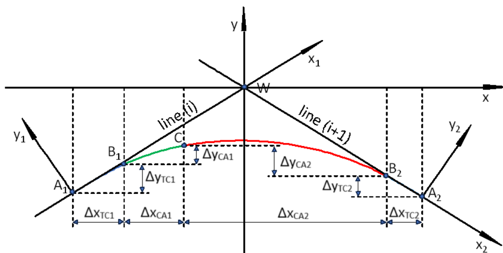
Figure 8. Designed compound curve in the local coordinate system for the case of the geometric system located below the W vertex (the transition curves TC1 and TC2 are marked in blue, the CA1 circular arc in green, and the CA2 arc in red).
