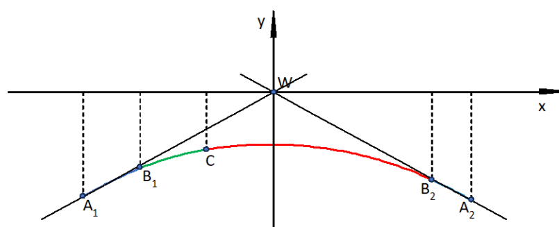
Figure 7. Geometric system of the compound curve in the local coordinate system (the transition curves TC1 and TC2 are marked in blue, the CA1 circular arc in green, and the CA2 arc in red).
