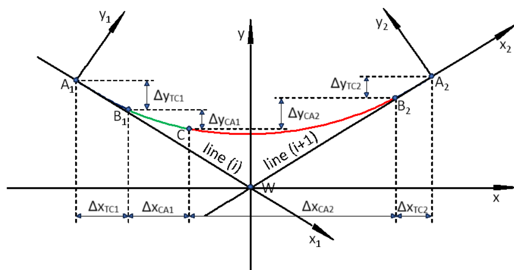
Figure 9. Designed compound curve in the local coordinate system for the case of the geometric system located above the W vertex (designations of transition curves and circular arcs as in Figure 8).
