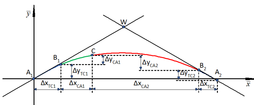
Figure 6. Geometric system of the compound curve against the background of the introduced main directions of the route (the transition curves TC1 and TC2 are marked in blue, the CA1 circular arc in green, and the CA2 arc in red).
