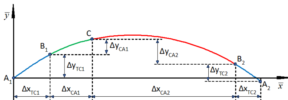
Figure 5. Geometric system for Case I created after correcting the TC2 and CA2 ordinates from Figure 4 (the transition curves TC1 and TC2 are marked in blue, the CA1 circular arc in green, and the CA2 arc in red).
