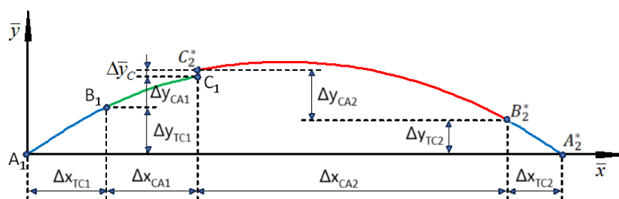
Figure 4. Geometric system created as a result of mirror reflection of TC2 and CA2 with respect to the abscissa \bar{x}_C (the transition curves TC1 and TC2 are marked in blue, the CA1 circular arc in green, and the CA2 arc in red).
