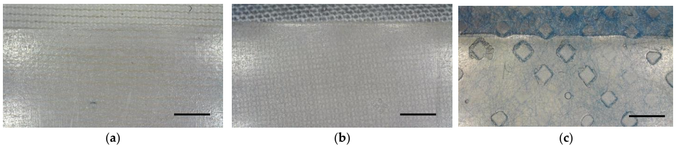
Figure 3. Microscopic images of the back of the printed composites on different textile fabrics: (a) warp-knitted PET; (b) cotton woven fabric; (c) PP nonwoven. Scale bars correspond to 200 \mu\text{m} .
