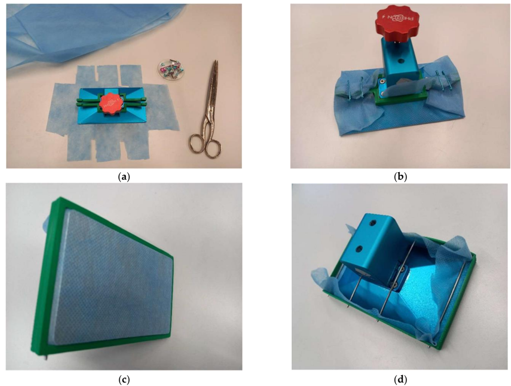
Figure A1. Different approaches for fixing a textile fabric (here, a polypropylene (PP) nonwoven) to the original printing bed of the Anycubic Photon S printer: (a) textile fabric cut before mounting, with green 3D-printed bars for fixation with safety pins; (b) fabric fixed using this bar and safety pins; (c) alternative fixing with a frame, showing the stretched fabric on the printing bed; (d) alternative fixing with a frame, as seen from the back, including metal pins for fixation.
