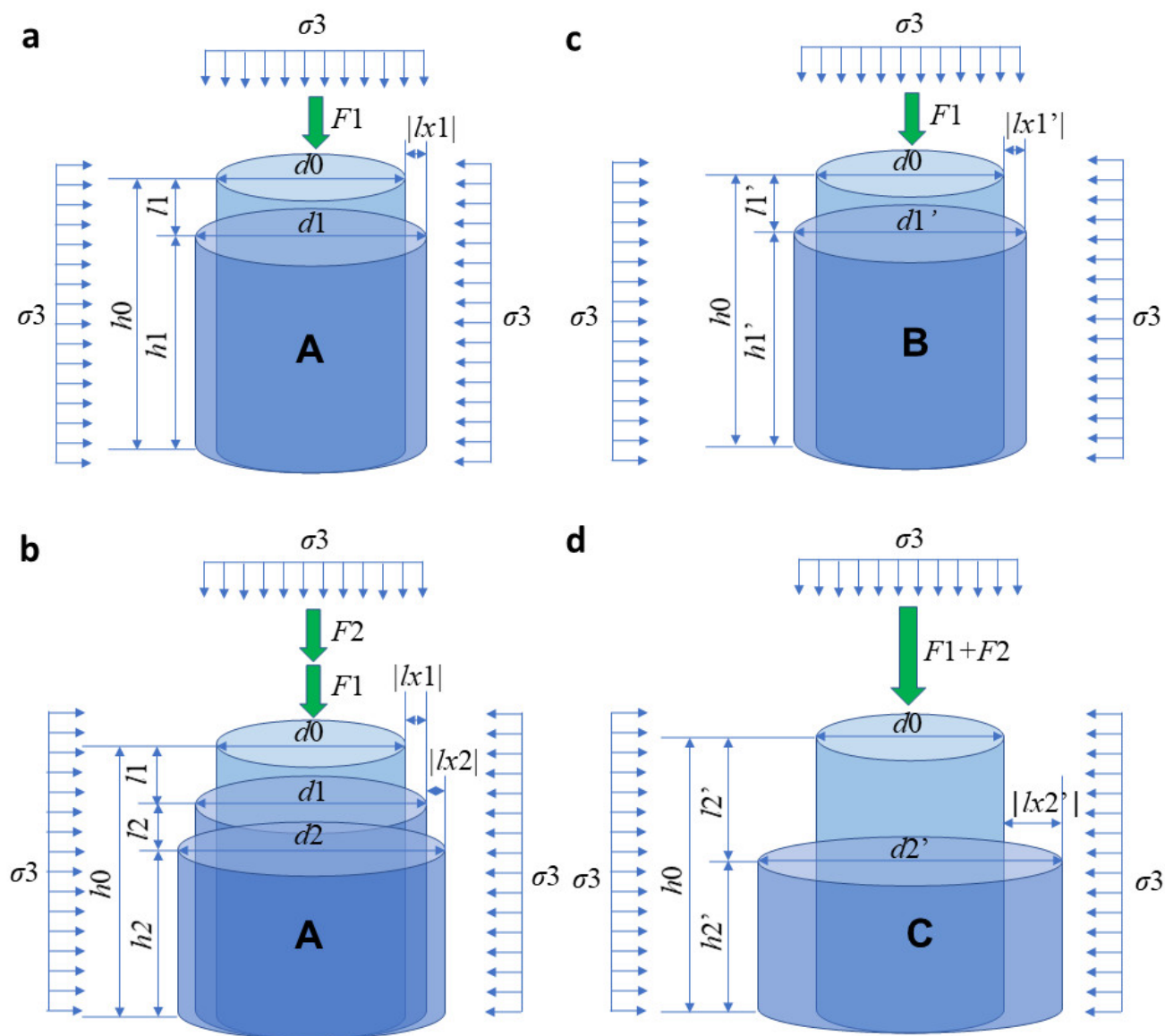
Figure 3. Illustration of SL process on specimen A and RL process on specimen B and C. (a) Specimen A is deformed under F_1 load. (b) Specimen A is continually deformed under another F_2 load after it reached a stable deformation state under F_1 load. (c) Specimen B is deformed under F_1 load. (d) Specimen C is deformed under (F_1 + F_2) load.
