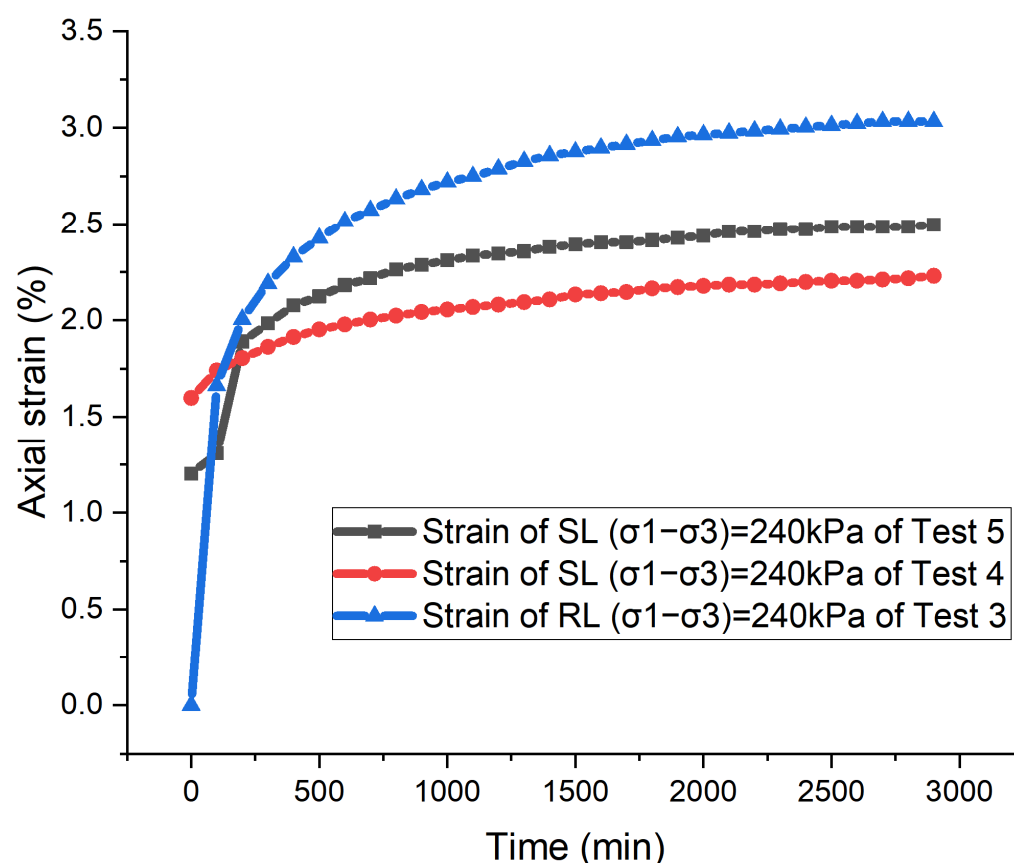
Figure 8. Comparison of axial strain tested in different loading modes when (\sigma_1 - \sigma_3) = 240 kPa (Test 3, 4, 5).
