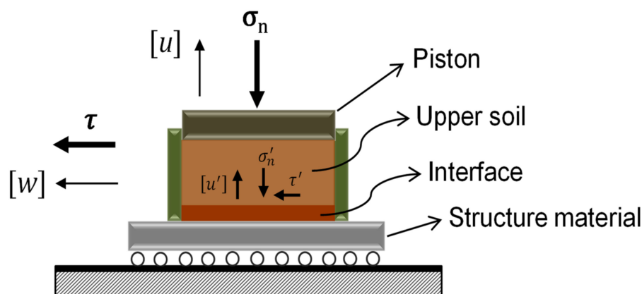
Figure 17. Interface direct shear test box (after Boulon [110]).
