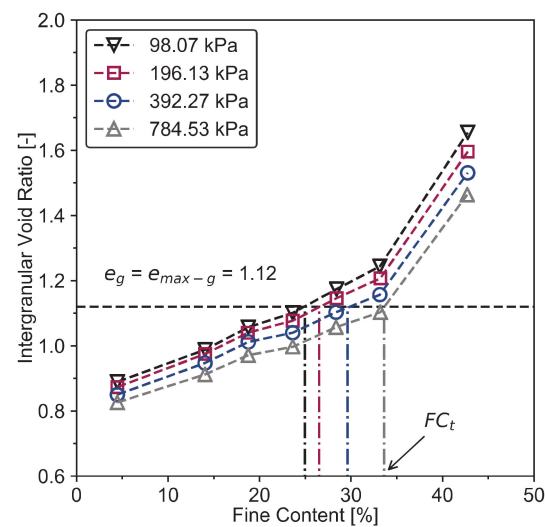
Figure 13. Intergranular void ratio as a function of fines content under different oedometric stress (after Monkul and Ozden [83]).
