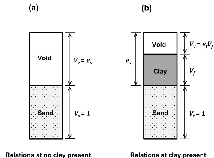
Figure 16. Phase diagram for the transitional fines content calculation: (a) relations at no clay present and (b) relations at clay present (after Hazirbaba [94]).
