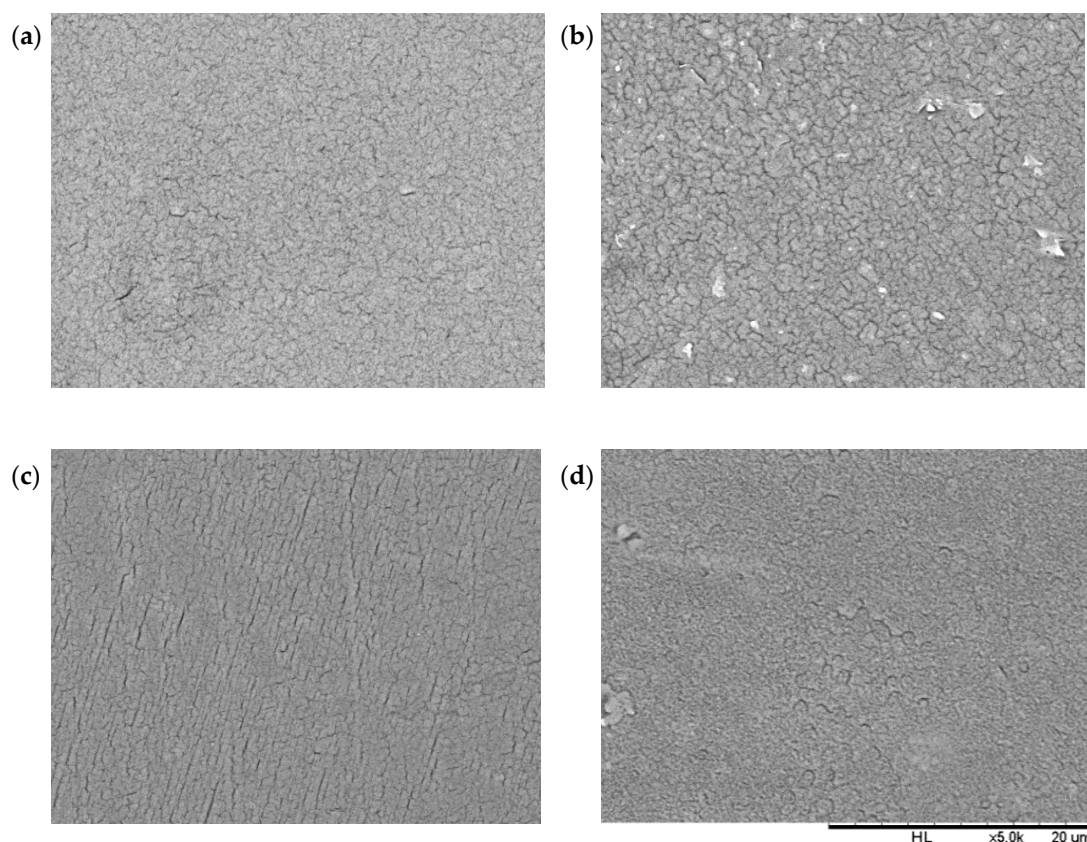
Figure 1. SEM evaluation of PHB/fibrillated cellulose paper coatings in top view at comparable magnification 5000 \times , including (a) pure PHB, (b) MFC-5 coating, (c) NFC-5 coating, and (d) mMFC-5 coating (same scale-bar applies to all figures).
