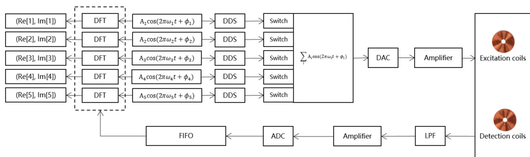
Figure 3. Digital eddy current signal processing.
