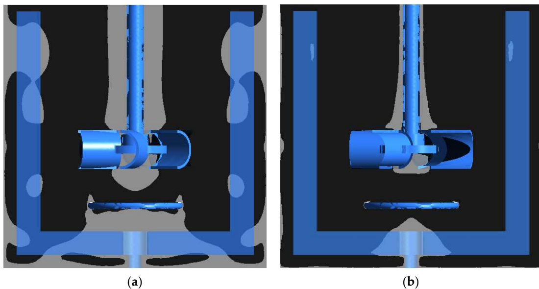
Figure 2. Fluid velocity distribution obtained by the large-scale coaxial mixer containing a 0.5 wt% CMC solution: (a) central impeller speed = 235 rpm, anchor impeller speed = 10 rpm, and aeration rate = 0.12 vvm, and (b) central impeller speed = 330 rpm, anchor impeller speed = 10 rpm, and aeration rate = 0.12 vvm.
