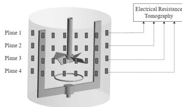
Figure 1. Experimental setup.
