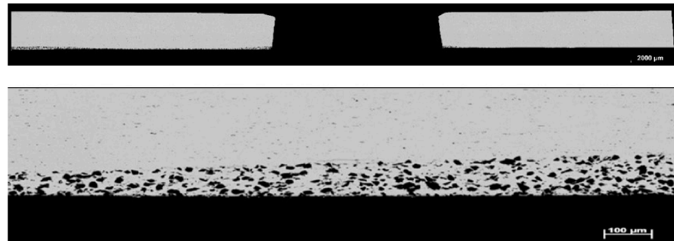
Figure 7. Microscopic analysis general observations and CS bond line quality.
