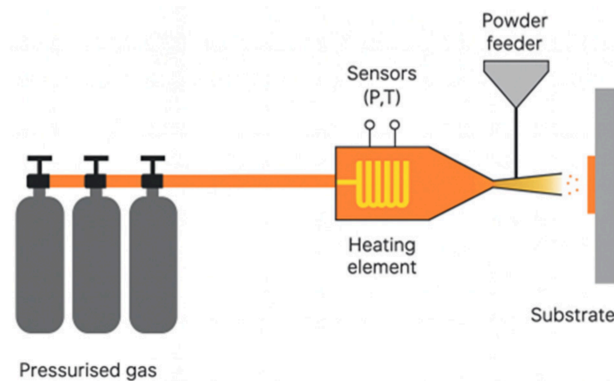
Figure 1. Illustration of the cold spray deposition process.
