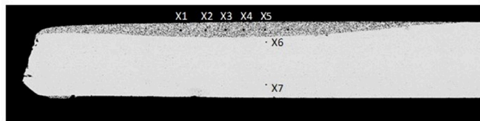
Figure 5. Locations of microhardness testing on cross-section 3-1 of bracket #3 (locations X1–X5 in coating side, locations X6–X7 in substrate).
