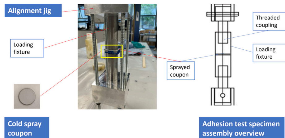
Figure 4. CS repair test specimen preparation according to ASTM C633.
