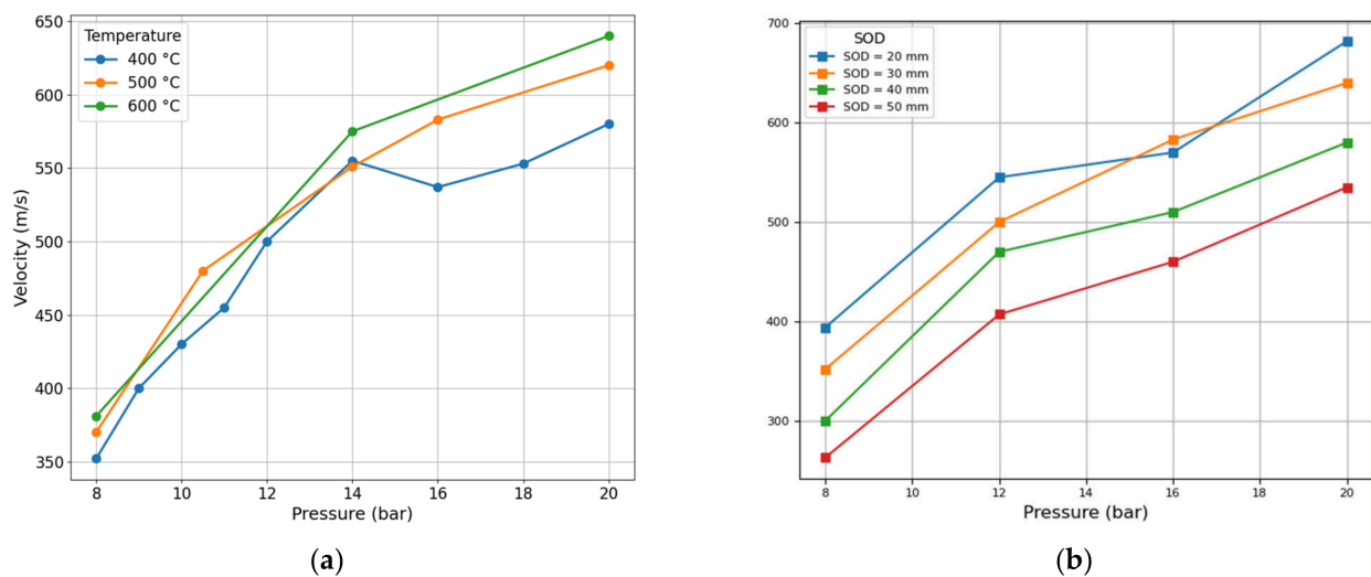
Figure 3. Particle velocity response of the system for (a) varying pressure and temperature (SOD at 30 mm) and (b) varying SOD, pressure and constant temperature (400 °C).
