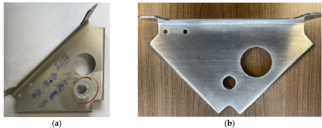
Figure 2. Images of the aircraft MLG bracket (AA 6013-T6), which has been employed as a use case: (a) bracket damaged by pitting corrosion around the indicated hole; (b) bracket repaired with CS.
