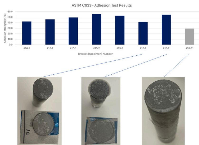
Figure 6. Results of bond strength test according to ASTM C633. Coupon #10-3* failed at a lower load due to poor application of the adhesive epoxy.
