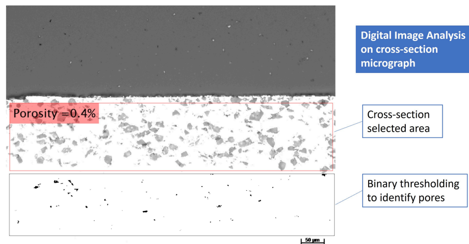
Figure 8. Porosity rating results according to ASTM E3/ASTM E2109.
