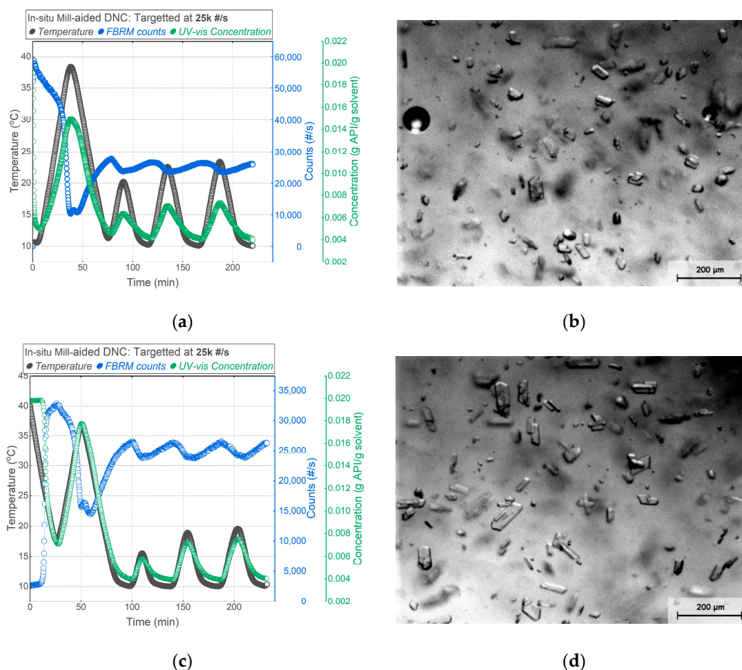
Figure 4. (a) Temperature —, FBRM counts —, and concentration — profiles for experiment IMDNC-1, and (b) PVM image of final product crystals of IMDNC-1. (c) Temperature —, FBRM counts —, and concentration — profiles for experiment IMDNC-2, and (d) PVM image of final product crystals for IMDNC-2.
