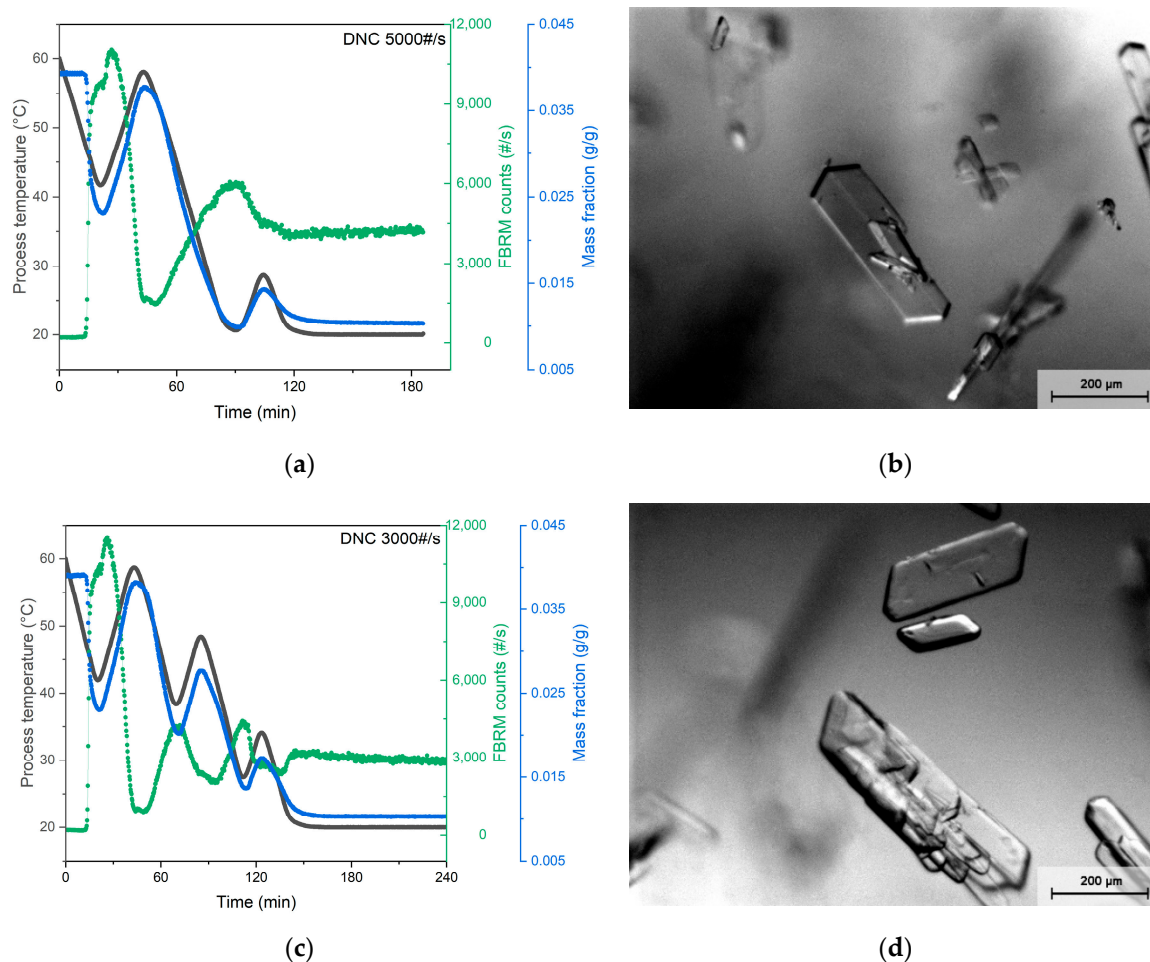
Figure 3. (a) Temperature —, FBRM counts —, and concentration — profiles for experiment DNC-1 with target counts of 5000 #/s and (b) PVM image of final product crystals of DNC-1. (c) Temperature —, FBRM counts —, and concentration — profiles for experiment DNC-2 with target counts of 3000 #/s, and (d) PVM image of final product crystals for DNC-2.
