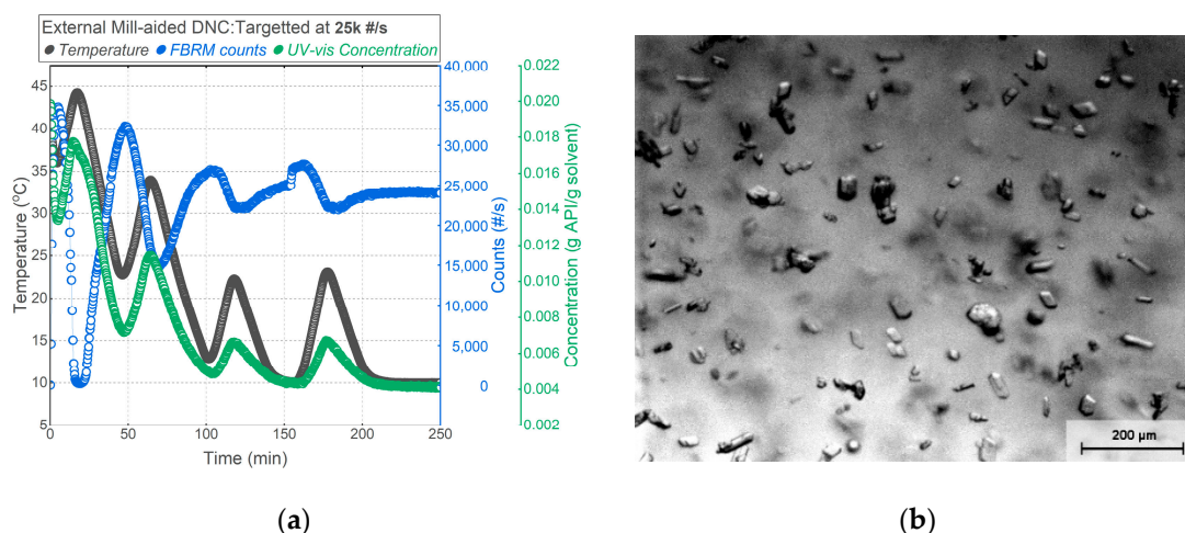
Figure 5. (a) Temperature —, FBRM counts —, and concentration — profiles for experiment EMDNC-1 with final target counts of 25,000 #/s, and (b) PVM image of final product crystals of EMDNC.
