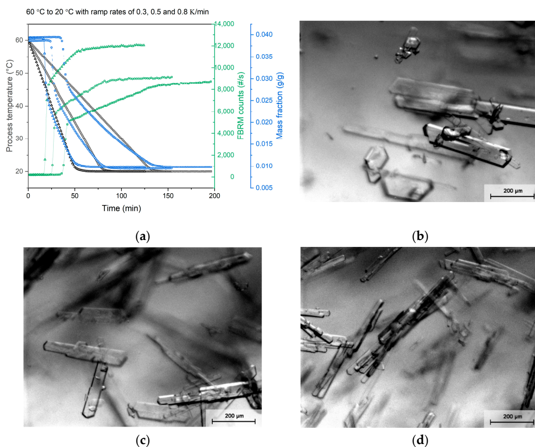
Figure 2. (a) Temperature —, FBRM counts —, and concentration — profiles for experiments LC-1 to LC-3 at different cooling rates of □ 0.3 K/min, ○ 0.5 K/min, and △ 0.8 K/min; PVM image of final product crystals of (b) LC-1, (c) LC-2, and (d) LC-3.
