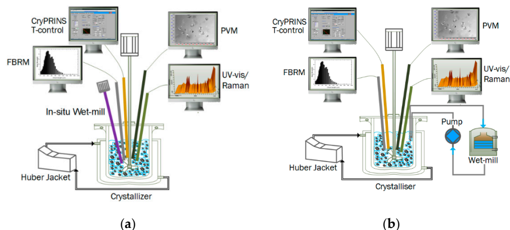
Figure 1. Schematic of the experimental set-up for (a) the in situ wet-mill crystallization unit and (b) external wet-mill crystallization with recirculation.
