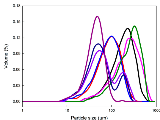
Figure 6. Particle size distribution for experiments LC-1—, LC-2—, LC3—, DNC-1—, DNC-2—, IMDNC-1—, IMDNC-2—, EMDNC—.
