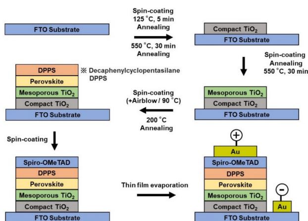
Figure 1. Schematics the processes for the PSC architectures.
