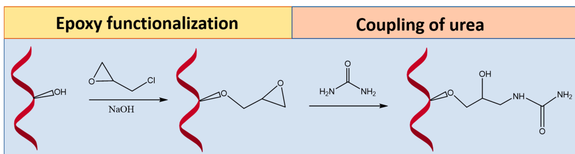
Figure 2. The synthesis pathway of the functionalization of maltodextrin with urea.
