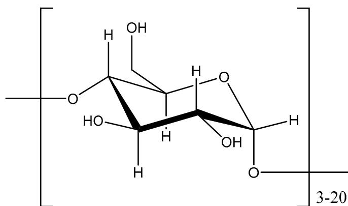
Figure 1. Maltodextrin structure.
