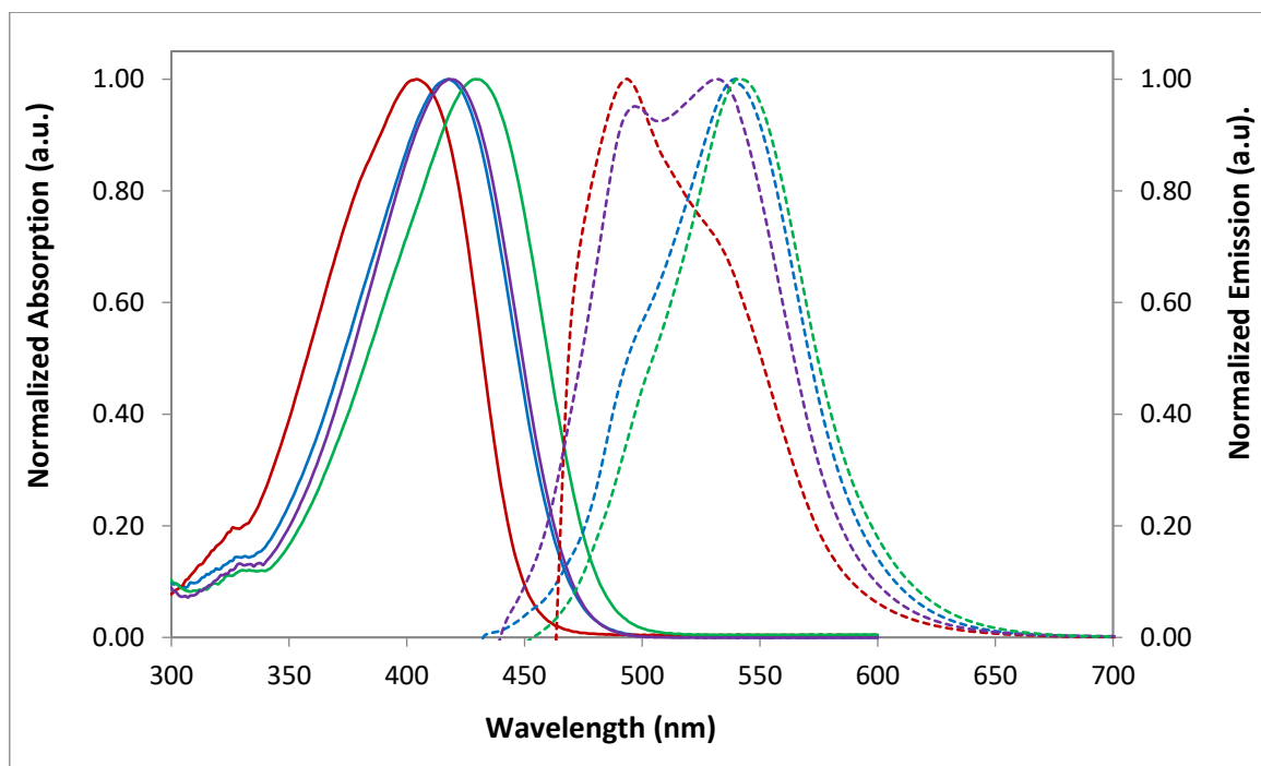
Figure 3. Normalized absorption and emission spectra of chalcone 2c in acetonitrile, diethyl ether, chloroform and dimethyl sulfoxide ( \lambda_{\text{exc}} = 418 nm, 404 nm, 418 nm and 429 nm, respectively; absorption, full line; emission, dotted line).
