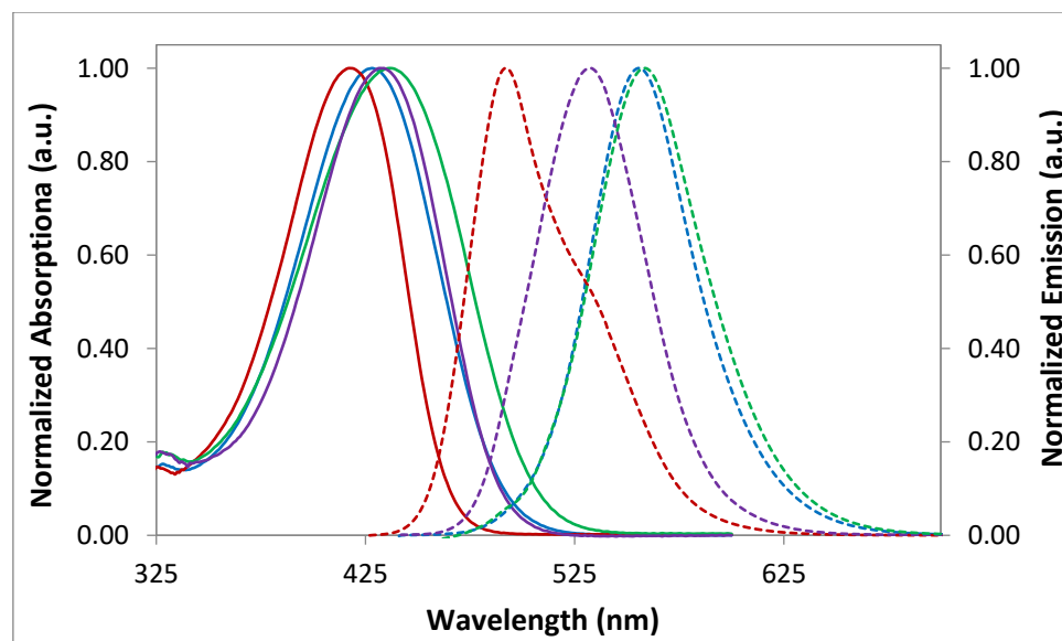
Figure 4. Normalized absorption and emission spectra of chalcone 4c in acetonitrile, diethyl ether, chloroform and dimethyl sulfoxide ( \lambda_{\text{exc}} = 428 nm, 417 nm, 432 nm and 437 nm, respectively; absorption, full line; emission, dotted line).
