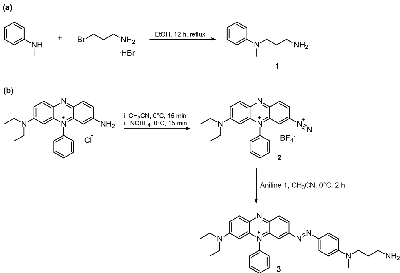
Scheme 1. Synthesis of BHQ3-amine 3 : (a) asymmetrical tertiary aniline 1 ; (b) BHQ-3 amine 3 .
