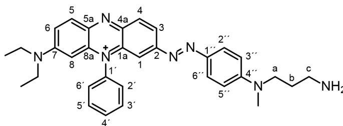
Figure 3. Structure of BHQ-3 amine 3 .
