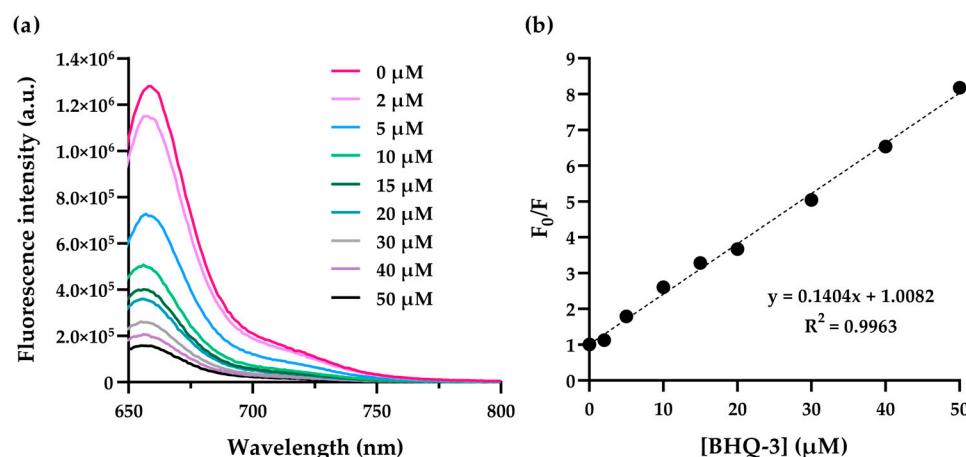
Figure 5. (a) Fluorescence spectra of a 5 \mu\text{M} Cy5 solution at varying concentrations of BHQ-3 amine (3). (b) Stern–Volmer plots illustrating the variation of F_0/F as a function of BHQ-3 concentration.
