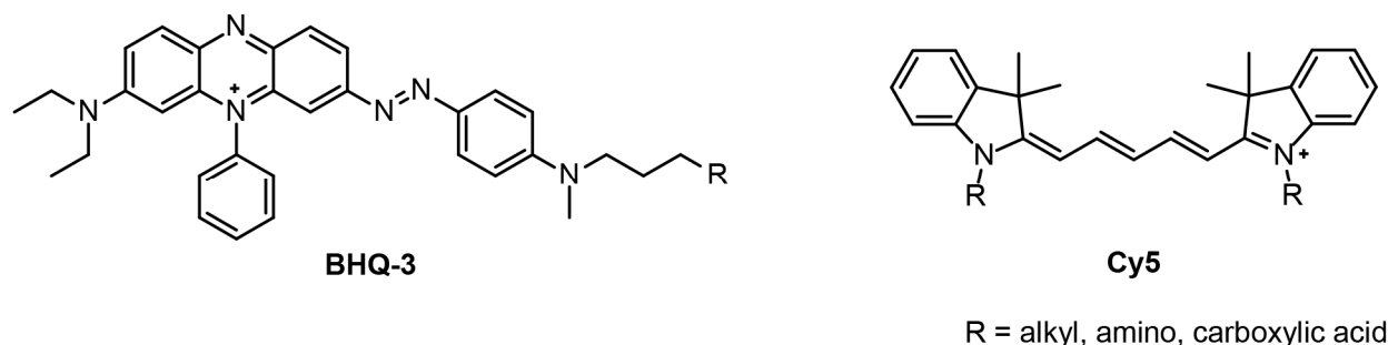
Figure 1. General structures of BHQ-3 and Cy5 derivatives.
