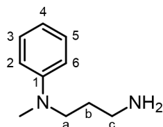
Figure 2. Structure of tertiary aniline 1 .
