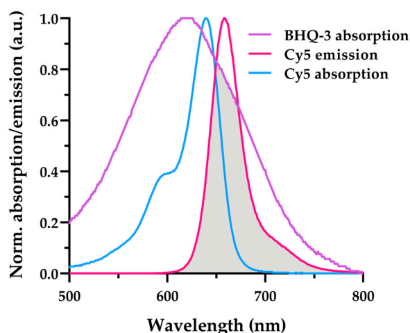
Figure 4. Normalized absorption and emission spectra of BHQ-3 amine ( 3 ) and Cy5 (5 \mu M) in PBS (pH 7.4). The shaded area highlights the spectral overlap between the emission spectrum of Cy5 and the absorption spectrum of BHQ-3 amine.
